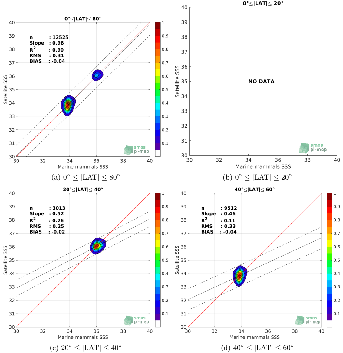
Figure 9: Contour maps of the concentration of SMAP SSS L3 v4 - Monthly (RSS) SSS (y-axis) versus Marine mammals SSS (x-axis) at match-up pairs for different latitude bands. For each plot, the red line shows x=y . The black thin and dashed lines indicate a linear fit through the data cloud and the \pm 95\% confidence levels, respectively. The number match-up pairs n , the slope and R^2 coefficient of the linear fit, the root mean square (RMS) and the mean bias between satellite and in situ data are indicated for each latitude band in each plots.
