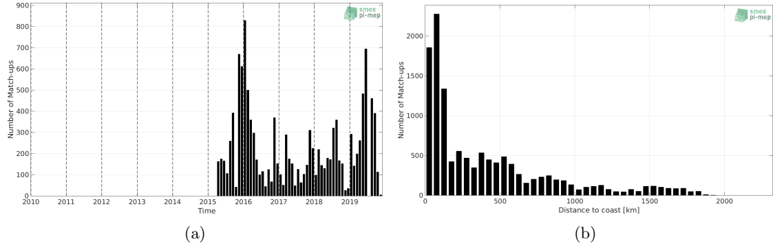
Figure 1: Number of match-ups between Marine mammals and SMAP SSS L3 v4 - Monthly (RSS) SSS as a function of time (a) and as function of the distance to coast (b) over the Indian Ocean Pi-MEP region and for the full satellite product period.
