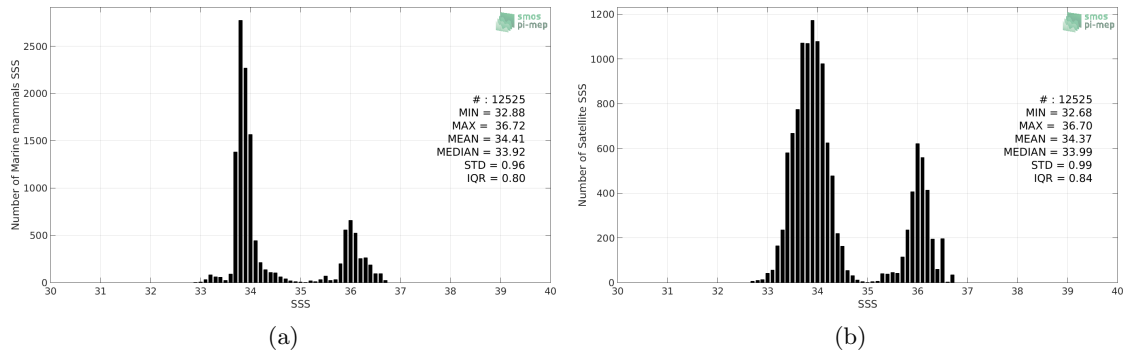
Figure 2: Histograms of SSS from Marine mammals (a) and SMAP SSS L3 v4 - Monthly (RSS) (b) considering all match-up pairs per bins of 0.1 over the Indian Ocean Pi-MEP region and for the full satellite product period.
