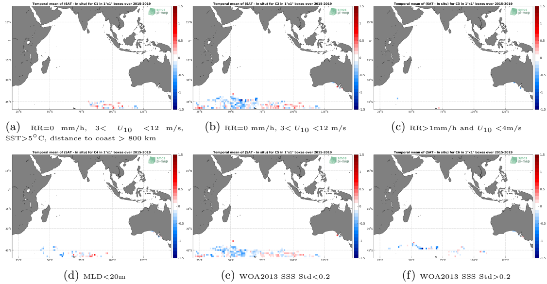
Figure 12: Temporal mean gridded over spatial boxes of size 1^\circ \times 1^\circ of \Delta SSS (SMAP SSS L3 v4 - Monthly (RSS) - Marine mammals) for 6 different subdatasets corresponding to:RR=0 mm/h, 3 < U_{10} < 12 m/s, SST >5^\circ\text{C} , distance to coast > 800 km (a), RR=0 mm/h, 3 < U_{10} < 12 m/s (b), RR >1 mm/h and U_{10} < 4 m/s (c),MLD <20 m (d),WOA2013 SSS Std <0.2 (e),WOA2013 SSS Std >0.2 (f).
