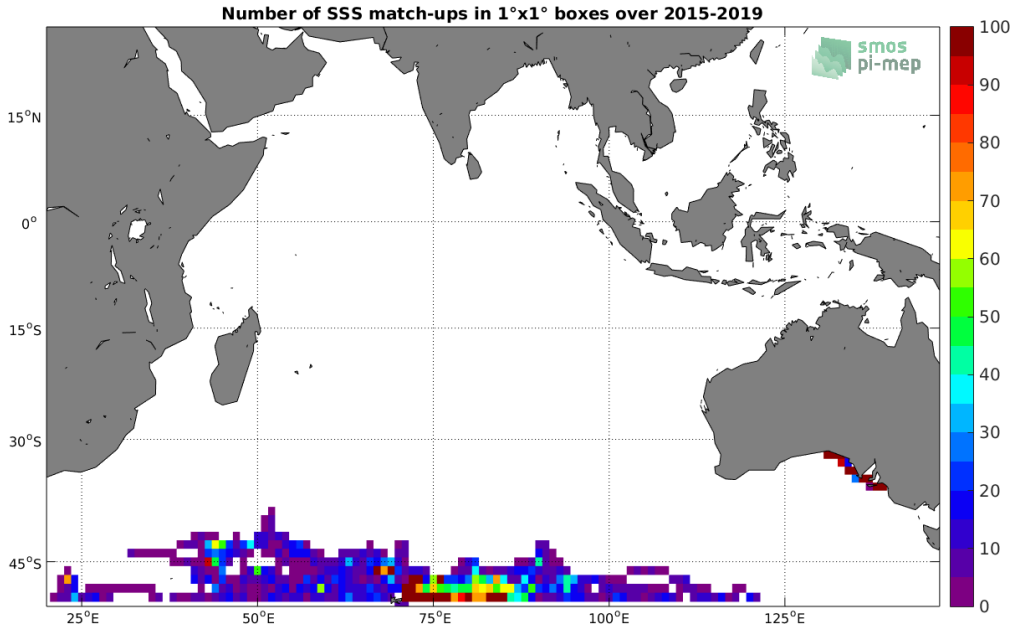
Figure 4: Number of SSS match-ups between Marine mammals SSS and the SMAP SSS L3 v4 - Monthly (RSS) SSS product for the Indian Ocean Pi-MEP region over 1^\circ \times 1^\circ boxes and for the full satellite product period.
