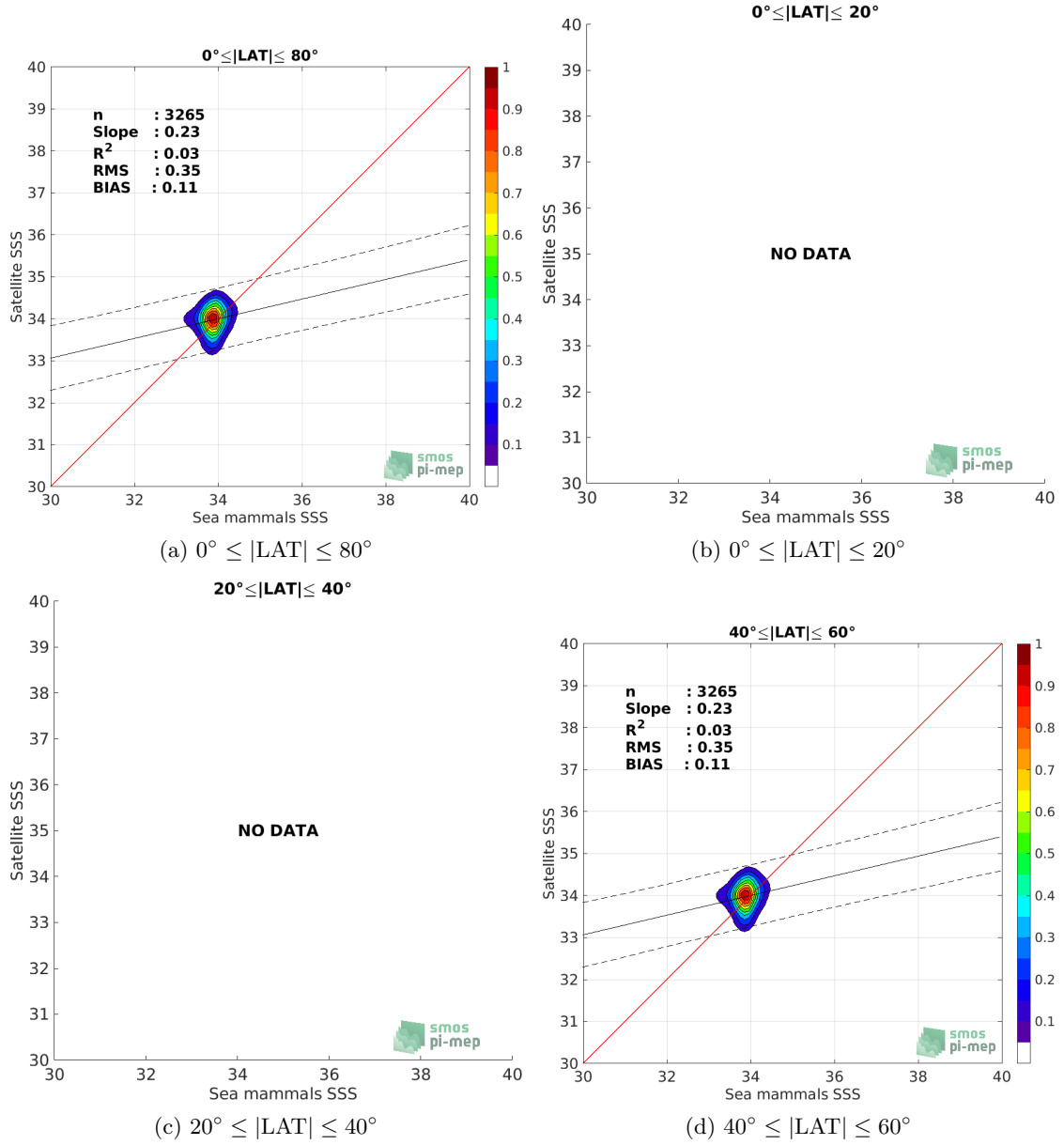
Figure 9: Contour maps of the concentration of SMAP SSS L3 v4 - Monthly (RSS) SSS (y-axis) versus Sea mammals SSS (x-axis) at match-up pairs for different latitude bands. For each plot, the red line shows x=y . The black thin and dashed lines indicate a linear fit through the data cloud and the \pm 95\% confidence levels, respectively. The number match-up pairs n , the slope and R^2 coefficient of the linear fit, the root mean square (RMS) and the mean bias between satellite and in situ data are indicated for each latitude band in each plot.
