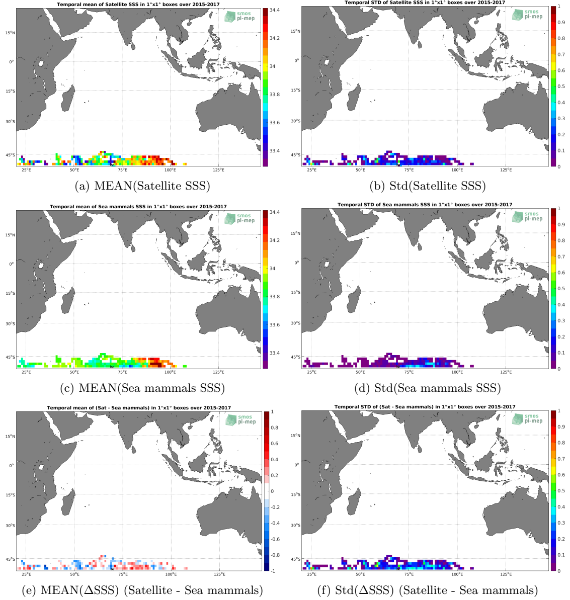
Figure 6: Temporal mean (left) and Std (right) of SSS from SMAP SSS L3 v4 - Monthly (RSS) (top), Sea mammals (middle), and of \Delta SSS (Satellite - Sea mammals). Only match-up pairs are used to generate these maps.
