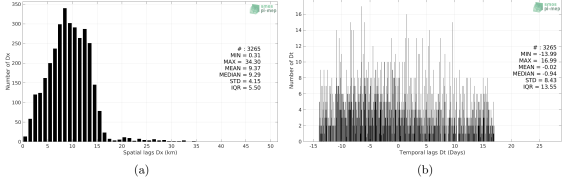
Figure 5: Histograms of the spatial (a) and temporal (b) lags between the location/time of the Sea mammals measurement and the date of the corresponding SMAP SSS L3 v4 - Monthly (RSS) SSS pixel.
