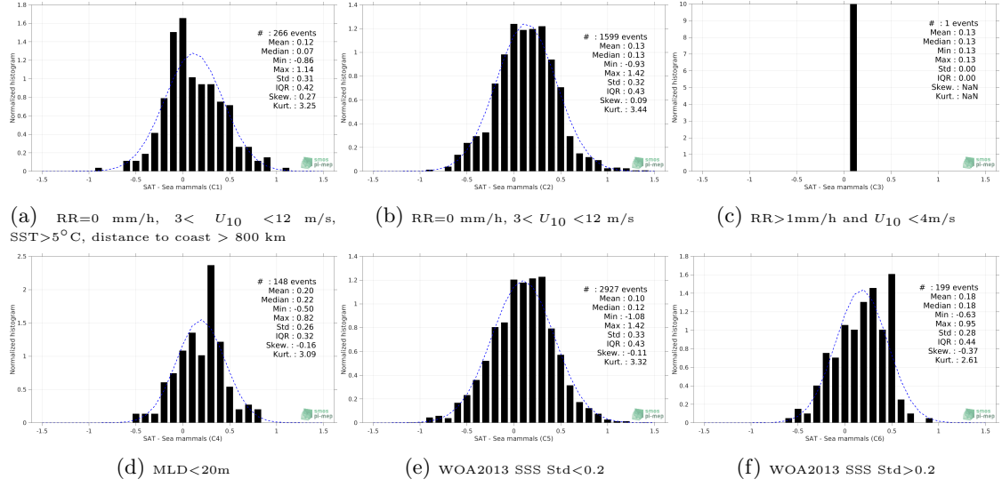
Figure 13: Normalized histogram of \Delta SSS (SMAP SSS L3 v4 - Monthly (RSS) - Sea mammals) for 6 different subdatasets corresponding to: RR=0 mm/h, 3 < U_{10} < 12 m/s, SST>5°C, distance to coast > 800 km (a), RR=0 mm/h, 3 < U_{10} < 12 m/s (b), RR>1mm/h and U_{10} < 4 m/s (c), MLD<20m (d), WOA2013 SSS Std<0.2 (e), WOA2013 SSS Std>0.2 (f).
