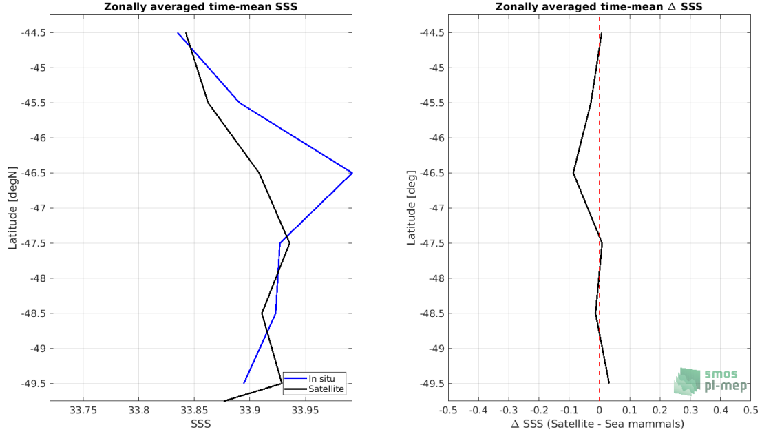
Figure 8: Left panel: Zonal mean SSS from SMAP SSS L3 v4 - Monthly (RSS) satellite product (black) and from Sea mammals (blue). Right panel: Zonal mean of \Delta SSS (Satellite - Sea mammals) for all the collected Pi-MEP match-up pairs estimated over the full satellite product period.
