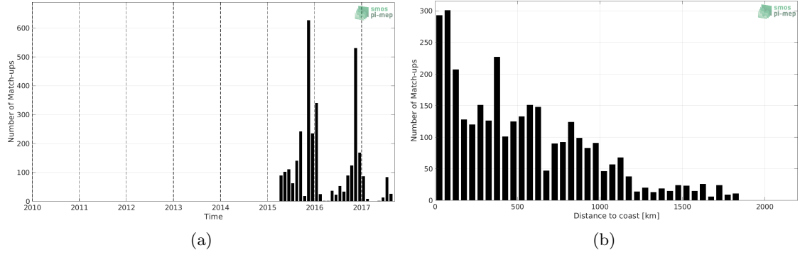
Figure 1: Number of match-ups between Sea mammals and SMAP SSS L3 v4 - Monthly (RSS) SSS as a function of time (a) and as function of the distance to coast (b) over the Indian Ocean Pi-MEP region and for the full satellite product period.
