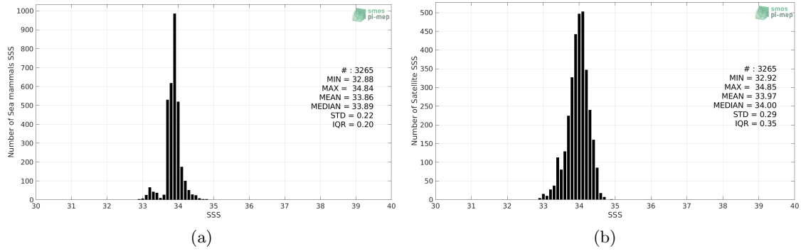
Figure 2: Histograms of SSS from Sea mammals (a) and SMAP SSS L3 v4 - Monthly (RSS) (b) considering all match-up pairs per bins of 0.1 over the Indian Ocean Pi-MEP region and for the full satellite product period.
