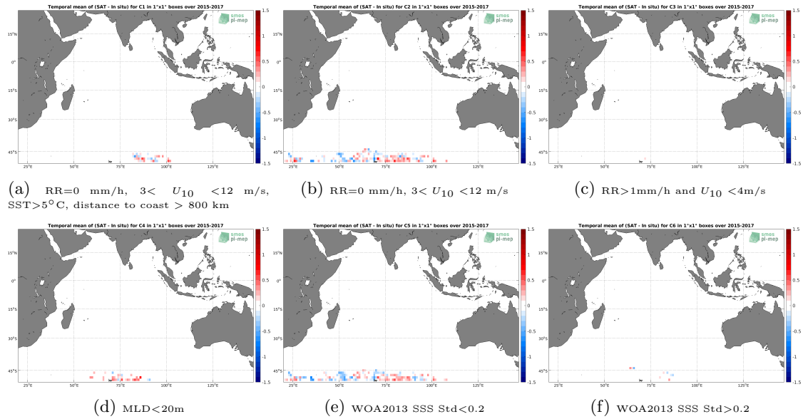
Figure 12: Temporal mean gridded over spatial boxes of size 1^{\circ}\times 1^{\circ} of \Delta\text{SSS} (SMAP SSS L3 v4 - Monthly (RSS) - Sea mammals) for 6 different subdatasets corresponding to: \text{RR}=0 mm/h, 3 < U_{10} < 12 m/s, \text{SST} > 5^{\circ}\text{C} , distance to coast > 800 km (a), \text{RR}=0 mm/h, 3 < U_{10} < 12 m/s (b), \text{RR} > 1\text{mm/h} and U_{10} < 4\text{m/s} (c), \text{MLD} < 20\text{m} (d), \text{WOA2013 SSS Std} < 0.2 (e), \text{WOA2013 SSS Std} > 0.2 (f).
