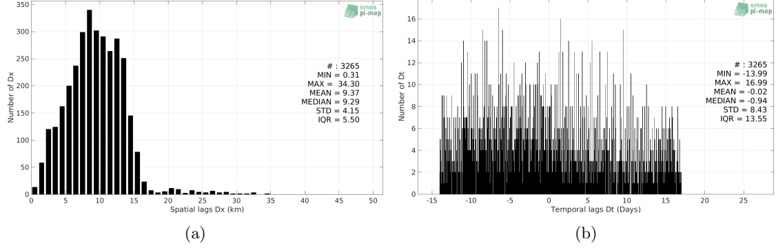
Figure 5: Histograms of the spatial (a) and temporal (b) lags between the time of the Sea mammals measurements and the date of the corresponding SMAP SSS L3 v4 - Monthly (RSS) SSS product.
