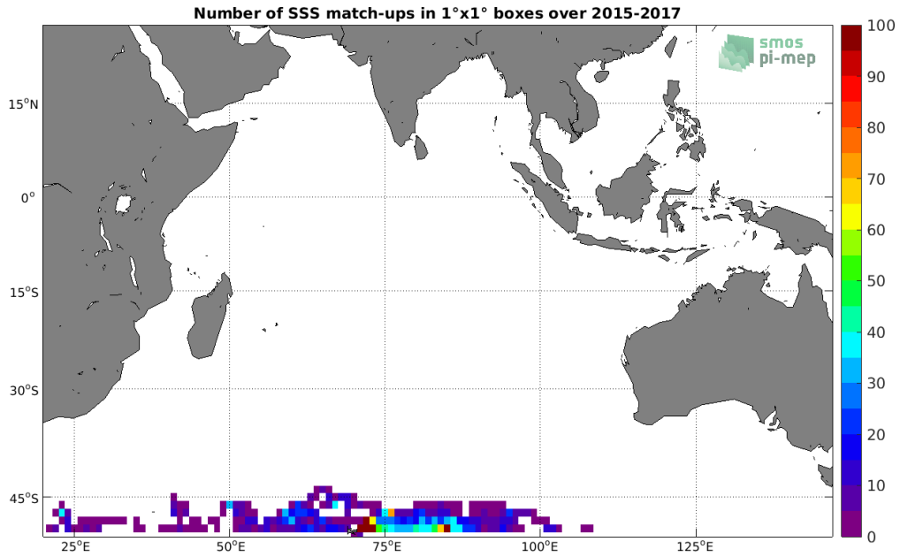
Figure 4: Number of SSS match-ups between Sea mammals SSS and the SMAP SSS L3 v4 - Monthly (RSS) SSS product for the Indian Ocean Pi-MEP region over 1°x1° boxes and for the full satellite product period.
