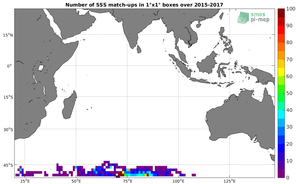
Figure 4: Number of SSS match-ups between Sea mammals SSS and the SMAP-L3-RSS-V4-MONTHLY SSS product for the Indian Ocean Pi-MEP region over 1°x1° boxes and for the full satellite product period.
