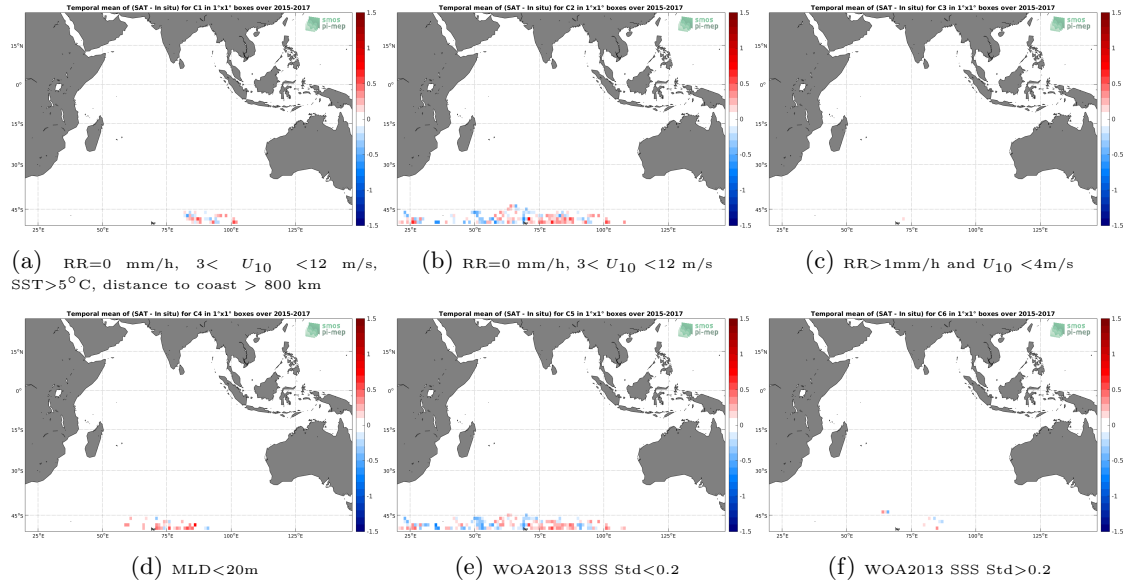
Figure 12: Temporal mean gridded over spatial boxes of size 1^{\circ}\times 1^{\circ} of \Delta\text{SSS} (SMAP-L3-RSS-V4-MONTHLY - Sea mammals) for 6 different subdatasets corresponding to:RR=0 mm/h, 3 < U_{10} < 12 m/s, SST >5^{\circ}\text{C} , distance to coast > 800 km (a), RR=0 mm/h, 3 < U_{10} < 12 m/s (b), RR >1\text{mm/h} and U_{10} < 4\text{m/s} (c),MLD <20\text{m} (d),WOA2013 SSS Std <0.2 (e),WOA2013 SSS Std >0.2 (f).
