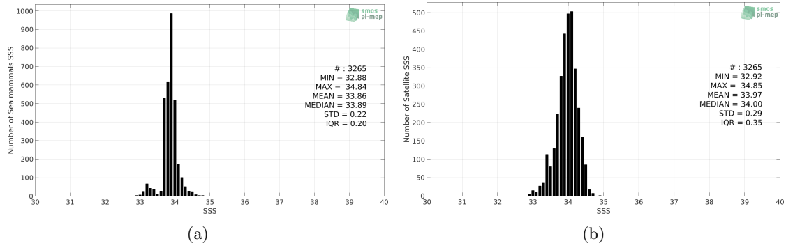
Figure 2: Histograms of SSS from Sea mammals (a) and SMAP-L3-RSS-V4-MONTHLY (b) considering all match-up pairs per bins of 0.1 over the Indian Ocean Pi-MEP region and for the full satellite product period.
