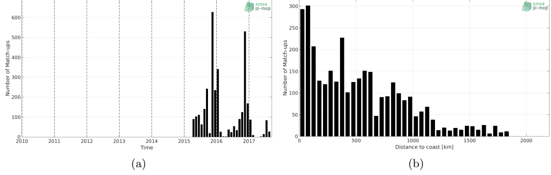
Figure 1: Number of match-ups between Sea mammals and SMAP-L3-RSS-V4-MONTHLY SSS as a function of time (a) and as function of the distance to coast (b) over the Indian Ocean Pi-MEP region and for the full satellite product period.
