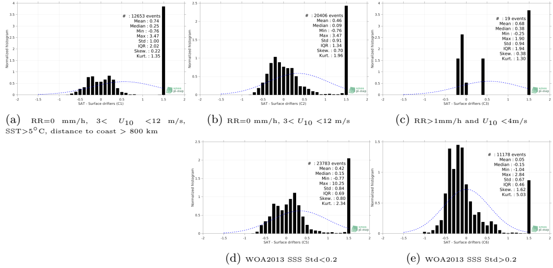
Figure 12: Normalized histogram of \Delta SSS (SMAP SSS L3 v4 - Monthly (RSS) - Surface drifters) for 5 different subdatasets corresponding to: RR=0 mm/h, 3 < U_{10} < 12 m/s, SST>5°C, distance to coast > 800 km (a), RR=0 mm/h, 3 < U_{10} < 12 m/s (b), RR>1mm/h and U_{10} < 4 m/s (c), WOA2013 SSS Std<0.2 (d), WOA2013 SSS Std>0.2 (e).
