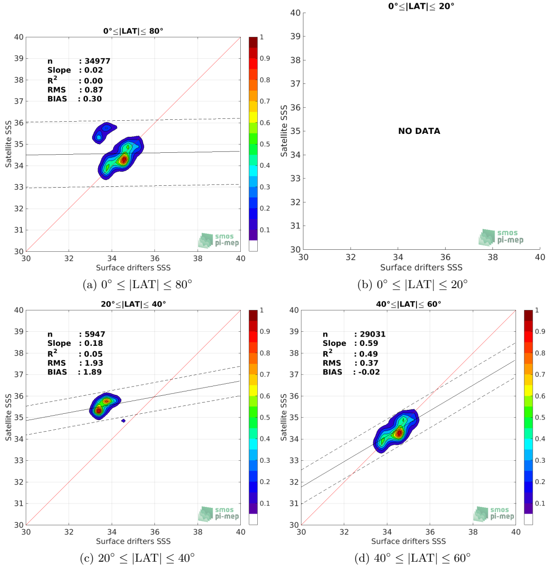
Figure 8: Contour maps of the concentration of SMAP SSS L3 v4 - Monthly (RSS) SSS (y-axis) versus Surface drifters SSS (x-axis) at match-up pairs for different latitude bands. For each plot, the red line shows x=y . The black thin and dashed lines indicate a linear fit through the data cloud and the \pm 95\% confidence levels, respectively. The number match-up pairs n , the slope and R^2 coefficient of the linear fit, the root mean square (RMS) and the mean bias between satellite and in situ data are indicated for each latitude band in each plots.
