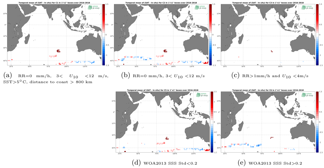
Figure 11: Temporal mean gridded over spatial boxes of size 1^\circ \times 1^\circ of \Delta SSS (SMAP SSS L3 v4 - Monthly (RSS) - Surface drifters) for 5 different subdatasets corresponding to: RR=0 mm/h, 3 < U_{10} < 12 m/s, SST > 5^\circ C , distance to coast > 800 km (a), RR=0 mm/h, 3 < U_{10} < 12 m/s (b), RR > 1 mm/h and U_{10} < 4 m/s (c), WOA2013 SSS Std < 0.2 (d), WOA2013 SSS Std > 0.2 (e).
