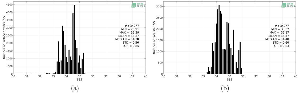
Figure 2: Histograms of SSS from Surface drifters (a) and SMAP SSS L3 v4 - Monthly (RSS) (b) considering all match-up pairs per bins of 0.1 over the Indian Ocean Pi-MEP region and for the full satellite product period.
