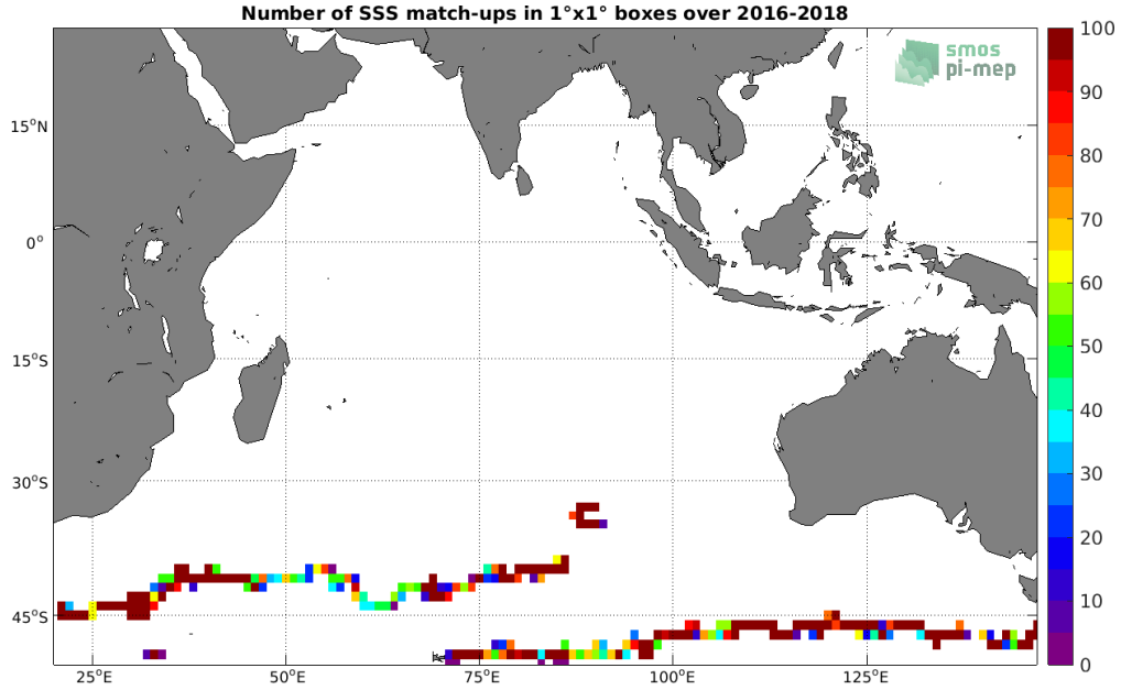
Figure 3: Number of SSS match-ups between Surface drifters SSS and the SMAP SSS L3 v4 - Monthly (RSS) SSS product for the Indian Ocean Pi-MEP region over 1^\circ \times 1^\circ boxes and for the full satellite product period.
