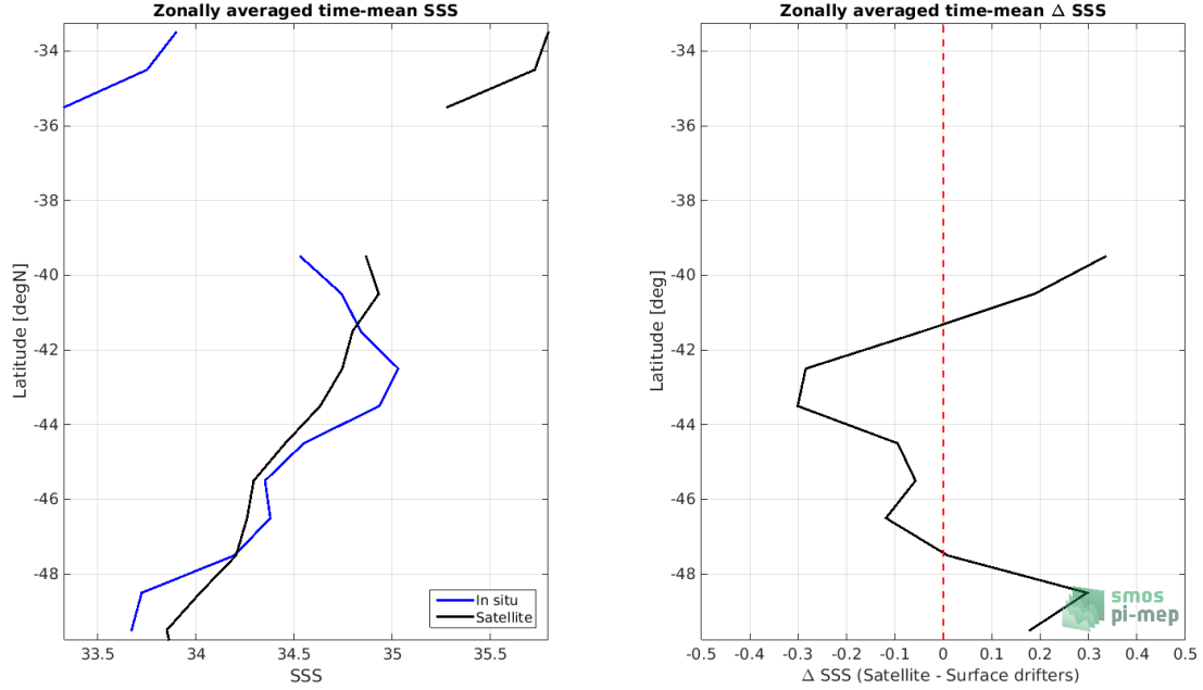
Figure 7: Left panel: Zonal mean SSS from SMAP SSS L3 v4 - Monthly (RSS) satellite product (black) and from Surface drifters (blue). Right panel: Zonal mean of \Delta SSS (Satellite - Surface drifters) for all the collected Pi-MEP match-up pairs estimated over the full satellite product period.
