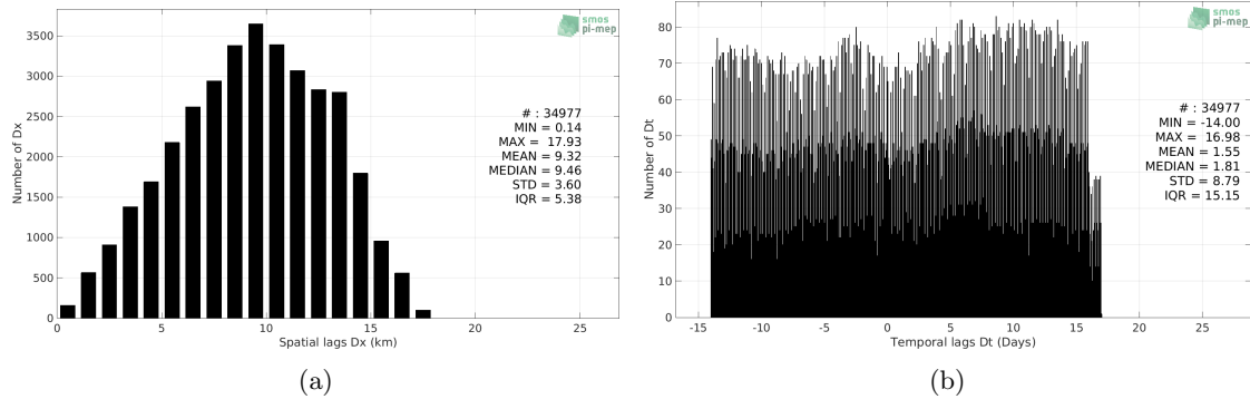
Figure 4: Histograms of the spatial (a) and temporal (b) lags between the time of the Surface drifters measurements and the date of the corresponding SMAP SSS L3 v4 - Monthly (RSS) SSS product.
