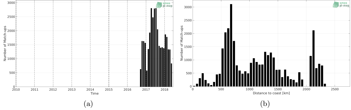
Figure 1: Number of match-ups between Surface drifters and SMAP SSS L3 v4 - Monthly (RSS) SSS as a function of time (a) and as function of the distance to coast (b) over the Indian Ocean Pi-MEP region and for the full satellite product period.
