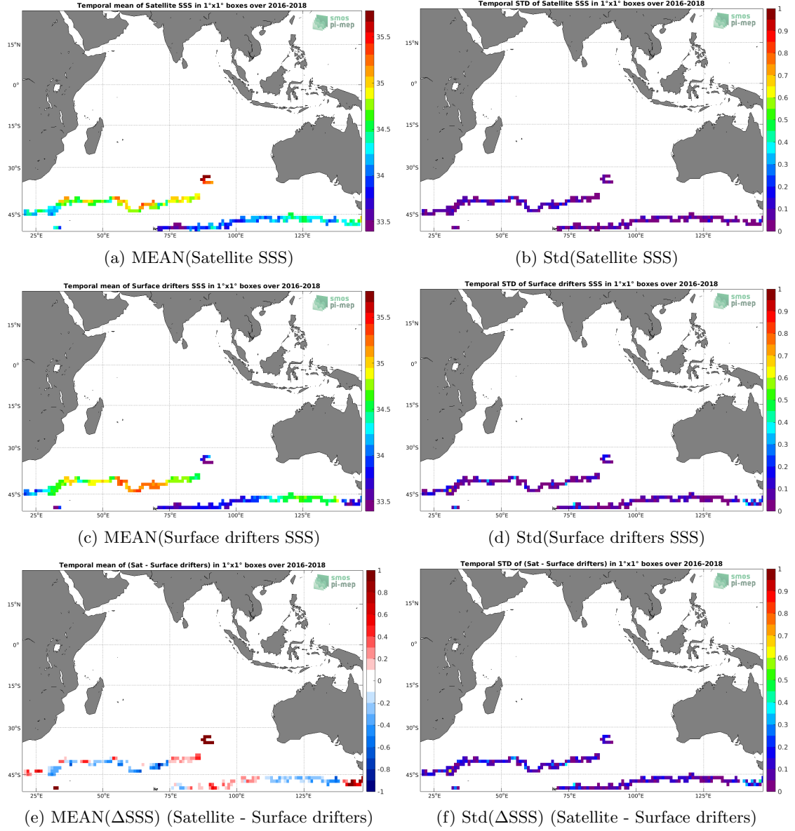
Figure 5: Temporal mean (left) and Std (right) of SSS from SMAP SSS L3 v4 - Monthly (RSS) (top), Surface drifters (middle), and of \Delta SSS (Satellite - Surface drifters). Only match-up pairs are used to generate these maps.
