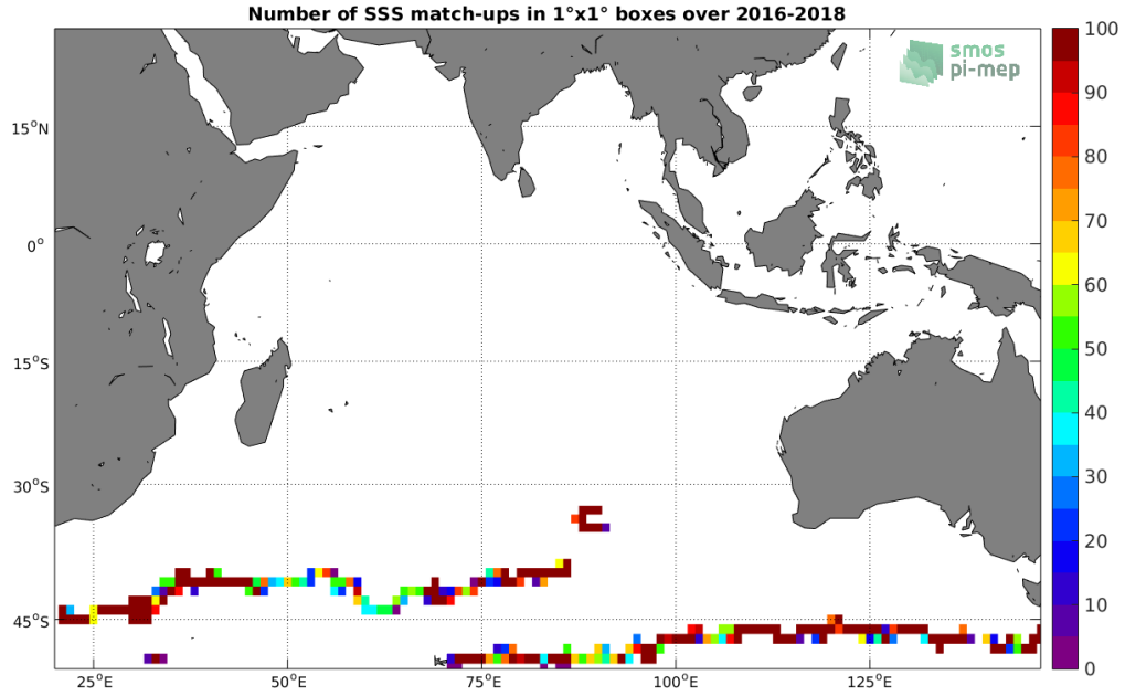
Figure 3: Number of SSS match-ups between Surface drifters SSS and the SMAP-L3-RSS-V4-MONTHLY SSS product for the Indian Ocean Pi-MEP region over 1°x1° boxes and for the full satellite product period.
