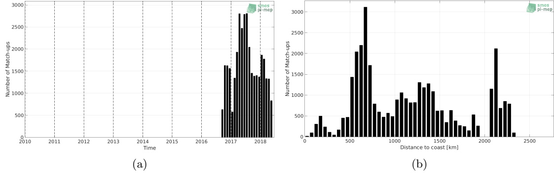
Figure 1: Number of match-ups between Surface drifters and SMAP-L3-RSS-V4-MONTHLY SSS as a function of time (a) and as function of the distance to coast (b) over the Indian Ocean Pi-MEP region and for the full satellite product period.
