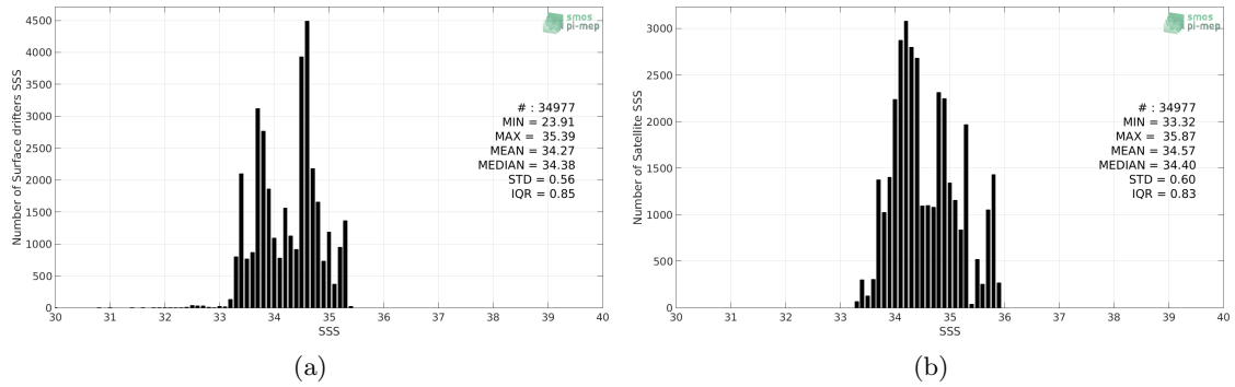
Figure 2: Histograms of SSS from Surface drifters (a) and SMAP-L3-RSS-V4-MONTHLY (b) considering all match-up pairs per bins of 0.1 over the Indian Ocean Pi-MEP region and for the full satellite product period.
