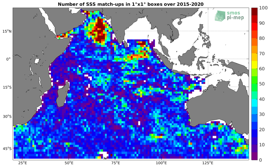
Figure 4: Number of SSS match-ups between Argo SSS and the SMAP SSS L3 v4 - Monthly (RSS) SSS product for the Indian Ocean Pi-MEP region over 1°x1° boxes and for the full satellite product period.
