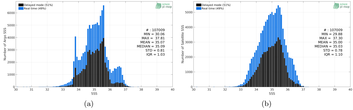
Figure 2: Histograms of SSS from Argo (a) and SMAP-L3-RSS-V4-MONTHLY (b) considering all match-up pairs per bins of 0.1 over the Indian Ocean Pi-MEP region and for the full satellite product period.
