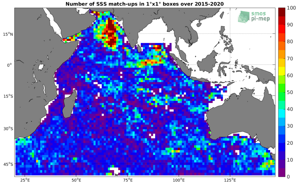
Figure 4: Number of SSS match-ups between Argo SSS and the SMAP-L3-RSS-V4-MONTHLY SSS product for the Indian Ocean Pi-MEP region over 1^\circ \times 1^\circ boxes and for the full satellite product period.
