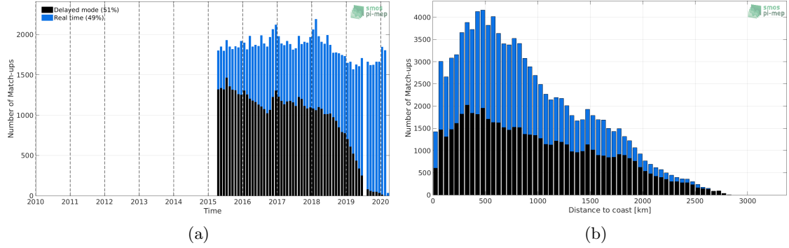
Figure 1: Number of match-ups between Argo and SMAP-L3-RSS-V4-MONTHLY SSS as a function of time (a) and as function of the distance to coast (b) over the Indian Ocean Pi-MEP region and for the full satellite product period.
