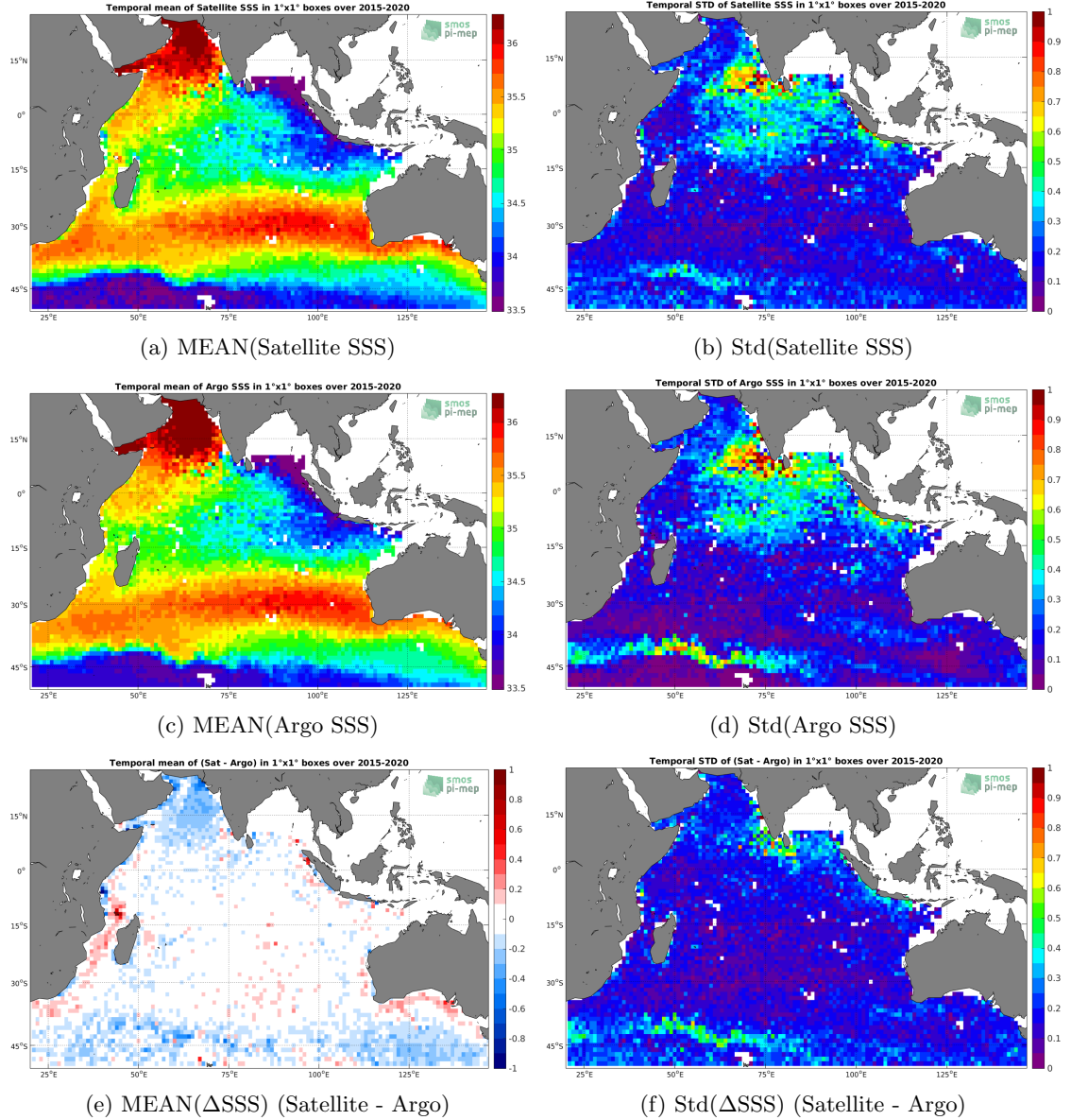
Figure 6: Temporal mean (left) and Std (right) of SSS from SMAP-L3-RSS-V4-MONTHLY (top), Argo (middle), and of \Delta SSS (Satellite - Argo). Only match-up pairs are used to generate these maps.
