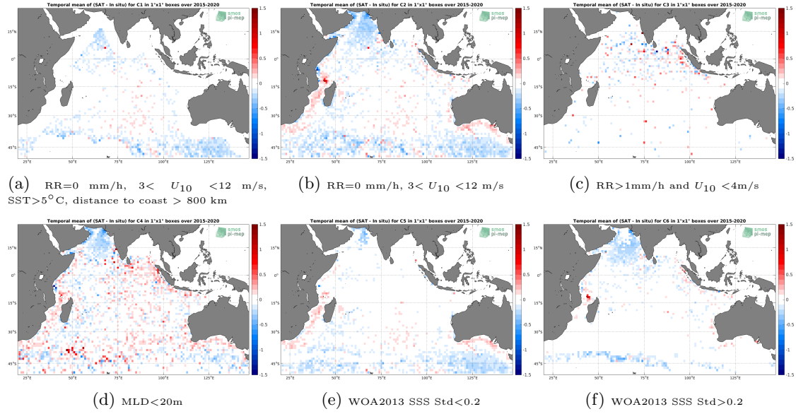
Figure 12: Temporal mean gridded over spatial boxes of size 1^\circ \times 1^\circ of \Delta SSS (SMAP-L3-RSS-V4-MONTHLY - Argo) for 6 different subdatasets corresponding to: RR=0 mm/h, 3 < U_{10} < 12 m/s, SST > 5^\circ\text{C} , distance to coast > 800 km (a), RR=0 mm/h, 3 < U_{10} < 12 m/s (b), RR > 1 mm/h and U_{10} < 4 m/s (c), MLD < 20 m (d), WOA2013 SSS Std < 0.2 (e), WOA2013 SSS Std > 0.2 (f).
