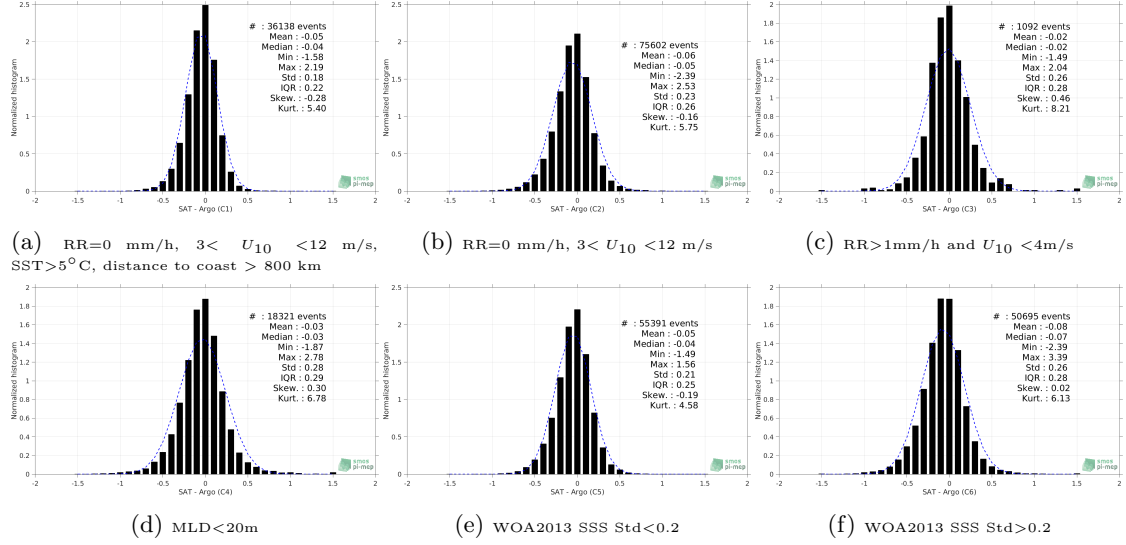
Figure 13: Normalized histogram of \Delta\text{SSS} (SMAP-L3-RSS-V4-MONTHLY - Argo) for 6 different subdatasets corresponding to: RR=0 mm/h, 3 < U_{10} < 12 m/s, SST>5°C, distance to coast > 800 km (a), RR=0 mm/h, 3 < U_{10} < 12 m/s (b), RR>1mm/h and U_{10} < 4 m/s (c), MLD<20m (d), WOA2013 SSS Std<0.2 (e), WOA2013 SSS Std>0.2 (f).
