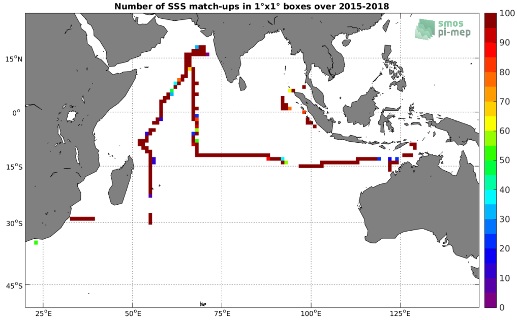
Figure 4: Number of SSS match-ups between TSG-SAMOS SSS and the SMAP-L3-RSS-V3-8DAY-RUNNING-70KM SSS product for the Indian Ocean Pi-MEP region over 1^\circ \times 1^\circ boxes and for the full satellite product period.
