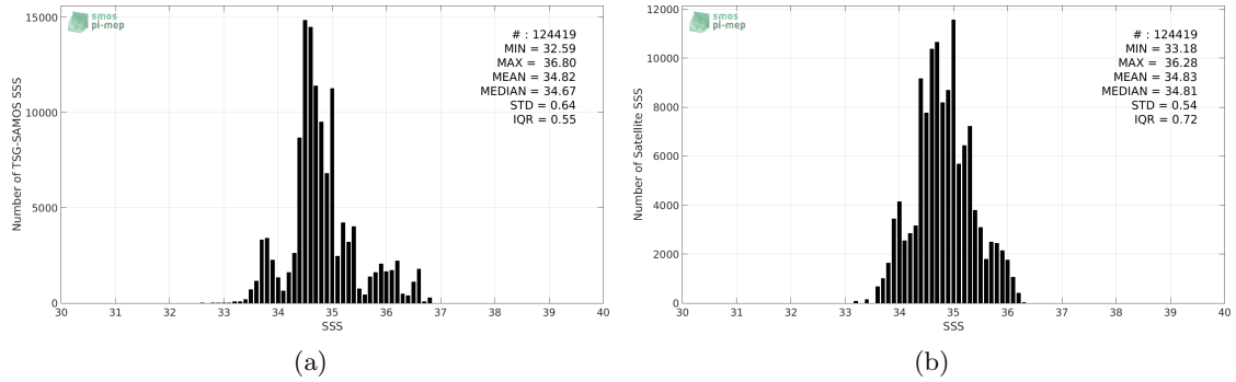
Figure 2: Histograms of SSS from TSG-SAMOS (a) and SMAP-L3-RSS-V3-8DAY-RUNNING-70KM (b) considering all match-up pairs per bins of 0.1 over the Indian Ocean Pi-MEP region and for the full satellite product period.
