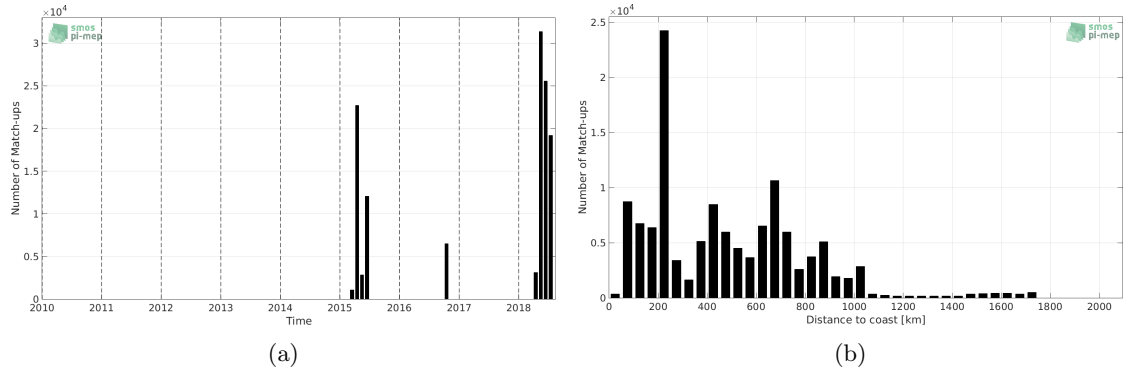
Figure 1: Number of match-ups between TSG-SAMOS and SMAP-L3-RSS-V3-8DAY-RUNNING-70KM SSS as a function of time (a) and as function of the distance to coast (b) over the Indian Ocean Pi-MEP region and for the full satellite product period.
