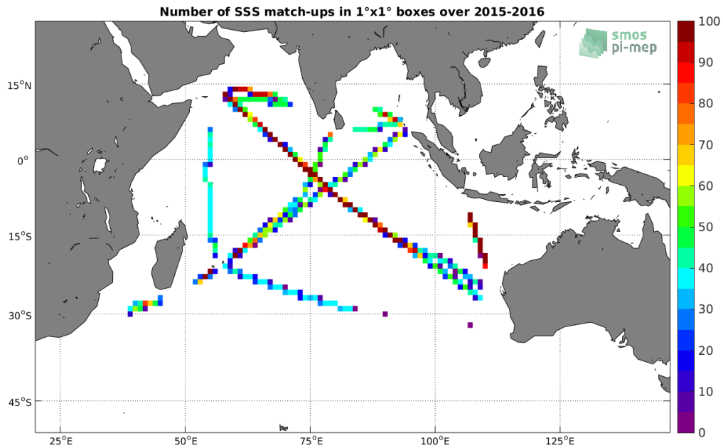
Figure 4: Number of SSS match-ups between TSG-LEGOS-DM SSS and the SMAP-L3-RSS-V3-8DAY-RUNNING-70KM SSS product for the Indian Ocean Pi-MEP region over 1^\circ \times 1^\circ boxes and for the full satellite product period.
