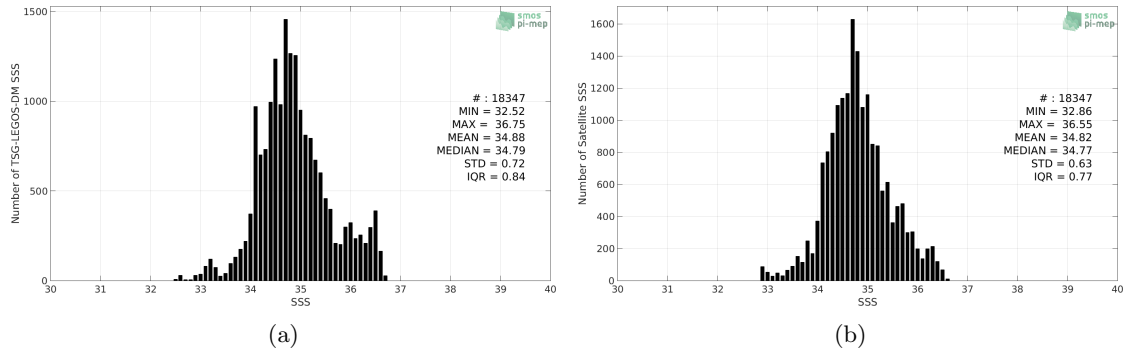
Figure 2: Histograms of SSS from TSG-LEGOS-DM (a) and SMAP-L3-RSS-V3-8DAY-RUNNING-70KM (b) considering all match-up pairs per bins of 0.1 over the Indian Ocean Pi-MEP region and for the full satellite product period.
