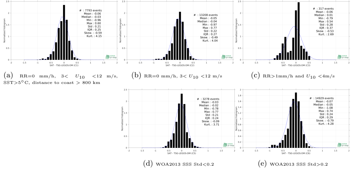
Figure 13: Normalized histogram of \Delta\text{SSS} (SMAP-L3-RSS-V3-8DAY-RUNNING-70KM - TSG-LEGOS-DM) for 5 different subdatasets corresponding to: RR=0 mm/h, 3 < U_{10} < 12 m/s, SST > 5^{\circ}\text{C} , distance to coast > 800 km (a), RR=0 mm/h, 3 < U_{10} < 12 m/s (b), RR > 1\text{mm/h} and U_{10} < 4\text{m/s} (c), WOA2013 SSS Std < 0.2 (d), WOA2013 SSS Std > 0.2 (e).
