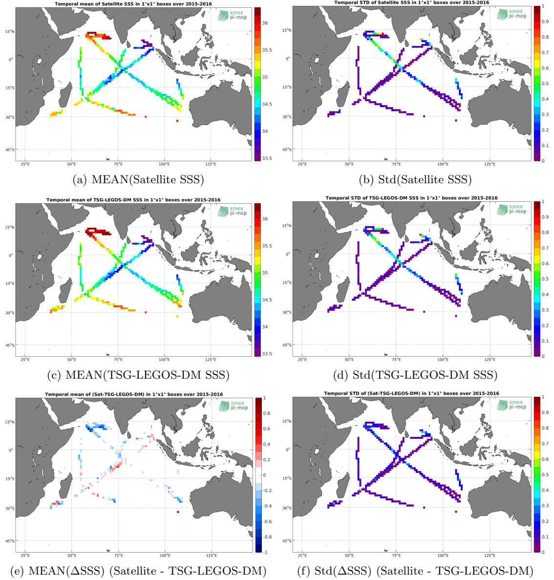
Figure 6: Temporal mean (left) and Std (right) of SSS from SMAP-L3-RSS-V3-8DAY-RUNNING-70KM (top), TSG-LEGOS-DM (middle), and of \Delta SSS (Satellite - TSG-LEGOS-DM). Only match-up pairs are used to generate these maps.
