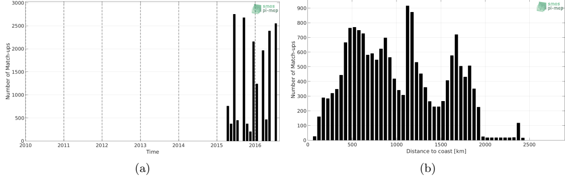
Figure 1: Number of match-ups between TSG-LEGOS-DM and SMAP-L3-RSS-V3-8DAY-RUNNING-70KM SSS as a function of time (a) and as function of the distance to coast (b) over the Indian Ocean Pi-MEP region and for the full satellite product period.
