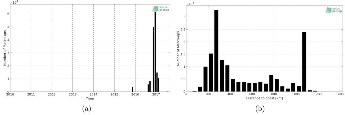
Figure 1: Number of match-ups between TSG-GOSUD-Research-vessel and SMAP-L3-RSS-V3-8DAY-RUNNING-70KM SSS as a function of time (a) and as function of the distance to coast (b) over the Indian Ocean Pi-MEP region and for the full satellite product period.
