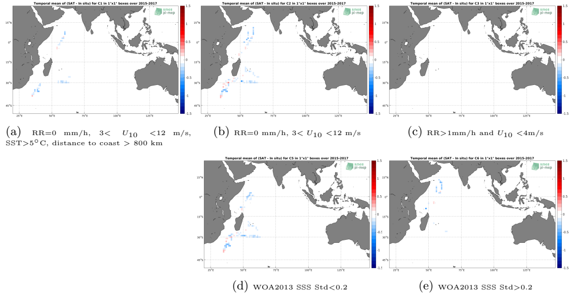
Figure 12: Temporal mean gridded over spatial boxes of size 1^\circ \times 1^\circ of \Delta SSS (SMAP-L3-RSS-V3-8DAY-RUNNING-70KM - TSG-GOSUD-Research-vessel) for 5 different subdatasets corresponding to: RR=0 mm/h, 3 < U_{10} < 12 m/s, SST > 5^\circ C , distance to coast > 800 km (a), RR=0 mm/h, 3 < U_{10} < 12 m/s (b), RR > 1 mm/h and U_{10} < 4 m/s (c), WOA2013 SSS Std < 0.2 (d), WOA2013 SSS Std > 0.2 (e).
