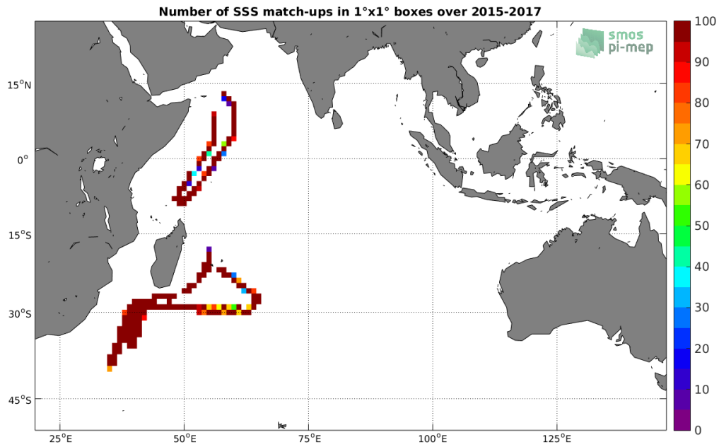
Figure 4: Number of SSS match-ups between TSG-GOSUD-Research-vessel SSS and the SMAP-L3-RSS-V3-8DAY-RUNNING-70KM SSS product for the Indian Ocean Pi-MEP region over 1^\circ \times 1^\circ boxes and for the full satellite product period.
