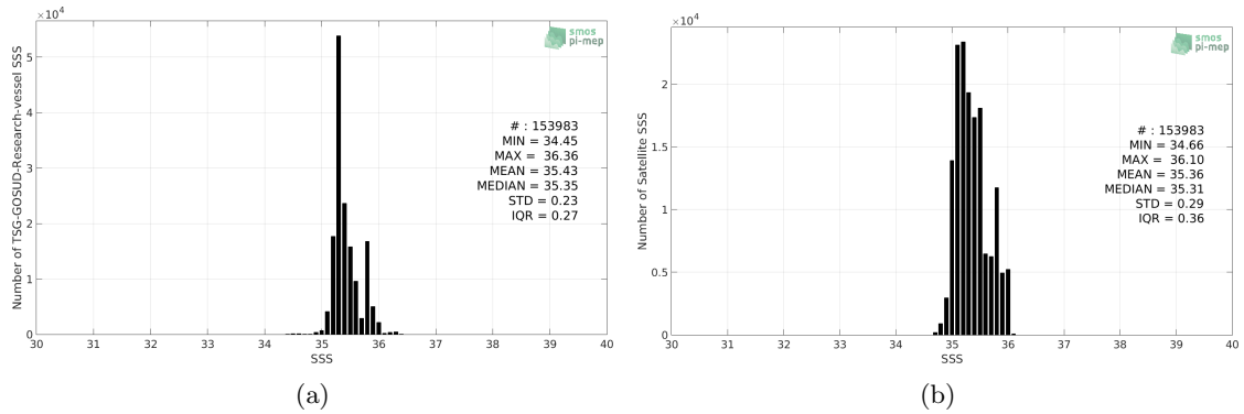
Figure 2: Histograms of SSS from TSG-GOSUD-Research-vessel (a) and SMAP-L3-RSS-V3-8DAY-RUNNING-70KM (b) considering all match-up pairs per bins of 0.1 over the Indian Ocean Pi-MEP region and for the full satellite product period.
