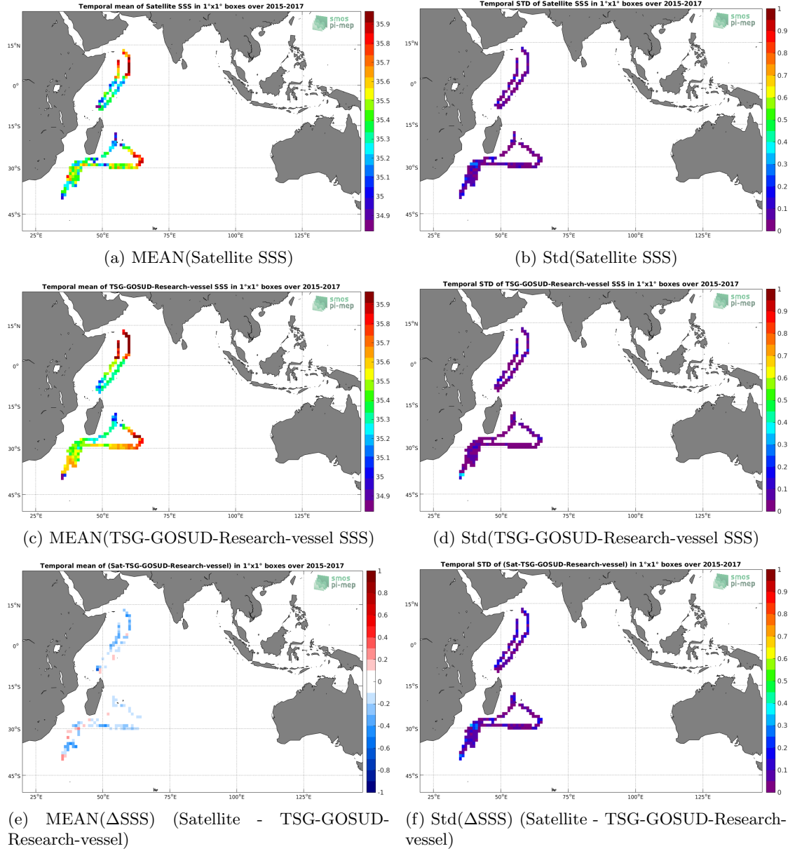
Figure 6: Temporal mean (left) and Std (right) of SSS from SMAP-L3-RSS-V3-8DAY-RUNNING-70KM (top), TSG-GOSUD-Research-vessel (middle), and of \Delta SSS (Satellite - TSG-GOSUD-Research-vessel). Only match-up pairs are used to generate these maps.
