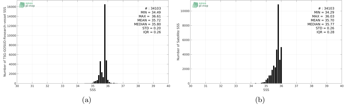
Figure 2: Histograms of SSS from TSG-GOSUD-Research-vessel (a) and SMAP-L3-RSS-V3-8DAY-RUNNING-70KM (b) considering all match-up pairs per bins of 0.1 over the Indian Ocean Pi-MEP region and for the full satellite product period.
