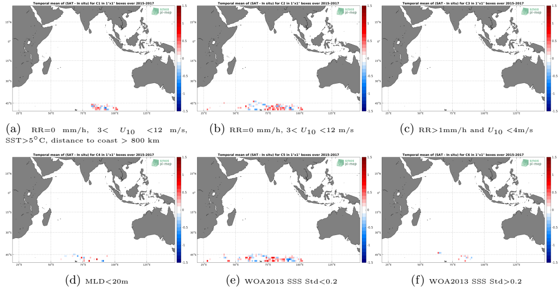
Figure 12: Temporal mean gridded over spatial boxes of size 1^\circ \times 1^\circ of \Delta SSS (SMAP-L3-RSS-V3-8DAY-RUNNING-70KM - Sea mammals) for 6 different subdatasets corresponding to: RR=0 mm/h, 3 < U_{10} < 12 m/s, SST > 5^\circ C , distance to coast > 800 km (a), RR=0 mm/h, 3 < U_{10} < 12 m/s (b), RR > 1 mm/h and U_{10} < 4 m/s (c), MLD < 20 m (d), WOA2013 SSS Std < 0.2 (e), WOA2013 SSS Std > 0.2 (f).
