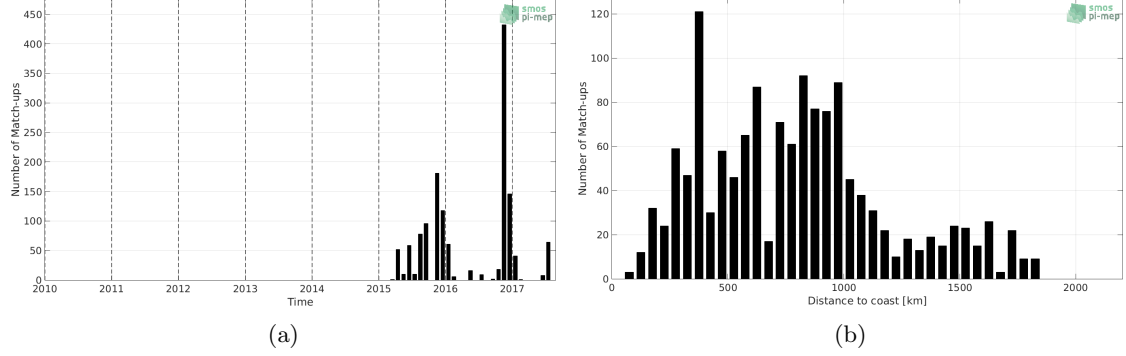
Figure 1: Number of match-ups between Sea mammals and SMAP-L3-RSS-V3-8DAY-RUNNING-70KM SSS as a function of time (a) and as function of the distance to coast (b) over the Indian Ocean Pi-MEP region and for the full satellite product period.
