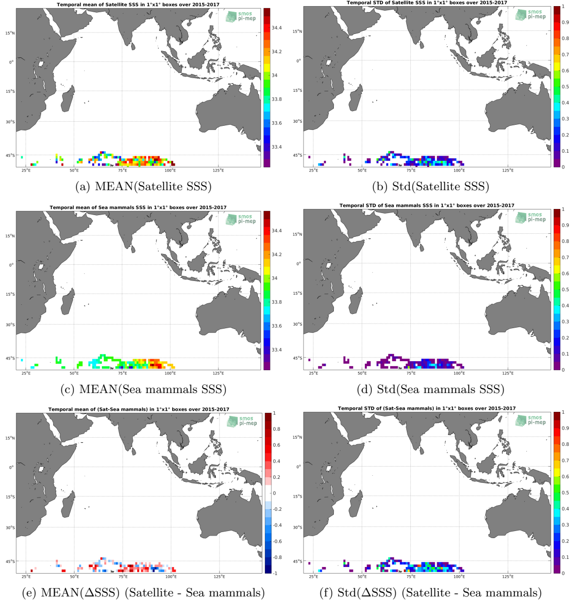
Figure 6: Temporal mean (left) and Std (right) of SSS from SMAP-L3-RSS-V3-8DAY-RUNNING-70KM (top), Sea mammals (middle), and of \Delta SSS (Satellite - Sea mammals). Only match-up pairs are used to generate these maps.
