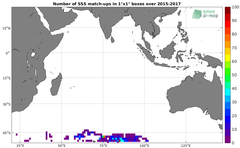
Figure 4: Number of SSS match-ups between Sea mammals SSS and the SMAP-L3-RSS-V3-8DAY-RUNNING-70KM SSS product for the Indian Ocean Pi-MEP region over 1^\circ \times 1^\circ boxes and for the full satellite product period.
