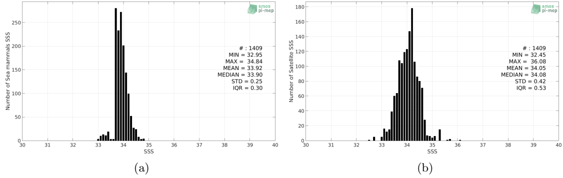
Figure 2: Histograms of SSS from Sea mammals (a) and SMAP-L3-RSS-V3-8DAY-RUNNING-70KM (b) considering all match-up pairs per bins of 0.1 over the Indian Ocean Pi-MEP region and for the full satellite product period.
