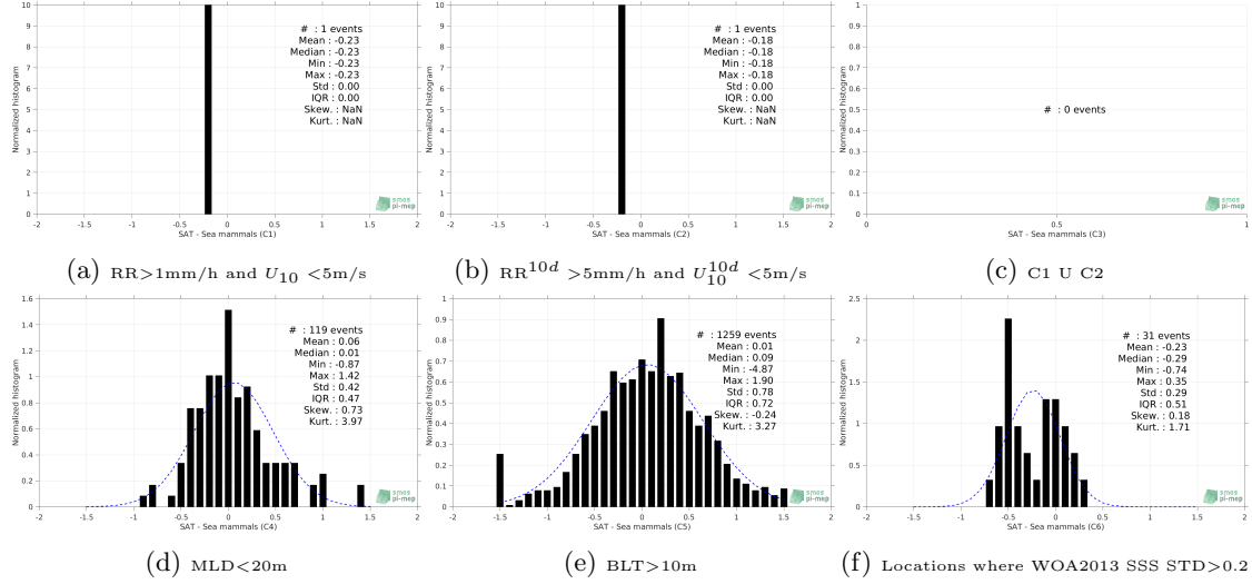
Figure 13: Normalized histogram of \Delta SSS (SMAP-L3-RSS-V3-8DAY-RUNNING-70KM - Sea mammals) for 6 different subdatasets corresponding to: RR > 1\text{mm/h} and U_{10} < 5\text{m/s} (a), RR^{10d} > 5\text{mm/h} and U_{10}^{10d} < 5\text{m/s} (b), C1 U C2 (c), MLD < 20\text{m} (d), BLT > 10\text{m} (e), Locations where WOA2013 SSS STD > 0.2 (f).
