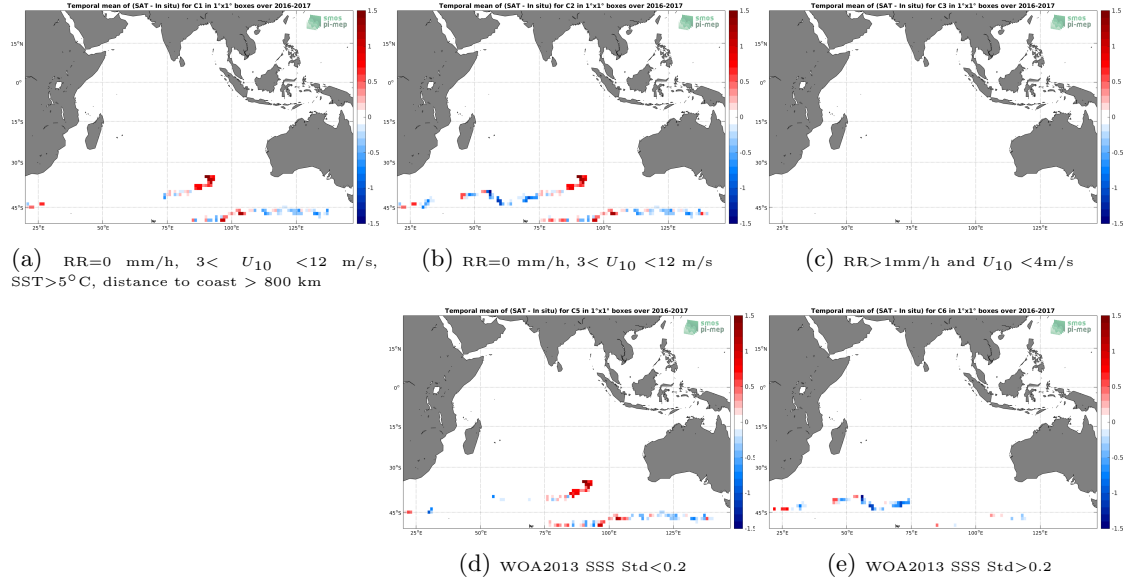
Figure 11: Temporal mean gridded over spatial boxes of size 1^\circ \times 1^\circ of \Delta SSS (SMAP-L3-RSS-V3-8DAY-RUNNING-70KM - Surface drifters) for 5 different subdatasets corresponding to: RR=0 mm/h, 3 < U_{10} < 12 m/s, SST > 5^\circ\text{C} , distance to coast > 800 km (a), RR=0 mm/h, 3 < U_{10} < 12 m/s (b), RR > 1 mm/h and U_{10} < 4 m/s (c), WOA2013 SSS Std < 0.2 (d), WOA2013 SSS Std > 0.2 (e).
