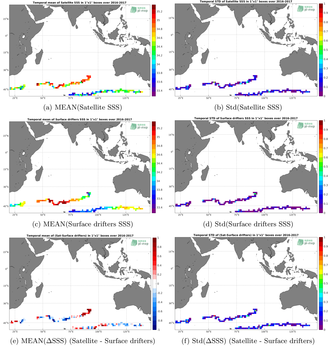
Figure 5: Temporal mean (left) and Std (right) of SSS from SMAP-L3-RSS-V3-8DAY-RUNNING-70KM (top), Surface drifters (middle), and of \Delta SSS (Satellite - Surface drifters). Only match-up pairs are used to generate these maps.
