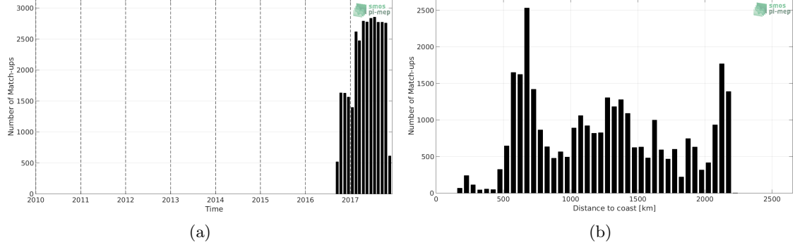
Figure 1: Number of match-ups between Surface drifters and SMAP-L3-RSS-V3-8DAY-RUNNING-70KM SSS as a function of time (a) and as function of the distance to coast (b) over the Indian Ocean Pi-MEP region and for the full satellite product period.
