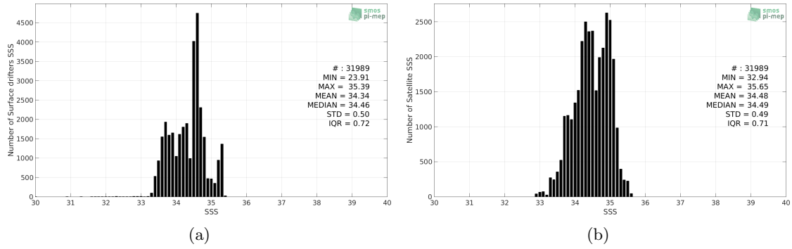
Figure 2: Histograms of SSS from Surface drifters (a) and SMAP-L3-RSS-V3-8DAY-RUNNING-70KM (b) considering all match-up pairs per bins of 0.1 over the Indian Ocean Pi-MEP region and for the full satellite product period.
