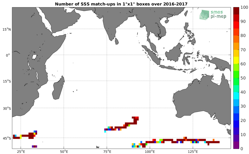
Figure 3: Number of SSS match-ups between Surface drifters SSS and the SMAP-L3-RSS-V3-8DAY-RUNNING-70KM SSS product for the Indian Ocean Pi-MEP region over 1^\circ \times 1^\circ boxes and for the full satellite product period.
