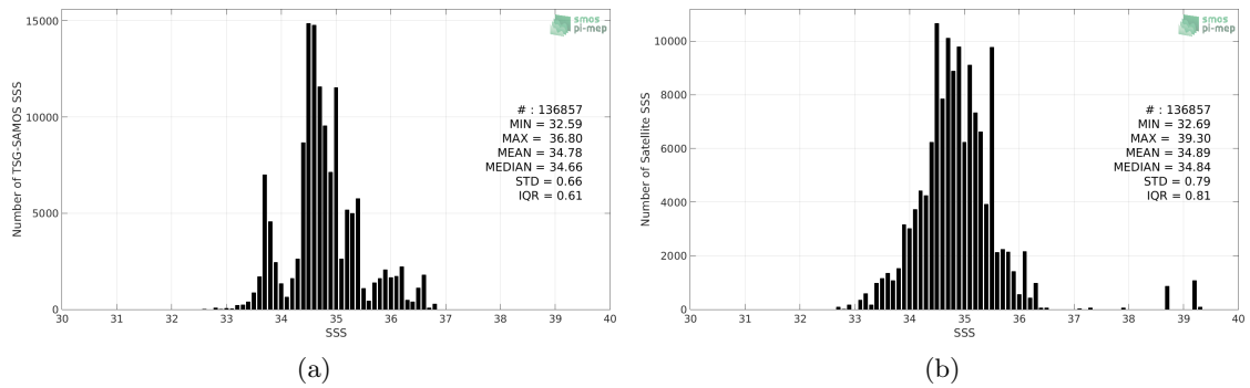
Figure 2: Histograms of SSS from TSG-SAMOS (a) and SMAP-L3-RSS-V3-8DAY-RUNNING-40KM (b) considering all match-up pairs per bins of 0.1 over the Indian Ocean Pi-MEP region and for the full satellite product period.
