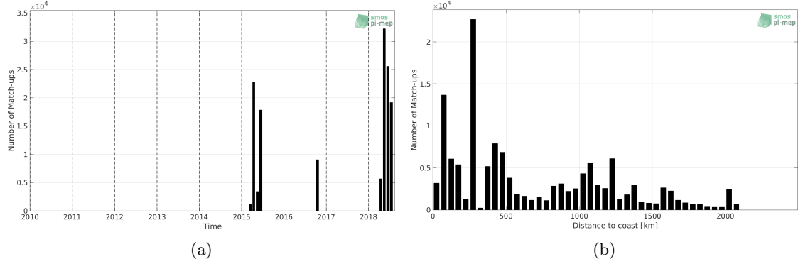
Figure 1: Number of match-ups between TSG-SAMOS and SMAP-L3-RSS-V3-8DAY-RUNNING-40KM SSS as a function of time (a) and as function of the distance to coast (b) over the Indian Ocean Pi-MEP region and for the full satellite product period.
