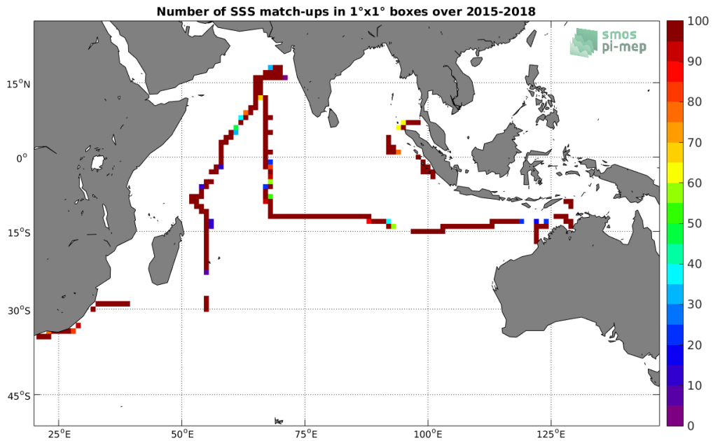
Figure 4: Number of SSS match-ups between TSG-SAMOS SSS and the SMAP-L3-RSS-V3-8DAY-RUNNING-40KM SSS product for the Indian Ocean Pi-MEP region over 1^{\circ} \times 1^{\circ} boxes and for the full satellite product period.
