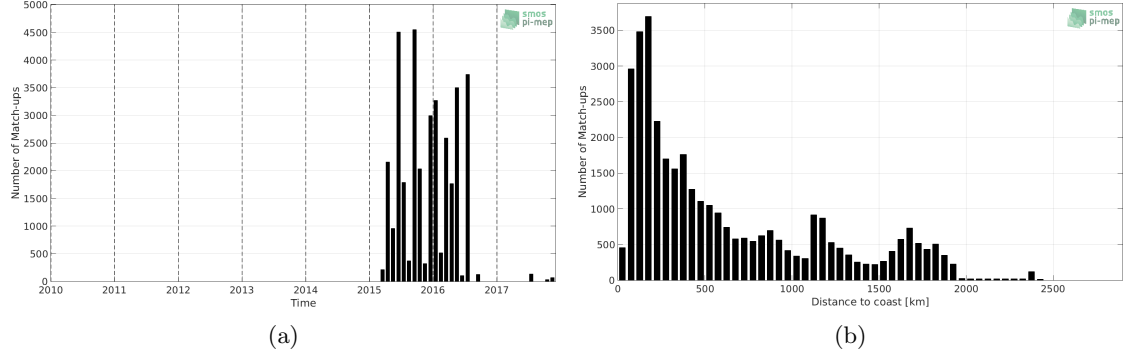
Figure 1: Number of match-ups between TSG-LEGOS-DM and SMAP-L3-RSS-V3-8DAY-RUNNING-40KM SSS as a function of time (a) and as function of the distance to coast (b) over the Indian Ocean Pi-MEP region and for the full satellite product period.
