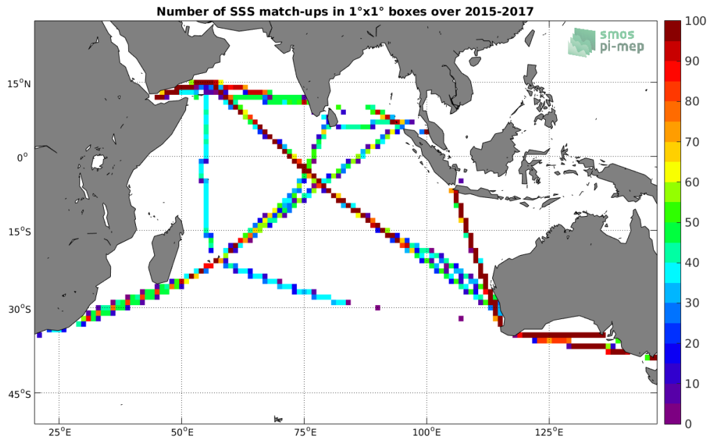
Figure 4: Number of SSS match-ups between TSG-LEGOS-DM SSS and the SMAP-L3-RSS-V3-8DAY-RUNNING-40KM SSS product for the Indian Ocean Pi-MEP region over 1^\circ \times 1^\circ boxes and for the full satellite product period.
