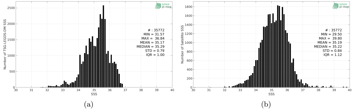
Figure 2: Histograms of SSS from TSG-LEGOS-DM (a) and SMAP-L3-RSS-V3-8DAY-RUNNING-40KM (b) considering all match-up pairs per bins of 0.1 over the Indian Ocean Pi-MEP region and for the full satellite product period.
