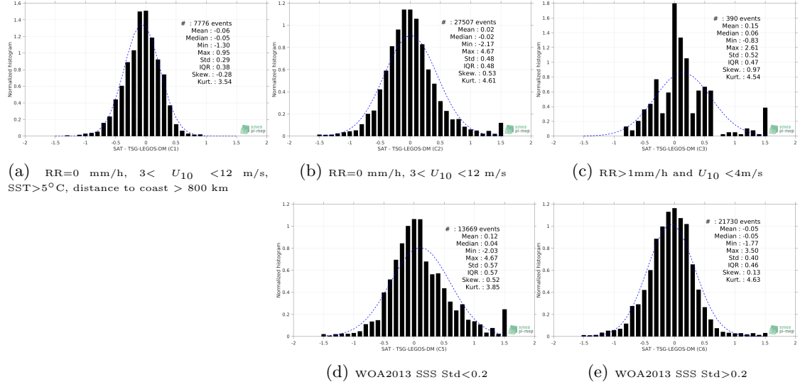
Figure 13: Normalized histogram of \Delta\text{SSS} (SMAP-L3-RSS-V3-8DAY-RUNNING-40KM - TSG-LEGOS-DM) for 5 different subdatasets corresponding to: RR=0 mm/h, 3 < U_{10} < 12 m/s, SST >5^{\circ}\text{C} , distance to coast > 800 km (a), RR=0 mm/h, 3 < U_{10} < 12 m/s (b), RR>1\text{mm/h} and U_{10} < 4\text{m/s} (c), WOA2013 SSS Std <0.2 (d), WOA2013 SSS Std >0.2 (e).
