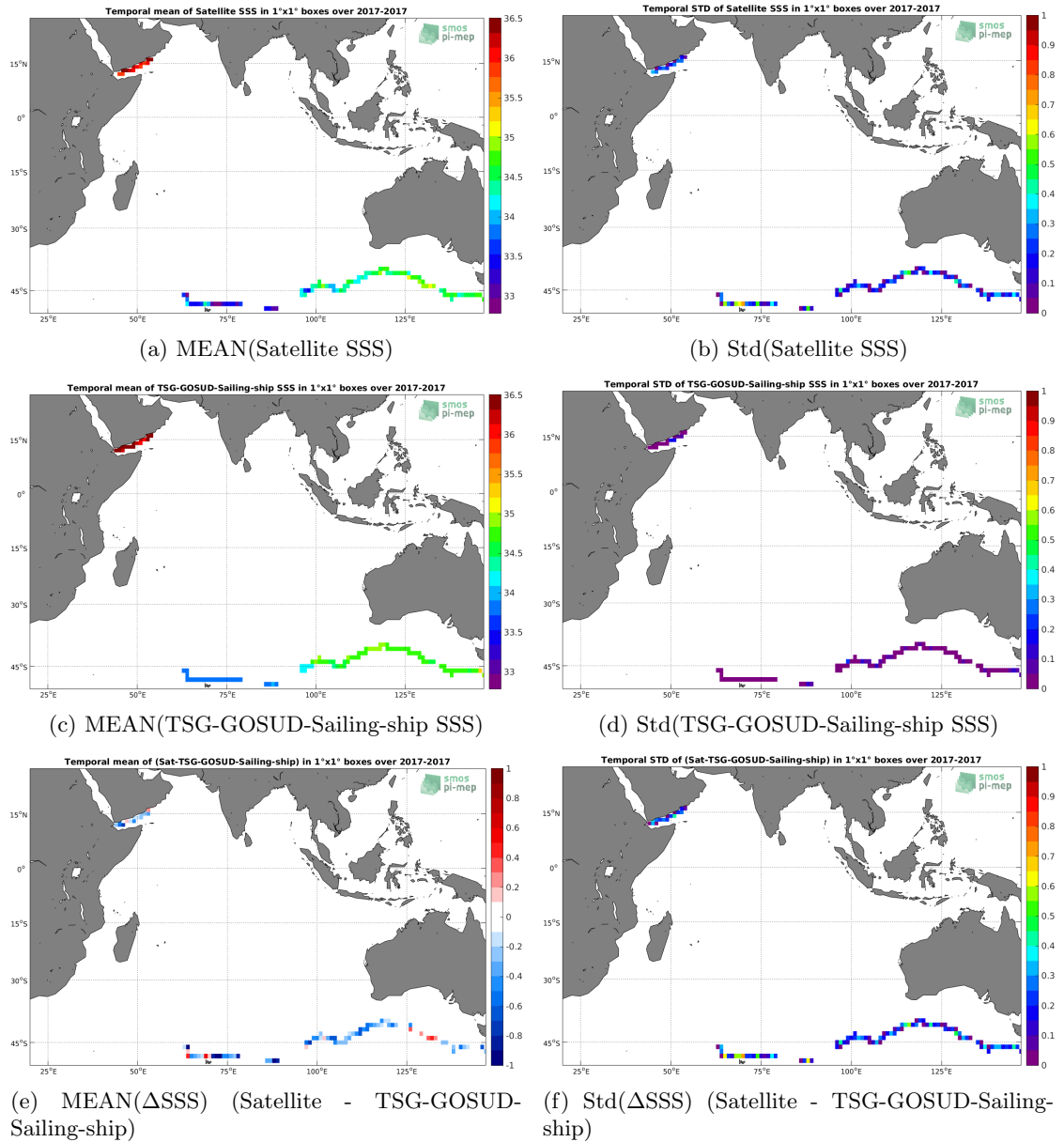
Figure 6: Temporal mean (left) and Std (right) of SSS from SMAP-L3-RSS-V3-8DAY-RUNNING-40KM (top), TSG-GOSUD-Sailing-ship (middle), and of \Delta SSS (Satellite - TSG-GOSUD-Sailing-ship). Only match-up pairs are used to generate these maps.
