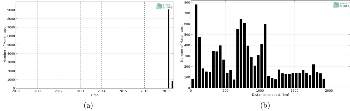
Figure 1: Number of match-ups between TSG-GOSUD-Sailing-ship and SMAP-L3-RSS-V3-8DAY-RUNNING-40KM SSS as a function of time (a) and as function of the distance to coast (b) over the Indian Ocean Pi-MEP region and for the full satellite product period.
