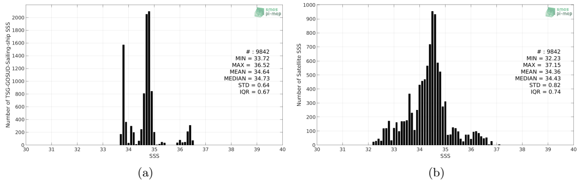
Figure 2: Histograms of SSS from TSG-GOSUD-Sailing-ship (a) and SMAP-L3-RSS-V3-8DAY-RUNNING-40KM (b) considering all match-up pairs per bins of 0.1 over the Indian Ocean Pi-MEP region and for the full satellite product period.
