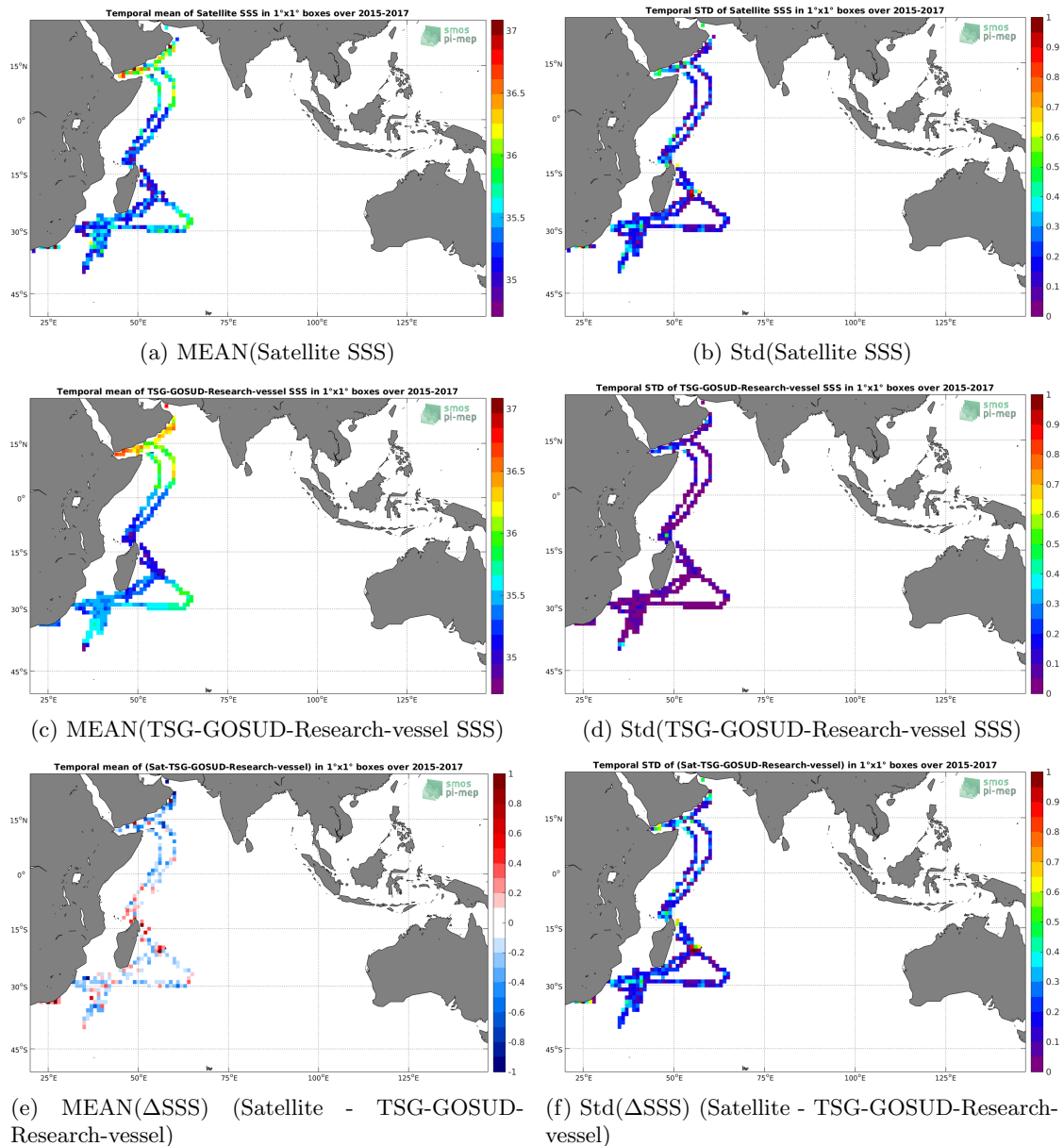
Figure 6: Temporal mean (left) and Std (right) of SSS from SMAP-L3-RSS-V3-8DAY-RUNNING-40KM (top), TSG-GOSUD-Research-vessel (middle), and of \Delta SSS (Satellite - TSG-GOSUD-Research-vessel). Only match-up pairs are used to generate these maps.
