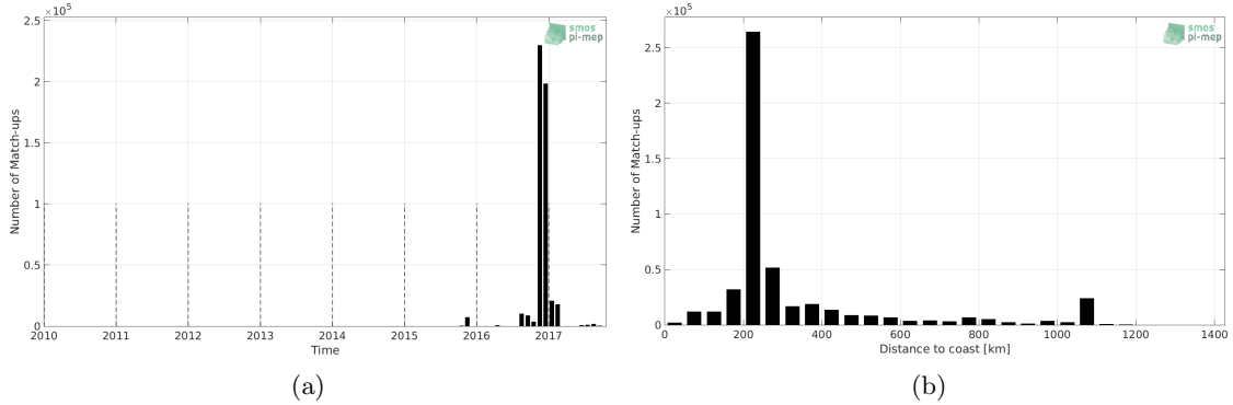
Figure 1: Number of match-ups between TSG-GOSUD-Research-vessel and SMAP-L3-RSS-V3-8DAY-RUNNING-40KM SSS as a function of time (a) and as function of the distance to coast (b) over the Indian Ocean Pi-MEP region and for the full satellite product period.
