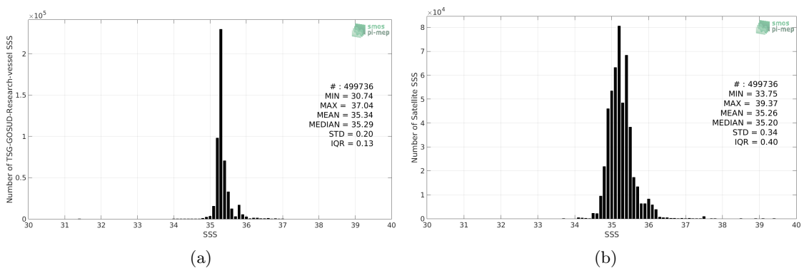
Figure 2: Histograms of SSS from TSG-GOSUD-Research-vessel (a) and SMAP-L3-RSS-V3-8DAY-RUNNING-40KM (b) considering all match-up pairs per bins of 0.1 over the Indian Ocean Pi-MEP region and for the full satellite product period.
