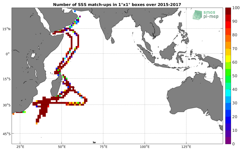
Figure 4: Number of SSS match-ups between TSG-GOSUD-Research-vessel SSS and the SMAP-L3-RSS-V3-8DAY-RUNNING-40KM SSS product for the Indian Ocean Pi-MEP region over 1^\circ \times 1^\circ boxes and for the full satellite product period.
