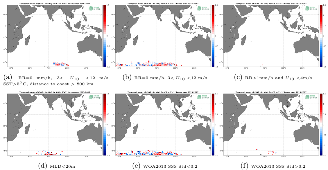
Figure 12: Temporal mean gridded over spatial boxes of size 1^\circ \times 1^\circ of \Delta SSS (SMAP-L3-RSS-V3-8DAY-RUNNING-40KM - Sea mammals) for 6 different subdatasets corresponding to:RR=0 mm/h, 3 < U_{10} < 12 m/s, SST >5^\circ C, distance to coast > 800 km (a), RR=0 mm/h, 3 < U_{10} < 12 m/s (b), RR >1 mm/h and U_{10} < 4 m/s (c),MLD <20 m (d),WOA2013 SSS Std <0.2 (e),WOA2013 SSS Std >0.2 (f).
