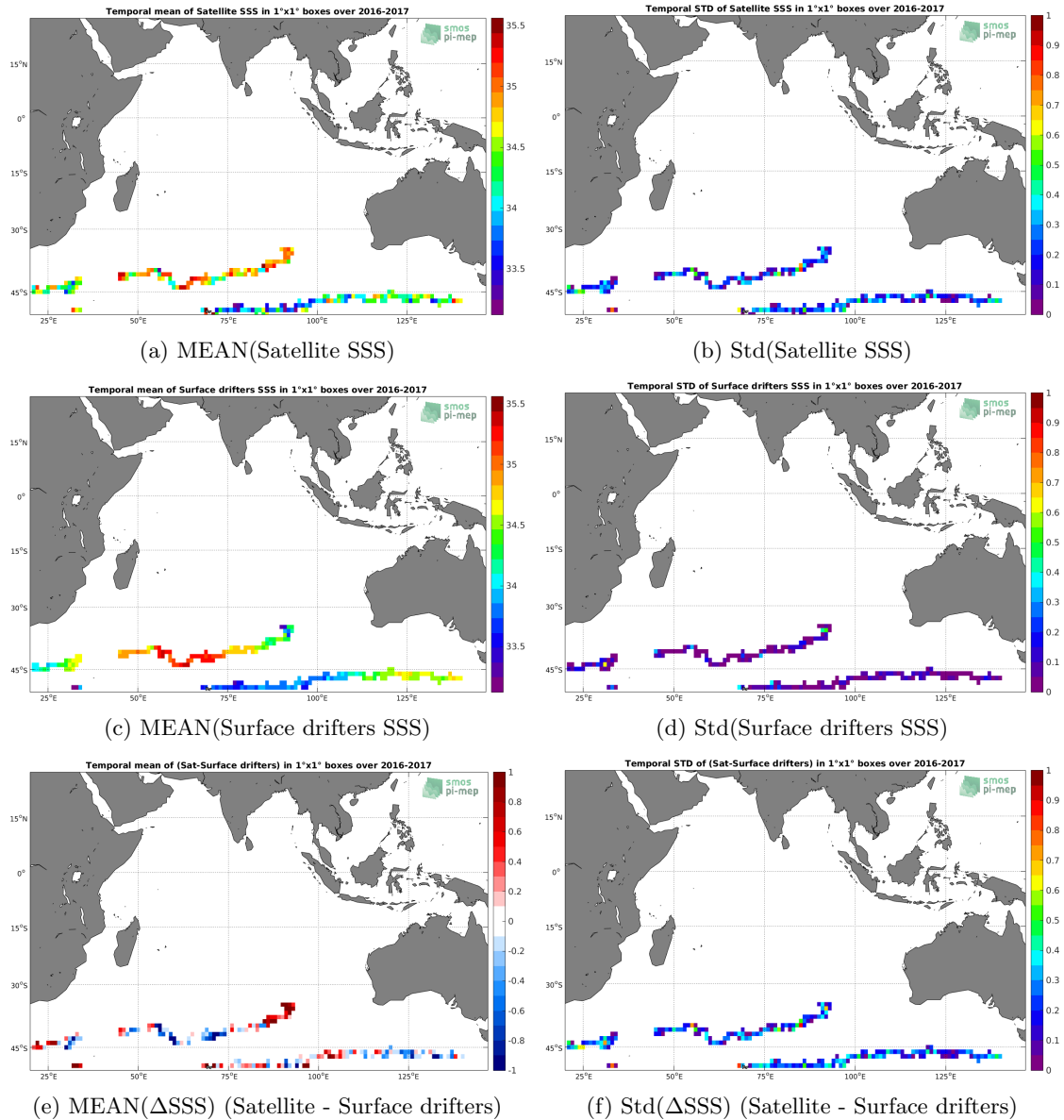
Figure 5: Temporal mean (left) and Std (right) of SSS from SMAP-L3-RSS-V3-8DAY-RUNNING-40KM (top), Surface drifters (middle), and of \Delta SSS (Satellite - Surface drifters). Only match-up pairs are used to generate these maps.
