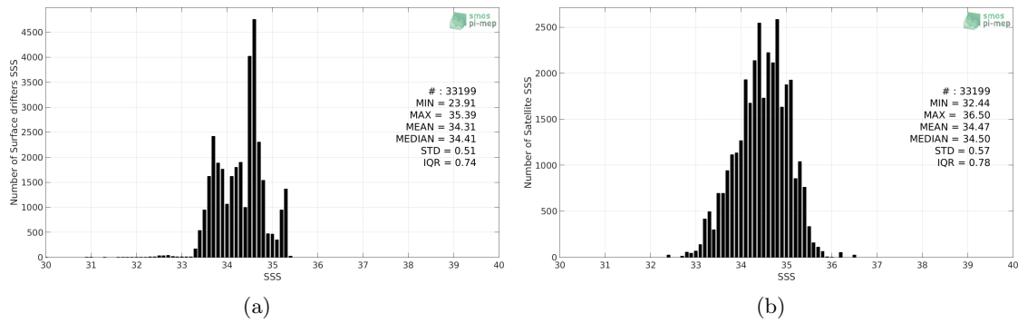
Figure 2: Histograms of SSS from Surface drifters (a) and SMAP-L3-RSS-V3-8DAY-RUNNING-40KM (b) considering all match-up pairs per bins of 0.1 over the Indian Ocean Pi-MEP region and for the full satellite product period.
