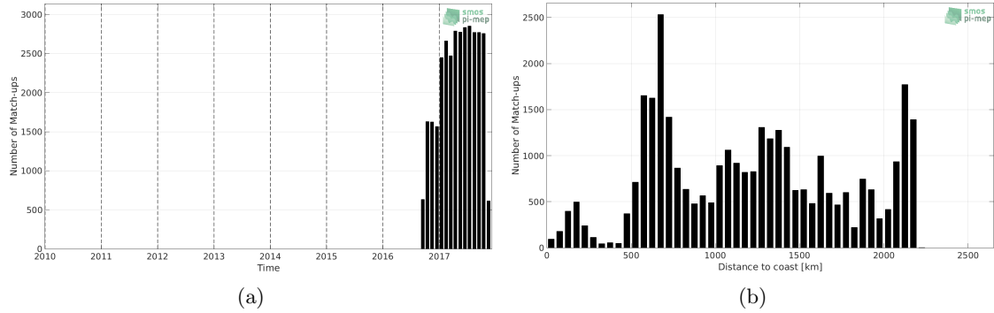
Figure 1: Number of match-ups between Surface drifters and SMAP-L3-RSS-V3-8DAY-RUNNING-40KM SSS as a function of time (a) and as function of the distance to coast (b) over the Indian Ocean Pi-MEP region and for the full satellite product period.
