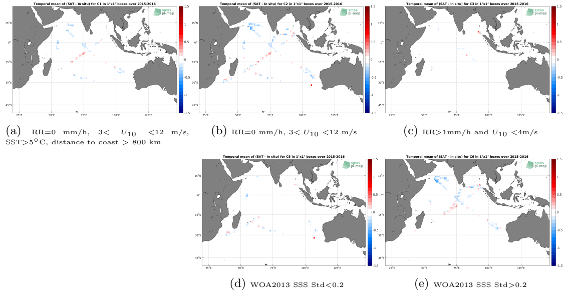
Figure 12: Temporal mean gridded over spatial boxes of size 1^\circ \times 1^\circ of \Delta SSS (SMAP-L3-RSS-V3-MONTHLY-70KM - TSG-LEGOS-DM) for 5 different subdatasets corresponding to: RR=0 mm/h, 3 < U_{10} < 12 m/s, SST >5^\circ\text{C} , distance to coast > 800 km (a), RR=0 mm/h, 3 < U_{10} < 12 m/s (b), RR >1 mm/h and U_{10} < 4 m/s (c), WOA2013 SSS Std <0.2 (d), WOA2013 SSS Std >0.2 (e).
