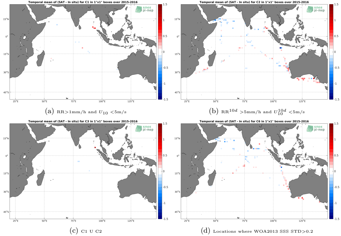
Figure 12: Temporal mean gridded over spatial boxes of size 1^\circ \times 1^\circ of \Delta SSS (SMAP-L3-RSS-V3-MONTHLY-70KM - TSG-LEGOS-DM) for 4 different subdatasets corresponding to: RR > 1\text{mm/h} and U_{10} < 5\text{m/s} (a), RR^{10d} > 5\text{mm/h} and U_{10}^{10d} < 5\text{m/s} (b), C1 U C2 (c), Locations where WOA2013 SSS STD > 0.2 (d).
