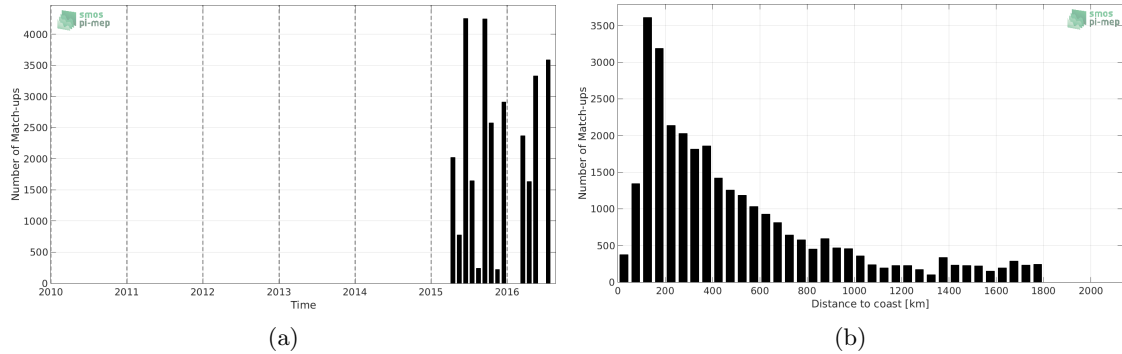
Figure 1: Number of match-ups between TSG-LEGOS-DM and SMAP-L3-RSS-V3-MONTHLY-70KM SSS as a function of time (a) and as function of the distance to coast (b) over the Indian Ocean Pi-MEP region and for the full satellite product period.
