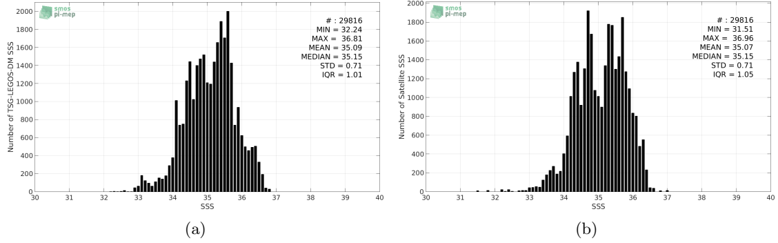
Figure 2: Histograms of SSS from TSG-LEGOS-DM (a) and SMAP-L3-RSS-V3-MONTHLY-70KM (b) considering all match-up pairs per bins of 0.1 over the Indian Ocean Pi-MEP region and for the full satellite product period.
