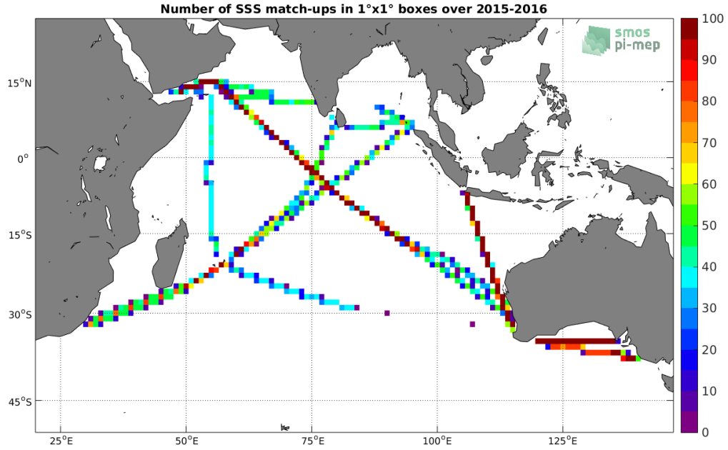
Figure 4: Number of SSS match-ups between TSG-LEGOS-DM SSS and the SMAP-L3-RSS-V3-MONTHLY-70KM SSS product for the Indian Ocean Pi-MEP region over 1^\circ \times 1^\circ boxes and for the full satellite product period.
