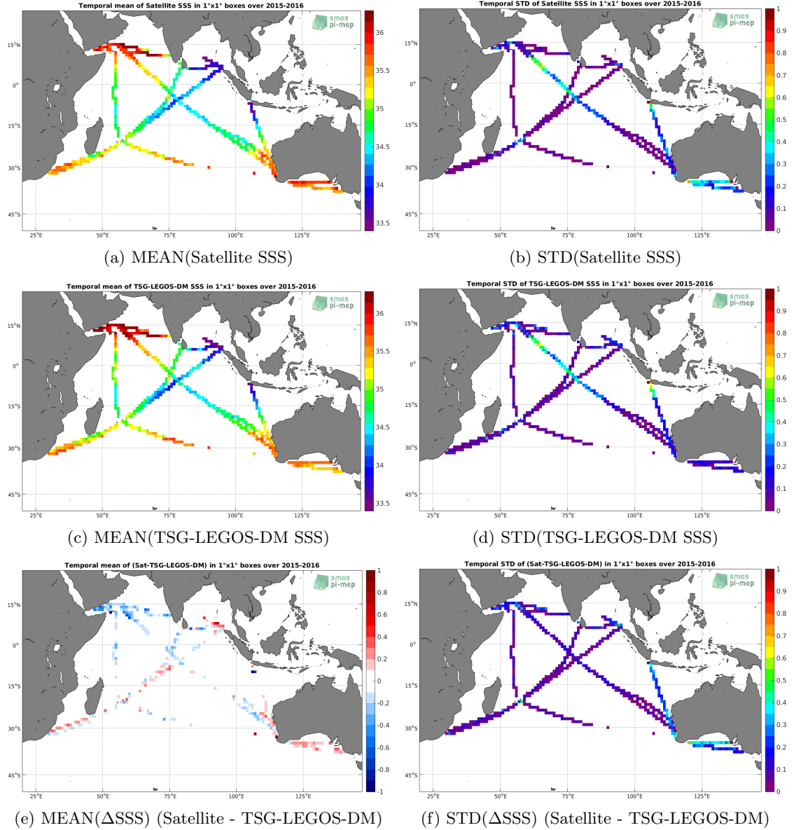
Figure 6: Temporal mean (left) and STD (right) of SSS from SMAP-L3-RSS-V3-MONTHLY-70KM (top), TSG-LEGOS-DM (middle), and of \Delta SSS (Satellite - TSG-LEGOS-DM). Only match-up pairs are used to generate these maps.
