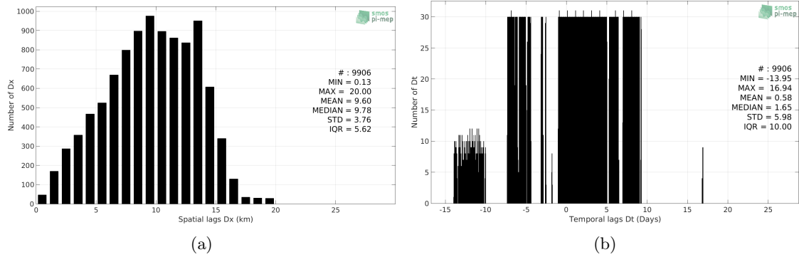
Figure 5: Histograms of the spatial (a) and temporal (b) lags between the time of the TSG-GOSUD-Sailing-ship measurements and the date of the corresponding SMAP-L3-RSS-V3-MONTHLY-0.25DEG-40KM SSS product.
