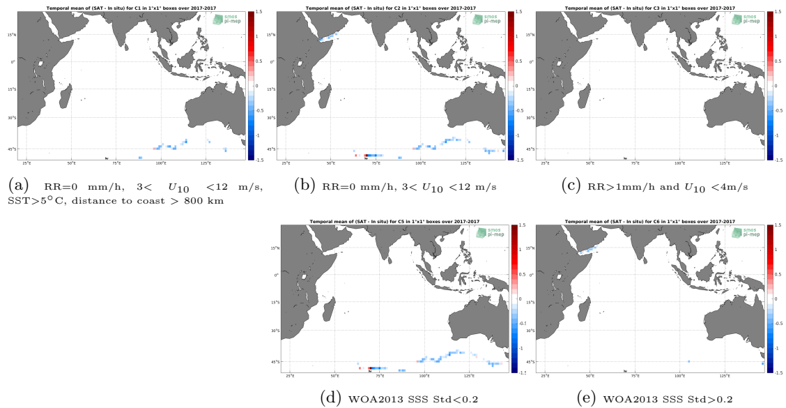
Figure 12: Temporal mean gridded over spatial boxes of size 1^\circ \times 1^\circ of \Delta SSS (SMAP-L3-RSS-V3-MONTHLY-0.25DEG-40KM - TSG-GOSUD-Sailing-ship) for 5 different subdatasets corresponding to:RR=0 mm/h, 3 < U_{10} < 12 m/s, SST >5^\circ C, distance to coast > 800 km (a), RR=0 mm/h, 3 < U_{10} < 12 m/s (b), RR >1 mm/h and U_{10} < 4 m/s (c), WOA2013 SSS Std <0.2 (d), WOA2013 SSS Std >0.2 (e).
