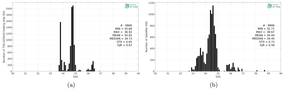
Figure 2: Histograms of SSS from TSG-GOSUD-Sailing-ship (a) and SMAP-L3-RSS-V3-MONTHLY-0.25DEG-40KM (b) considering all match-up pairs per bins of 0.1 over the Indian Ocean Pi-MEP region and for the full satellite product period.
