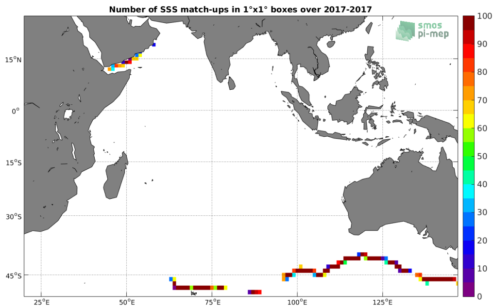
Figure 4: Number of SSS match-ups between TSG-GOSUD-Sailing-ship SSS and the SMAP-L3-RSS-V3-MONTHLY-0.25DEG-40KM SSS product for the Indian Ocean Pi-MEP region over 1^\circ \times 1^\circ boxes and for the full satellite product period.
