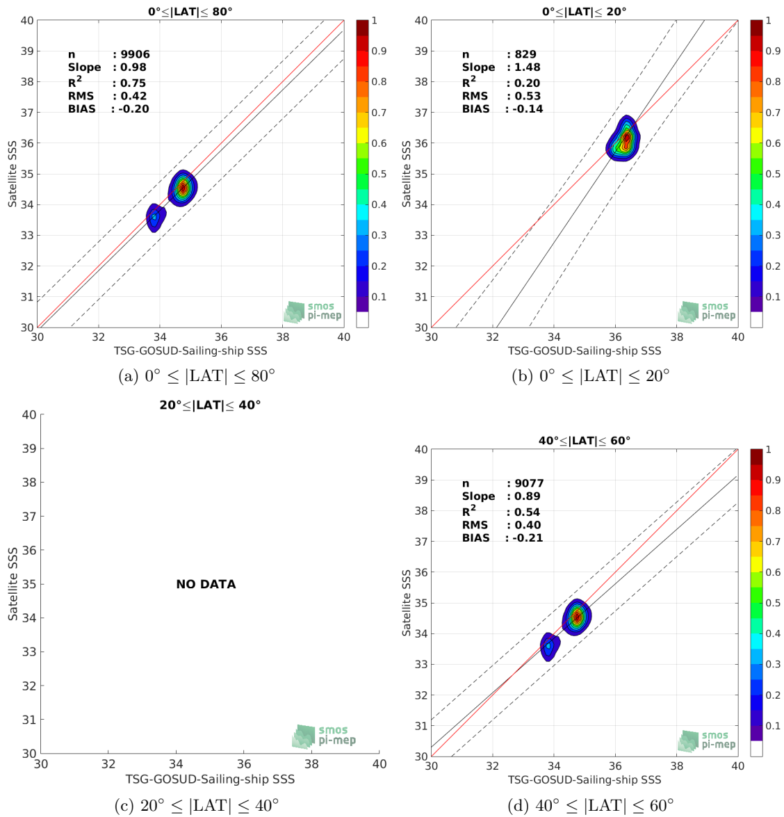
Figure 9: Contour maps of the concentration of SMAP-L3-RSS-V3-MONTHLY-0.25DEG-40KM SSS (y-axis) versus TSG-GOSUD-Sailing-ship SSS (x-axis) at match-up pairs for different latitude bands. For each plot, the red line shows x=y . The black thin and dashed lines indicate a linear fit through the data cloud and the \pm 95\% confidence levels, respectively. The number match-up pairs n , the slope and R^2 coefficient of the linear fit, the root mean square (RMS) and the mean bias between satellite and in situ data are indicated for each latitude band in each plots.
