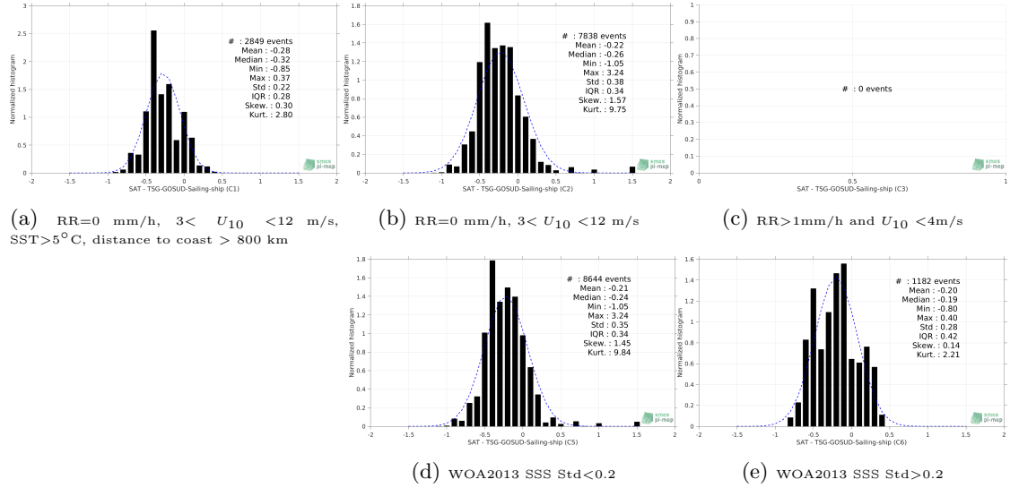
Figure 13: Normalized histogram of \Delta SSS (SMAP-L3-RSS-V3-MONTHLY-0.25DEG-40KM - TSG-GOSUD-Sailing-ship) for 5 different subdatasets corresponding to: RR=0 mm/h, 3 < U_{10} < 12 m/s, SST > 5°C, distance to coast > 800 km (a), RR=0 mm/h, 3 < U_{10} < 12 m/s (b), RR > 1mm/h and U_{10} < 4 m/s (c), WOA2013 SSS Std < 0.2 (d), WOA2013 SSS Std > 0.2 (e).
