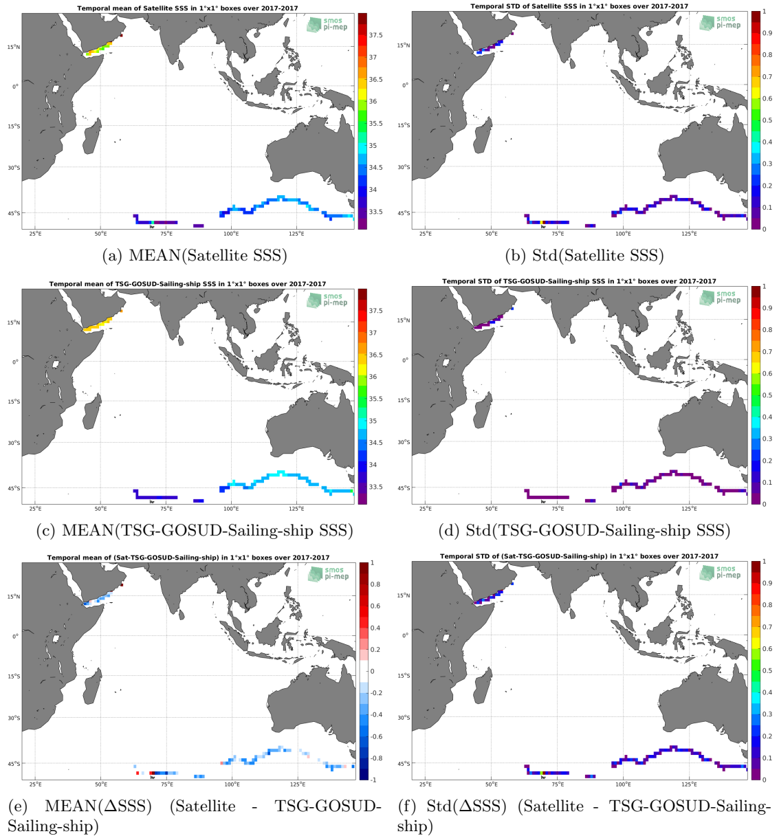
Figure 6: Temporal mean (left) and Std (right) of SSS from SMAP-L3-RSS-V3-MONTHLY-0.25DEG-40KM (top), TSG-GOSUD-Sailing-ship (middle), and of \Delta SSS (Satellite - TSG-GOSUD-Sailing-ship). Only match-up pairs are used to generate these maps.
