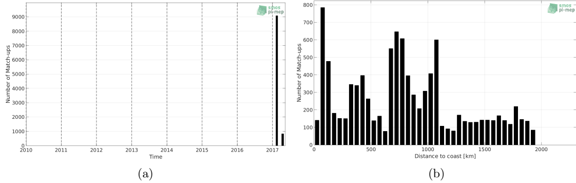
Figure 1: Number of match-ups between TSG-GOSUD-Sailing-ship and SMAP-L3-RSS-V3-MONTHLY-0.25DEG-40KM SSS as a function of time (a) and as function of the distance to coast (b) over the Indian Ocean Pi-MEP region and for the full satellite product period.
