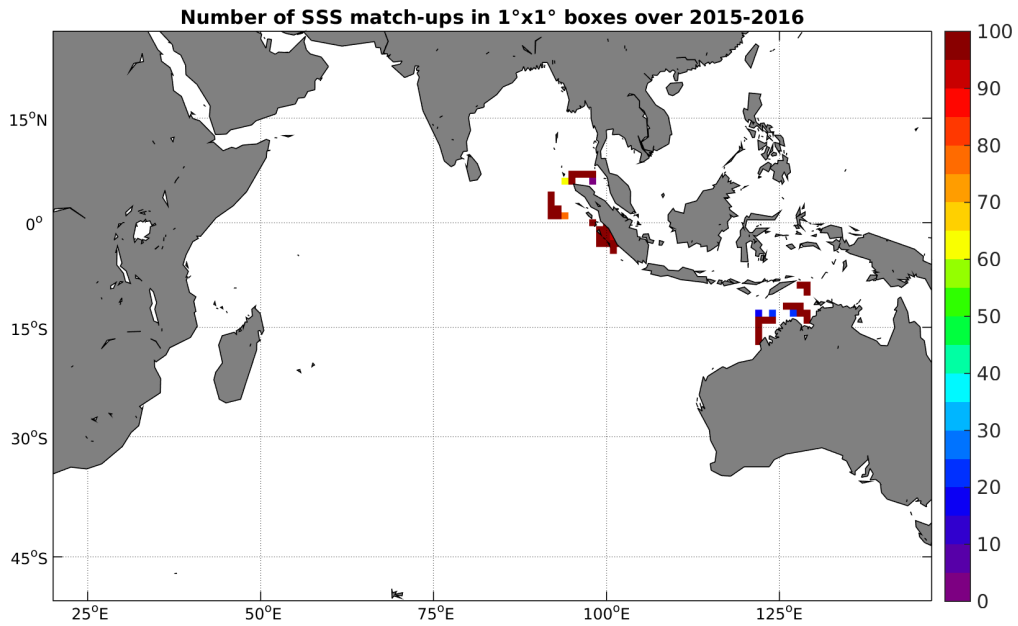
Figure 4: Number of SSS match-ups between TSG-SAMOS SSS and the SMAP-L3-RSS-V2-8DAY-RUNNING-40KM SSS product for the Indian Ocean Pi-MEP region over 1^\circ \times 1^\circ boxes and for the full satellite product period.
