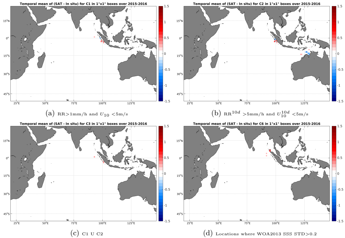
Figure 12: Temporal mean gridded over spatial boxes of size 1^\circ \times 1^\circ of \Delta SSS (SMAP-L3-RSS-V2-8DAY-RUNNING-40KM - TSG-SAMOS) for 4 different subdatasets corresponding to: RR > 1\text{mm/h} and U_{10} < 5\text{m/s} (a), RR^{10d} > 5\text{mm/h} and U_{10}^{10d} < 5\text{m/s} (b), C1 \cup C2 (c), Locations where WOA2013 SSS STD > 0.2 (d).
