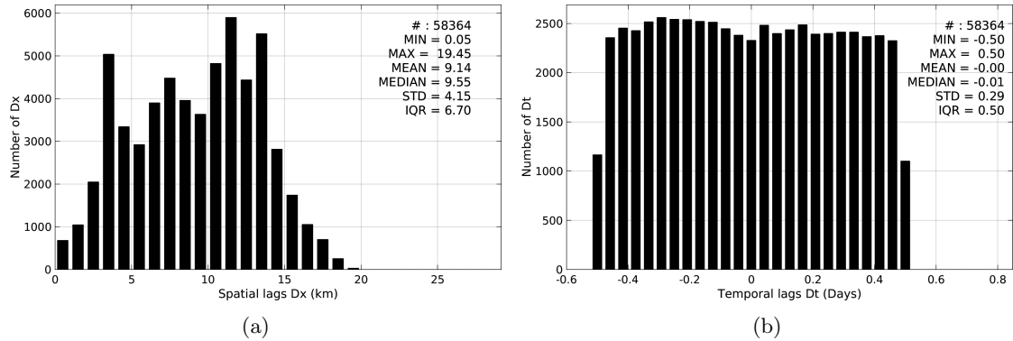
Figure 5: Histograms of the spatial (a) and temporal (b) lags between the time of the TSG-SAMOS measurements and the date of the corresponding SMAP-L3-RSS-V2-8DAY-RUNNING-40KM SSS product.
