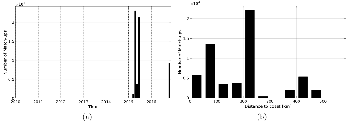
Figure 1: Number of match-ups between TSG-SAMOS and SMAP-L3-RSS-V2-8DAY-RUNNING-40KM SSS as a function of time (a) and as function of the distance to coast (b) over the Indian Ocean Pi-MEP region and for the full satellite product period.
