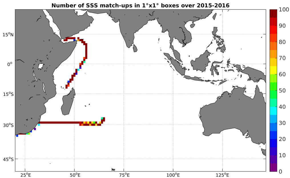
Figure 4: Number of SSS match-ups between TSG-GOSUD-Research-vessel SSS and the SMAP-L3-RSS-V2-8DAY-RUNNING-40KM SSS product for the Indian Ocean Pi-MEP region over 1^\circ \times 1^\circ boxes and for the full satellite product period.
