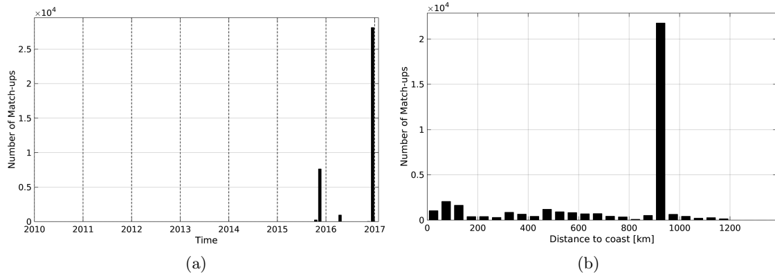
Figure 1: Number of match-ups between TSG-GOSUD-Research-vessel and SMAP-L3-RSS-V2-8DAY-RUNNING-40KM SSS as a function of time (a) and as function of the distance to coast (b) over the Indian Ocean Pi-MEP region and for the full satellite product period.
