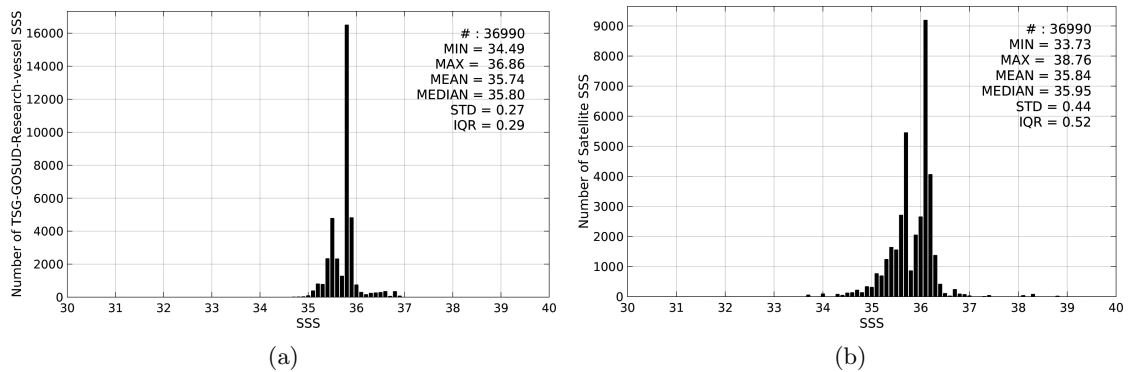
Figure 2: Histograms of SSS from TSG-GOSUD-Research-vessel (a) and SMAP-L3-RSS-V2-8DAY-RUNNING-40KM (b) considering all match-up pairs per bins of 0.1 over the Indian Ocean Pi-MEP region and for the full satellite product period.
