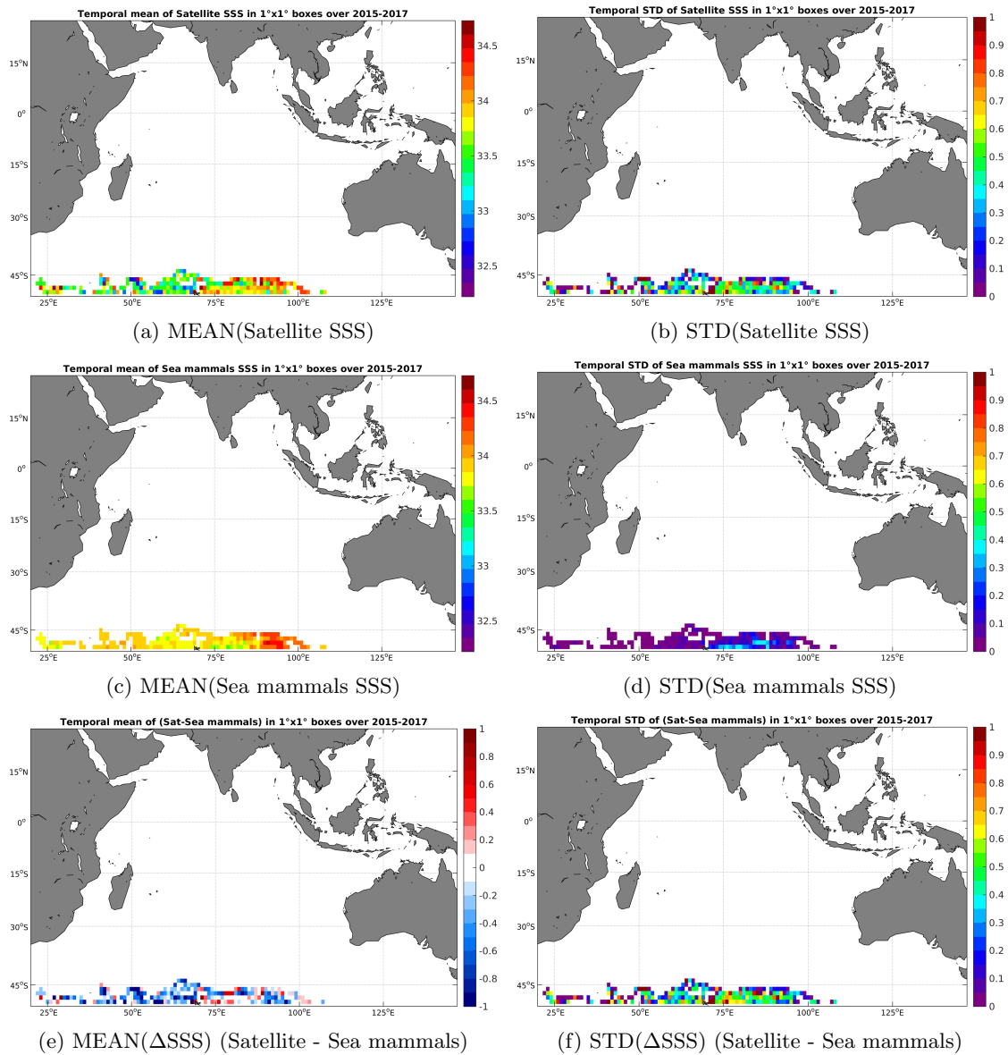
Figure 6: Temporal mean (left) and STD (right) of SSS from SMAP-L3-RSS-V2-8DAY-RUNNING-40KM (top), Sea mammals (middle), and of \Delta SSS (Satellite - Sea mammals). Only match-up pairs are used to generate these maps.
