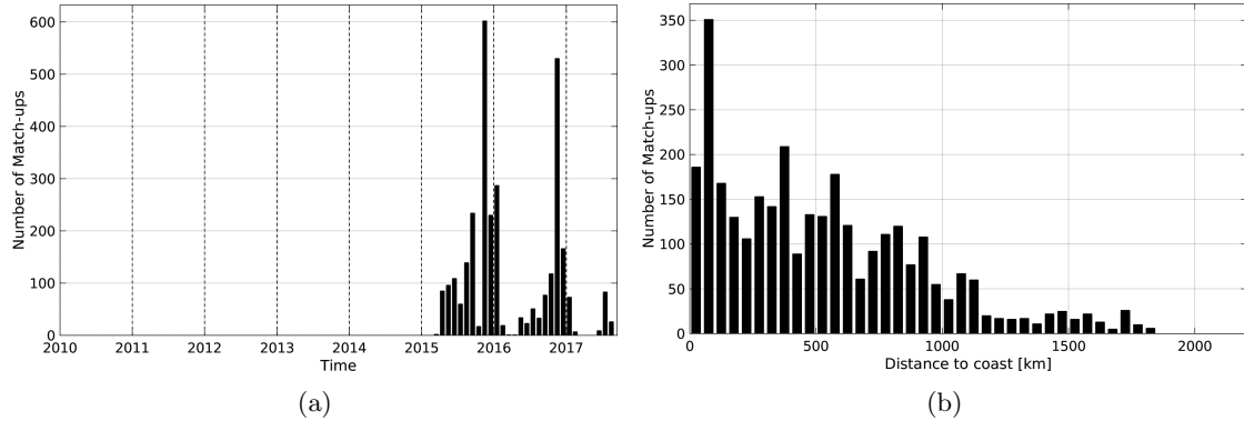
Figure 1: Number of match-ups between Sea mammals and SMAP-L3-RSS-V2-8DAY-RUNNING-40KM SSS as a function of time (a) and as function of the distance to coast (b) over the Indian Ocean Pi-MEP region and for the full satellite product period.
