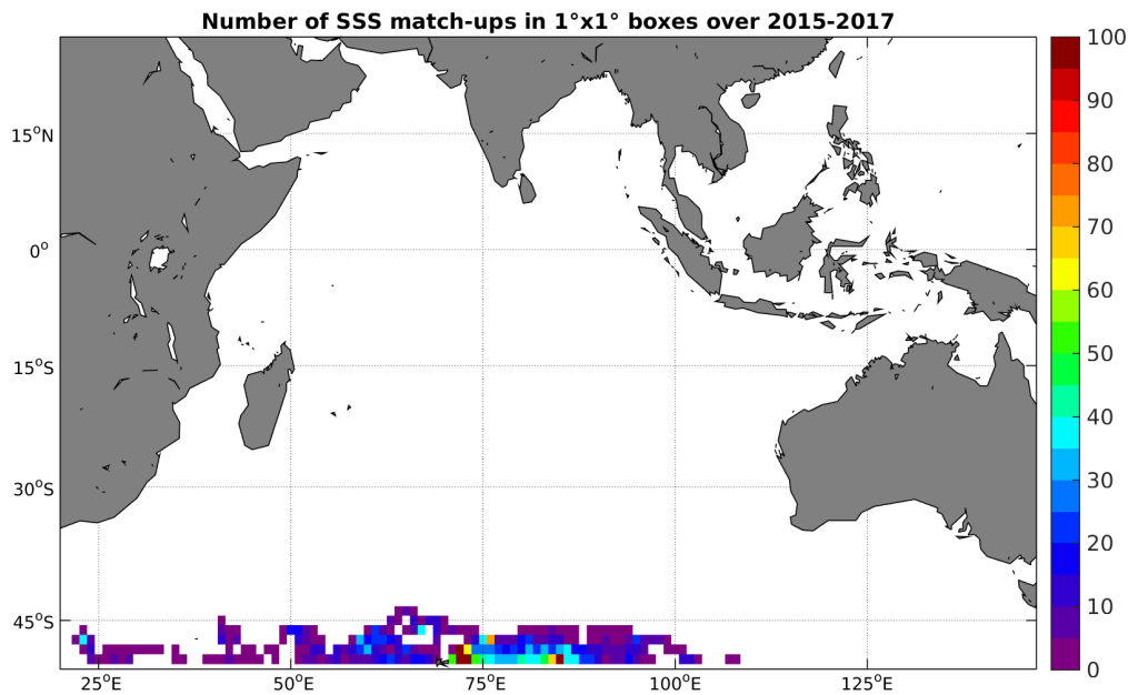
Figure 4: Number of SSS match-ups between Sea mammals SSS and the SMAP-L3-RSS-V2-8DAY-RUNNING-40KM SSS product for the Indian Ocean Pi-MEP region over 1^\circ \times 1^\circ boxes and for the full satellite product period.
