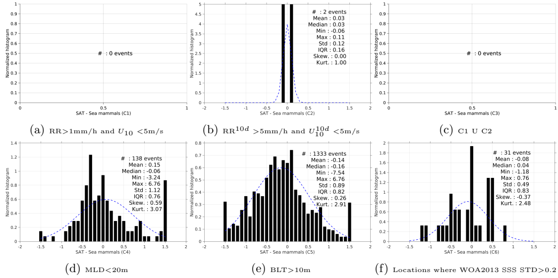
Figure 13: Normalized histogram of \Delta SSS (SMAP-L3-RSS-V2-8DAY-RUNNING-40KM - Sea mammals) for 6 different subdatasets corresponding to: RR>1mm/h and U_{10} < 5\text{m/s} (a), RR^{10d} > 5\text{mm/h} and U_{10}^{10d} < 5\text{m/s} (b), C1 U C2 (c), MLD<20m (d), BLT>10m (e), Locations where WOA2013 SSS STD>0.2 (f).
