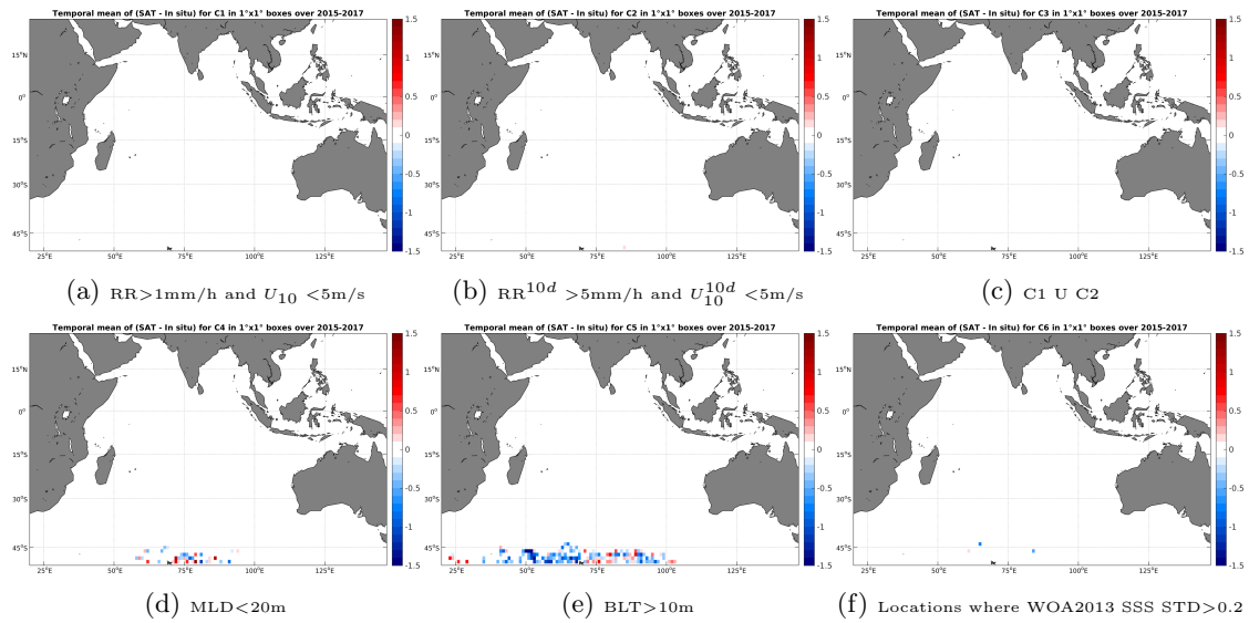
Figure 12: Temporal mean gridded over spatial boxes of size 1^\circ \times 1^\circ of \Delta SSS (SMAP-L3-RSS-V2-8DAY-RUNNING-40KM - Sea mammals) for 6 different subdatasets corresponding to:RR>1mm/h and U_{10} < 5m/s (a), RR^{10d} > 5mm/h and U_{10}^{10d} < 5m/s (b), C1 U C2 (c),MLD<20m (d),BLT>10m (e),Locations where WOA2013 SSS STD>0.2 (f).
