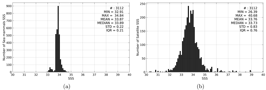
Figure 2: Histograms of SSS from Sea mammals (a) and SMAP-L3-RSS-V2-8DAY-RUNNING-40KM (b) considering all match-up pairs per bins of 0.1 over the Indian Ocean Pi-MEP region and for the full satellite product period.
