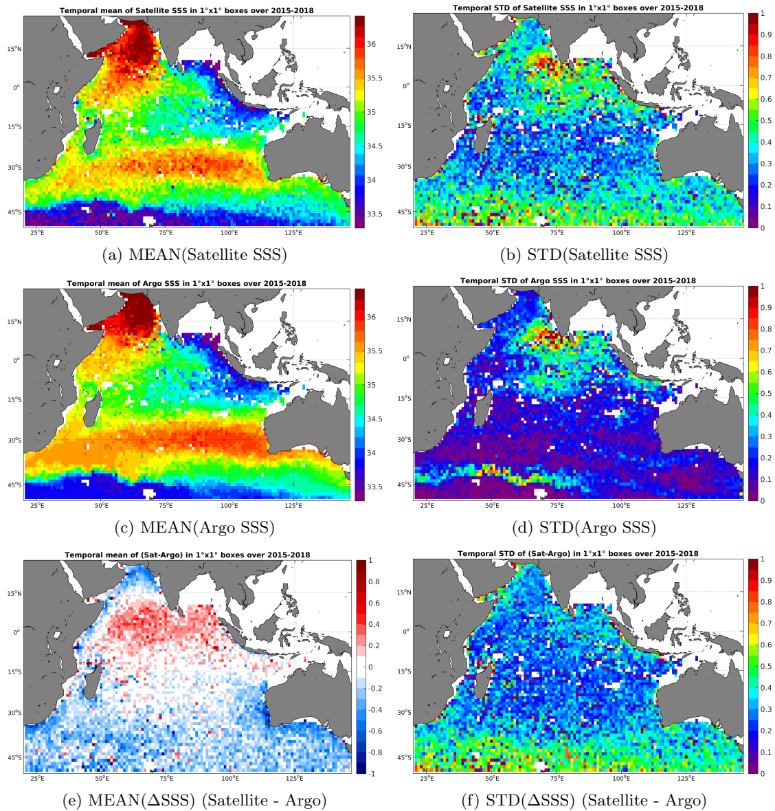
Figure 6: Temporal mean (left) and STD (right) of SSS from SMAP-L3-RSS-V2-8DAY-RUNNING-40KM (top), Argo (middle), and of \Delta SSS (Satellite - Argo). Only match-up pairs are used to generate these maps.
