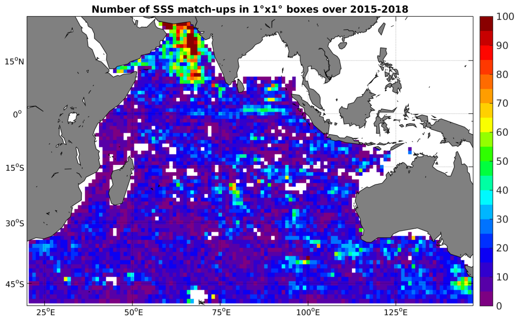
Figure 4: Number of SSS match-ups between Argo SSS and the SMAP-L3-RSS-V2-8DAY-RUNNING-40KM SSS product for the Indian Ocean Pi-MEP region over 1^{\circ} \times 1^{\circ} boxes and for the full satellite product period.
