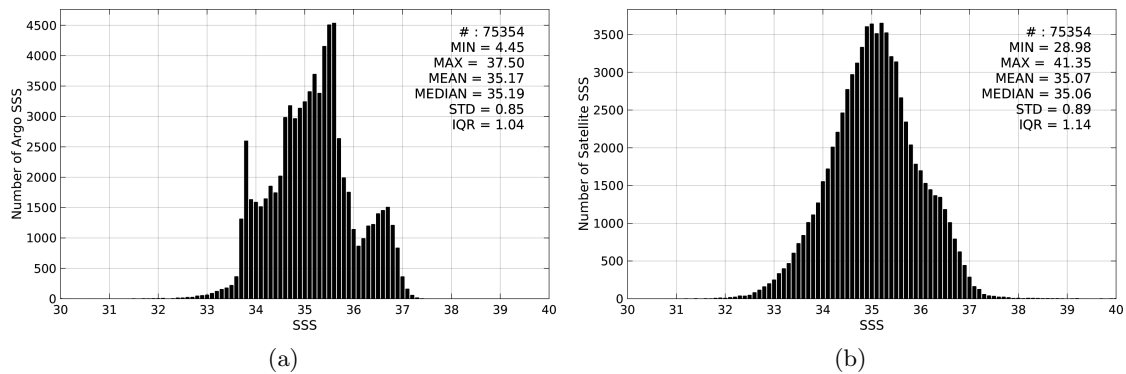
Figure 2: Histograms of SSS from Argo (a) and SMAP-L3-RSS-V2-8DAY-RUNNING-40KM (b) considering all match-up pairs per bins of 0.1 over the Indian Ocean Pi-MEP region and for the full satellite product period.
