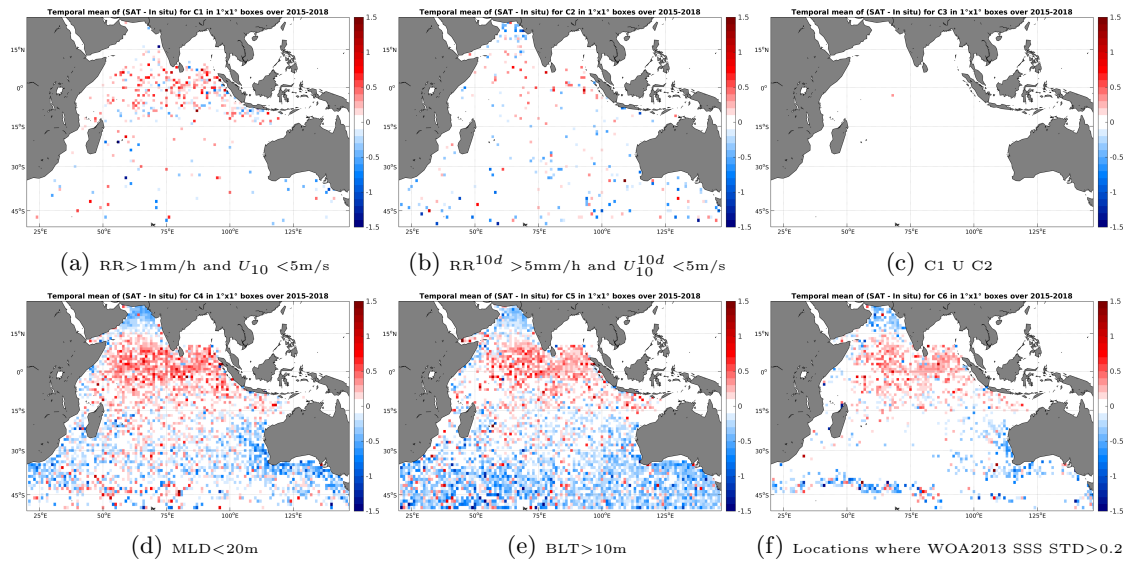
Figure 12: Temporal mean gridded over spatial boxes of size 1^\circ \times 1^\circ of \Delta SSS (SMAP-L3-RSS-V2-8DAY-RUNNING-40KM - Argo) for 6 different subdatasets corresponding to: RR > 1\text{mm/h} and U_{10} < 5\text{m/s} (a), RR^{10d} > 5\text{mm/h} and U_{10}^{10d} < 5\text{m/s} (b), C1 U C2 (c), MLD < 20\text{m} (d), BLT > 10\text{m} (e), Locations where WOA2013 SSS STD > 0.2 (f).
