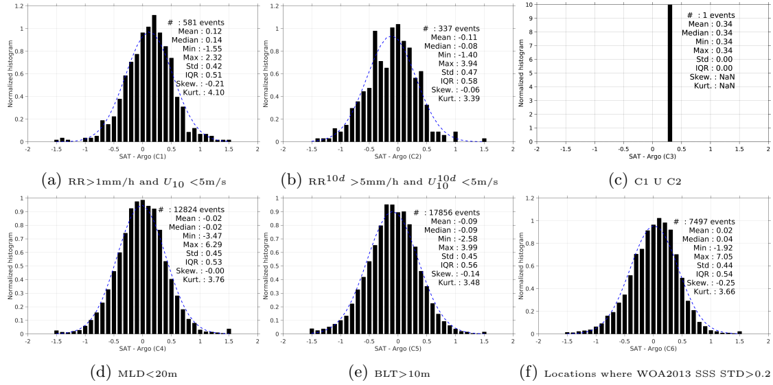
Figure 13: Normalized histogram of \Delta SSS (SMAP-L3-RSS-V2-8DAY-RUNNING-40KM - Argo) for 6 different subdatasets corresponding to: RR>1mm/h and U_{10} < 5\text{m/s} (a), RR 10d >5mm/h and U_{10}^{10d} < 5\text{m/s} (b), C1 U C2 (c),MLD<20m (d),BLT>10m (e),Locations where WOA2013 SSS STD>0.2 (f).
