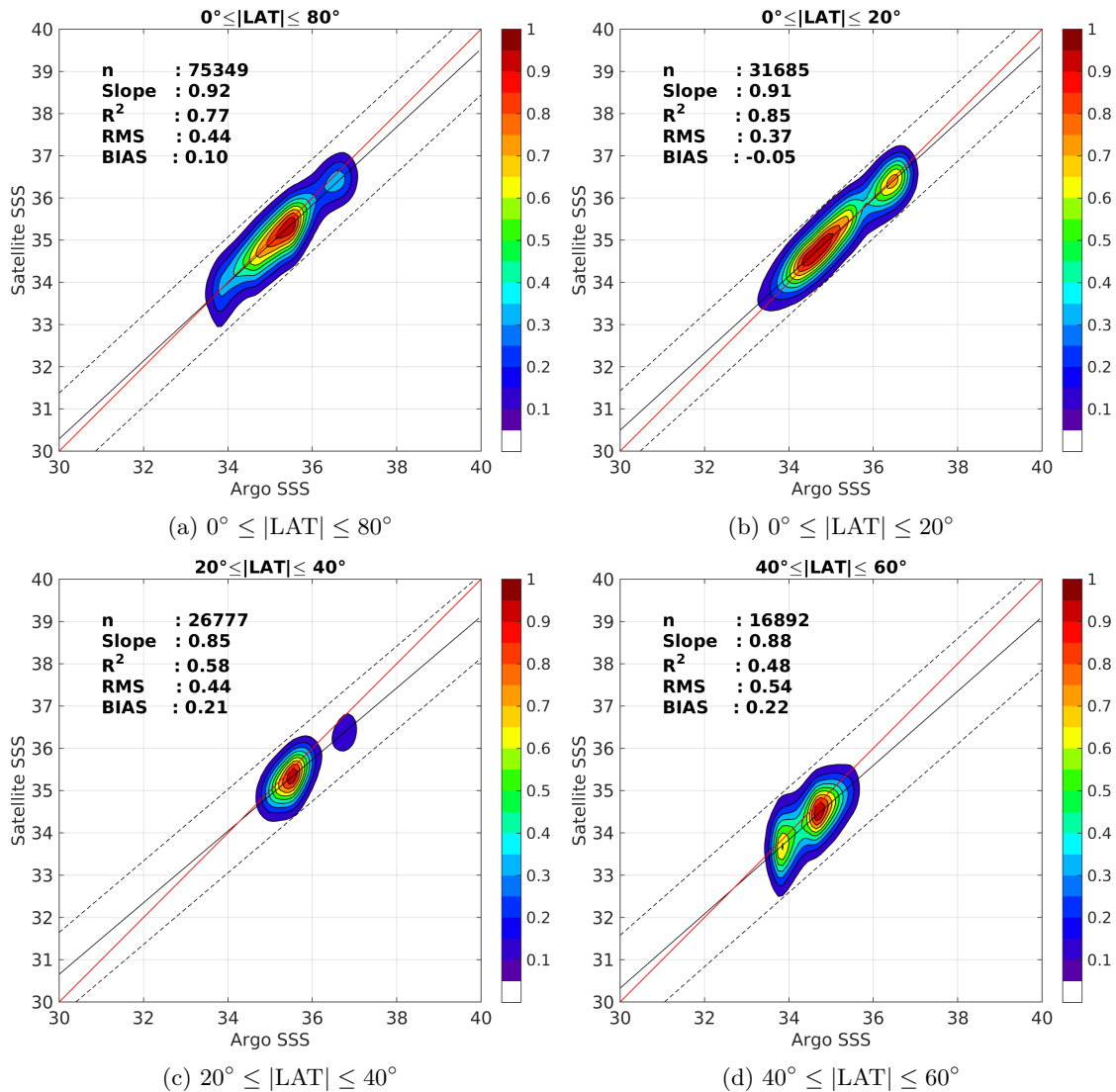
Figure 9: Contour maps of the concentration of SMAP-L3-RSS-V2-8DAY-RUNNING-40KM SSS (y-axis) versus Argo SSS (x-axis) at match-up pairs for different latitude bands. For each plot, the red line shows x=y . The black thin and dashed lines indicate a linear fit through the data cloud and the \pm 95\% confidence levels, respectively. The number match-up pairs n , the slope and R^2 coefficient of the linear fit, the root mean square (RMS) and the mean bias between satellite and in situ data are indicated for each latitude band in each plots.
