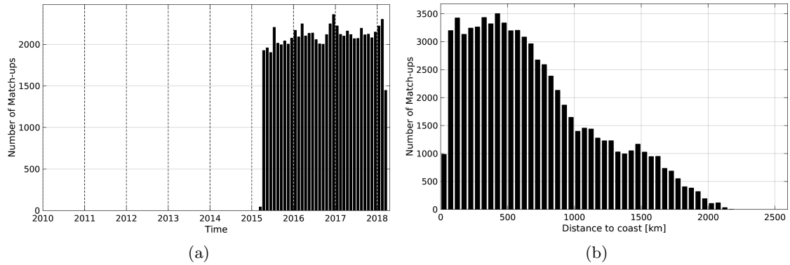
Figure 1: Number of match-ups between Argo and SMAP-L3-RSS-V2-8DAY-RUNNING-40KM SSS as a function of time (a) and as function of the distance to coast (b) over the Indian Ocean Pi-MEP region and for the full satellite product period.
