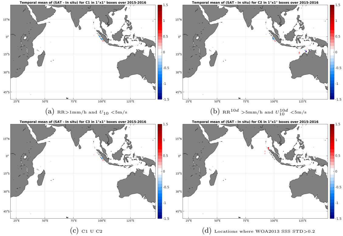
Figure 12: Temporal mean gridded over spatial boxes of size 1^\circ \times 1^\circ of \Delta SSS (SMAP-L3-RSS-V2-8DAY-RUNNING-70KM - TSG-SAMOS) for 4 different subdatasets corresponding to: RR > 1 mm/h and U_{10} < 5 m/s (a), RR^{10d} > 5 mm/h and U_{10}^{10d} < 5 m/s (b), C1 U C2 (c), Locations where WOA2013 SSS STD > 0.2 (d).
