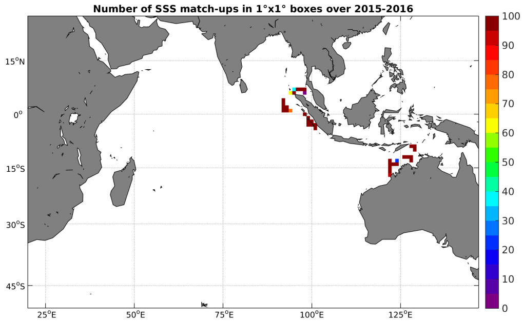
Figure 4: Number of SSS match-ups between TSG-SAMOS SSS and the SMAP-L3-RSS-V2-8DAY-RUNNING-70KM SSS product for the Indian Ocean Pi-MEP region over 1^\circ \times 1^\circ boxes and for the full satellite product period.
