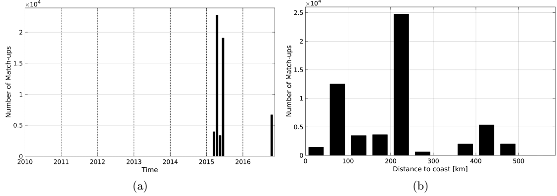
Figure 1: Number of match-ups between TSG-SAMOS and SMAP-L3-RSS-V2-8DAY-RUNNING-70KM SSS as a function of time (a) and as function of the distance to coast (b) over the Indian Ocean Pi-MEP region and for the full satellite product period.
