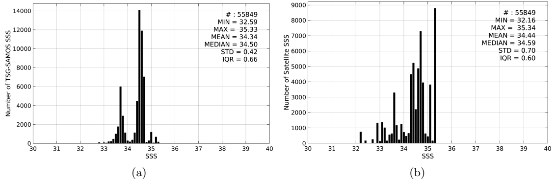
Figure 2: Histograms of SSS from TSG-SAMOS (a) and SMAP-L3-RSS-V2-8DAY-RUNNING-70KM (b) considering all match-up pairs per bins of 0.1 over the Indian Ocean Pi-MEP region and for the full satellite product period.
