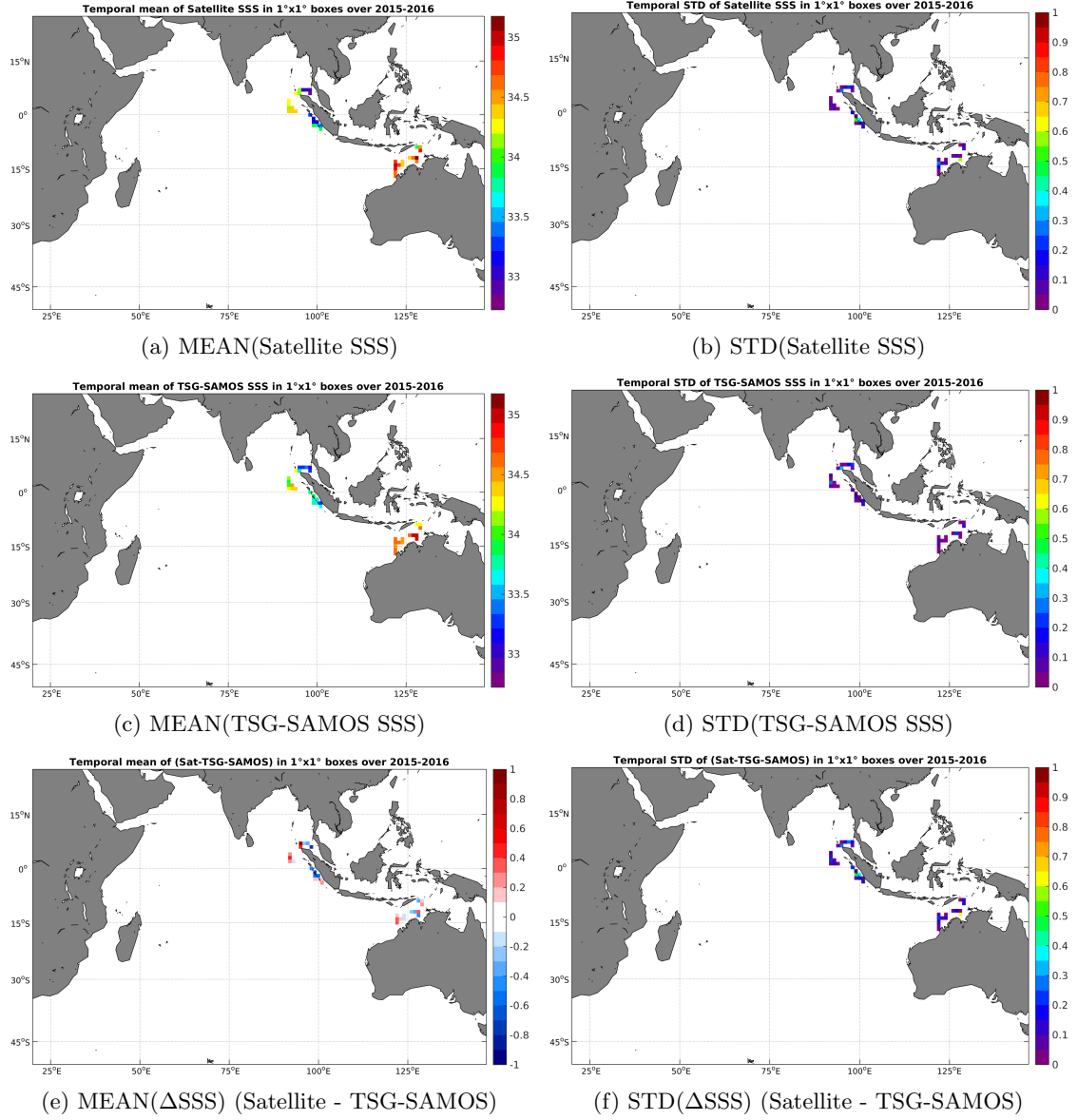
Figure 6: Temporal mean (left) and STD (right) of SSS from SMAP-L3-RSS-V2-8DAY-RUNNING-70KM (top), TSG-SAMOS (middle), and of \Delta SSS (Satellite - TSG-SAMOS). Only match-up pairs are used to generate these maps.
