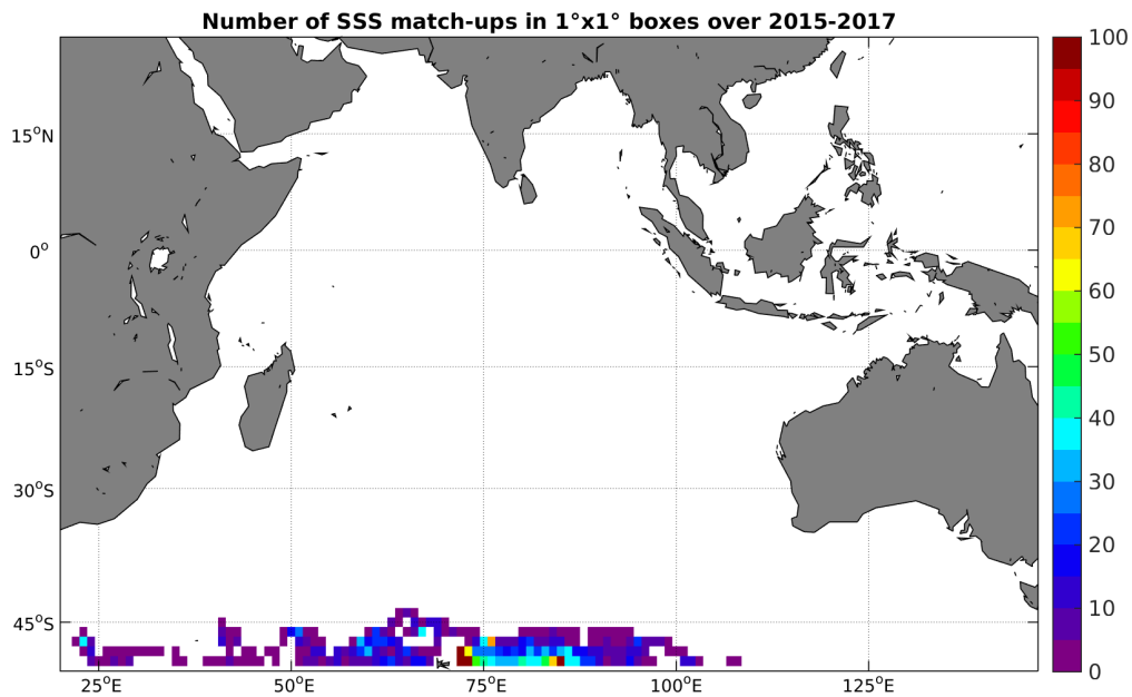
Figure 4: Number of SSS match-ups between Sea mammals SSS and the SMAP-L3-RSS-V2-8DAY-RUNNING-70KM SSS product for the Indian Ocean Pi-MEP region over 1^\circ \times 1^\circ boxes and for the full satellite product period.
