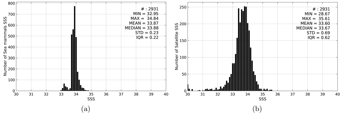
Figure 2: Histograms of SSS from Sea mammals (a) and SMAP-L3-RSS-V2-8DAY-RUNNING-70KM (b) considering all match-up pairs per bins of 0.1 over the Indian Ocean Pi-MEP region and for the full satellite product period.
