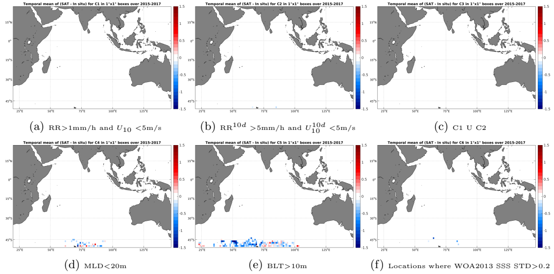
Figure 12: Temporal mean gridded over spatial boxes of size 1^\circ \times 1^\circ of \Delta SSS (SMAP-L3-RSS-V2-8DAY-RUNNING-70KM - Sea mammals) for 6 different subdatasets corresponding to: RR > 1mm/h and U_{10} < 5 m/s (a), RR^{10d} > 5 mm/h and U_{10}^{10d} < 5 m/s (b), C1 U C2 (c), MLD < 20m (d), BLT > 10m (e), Locations where WOA2013 SSS STD > 0.2 (f).
