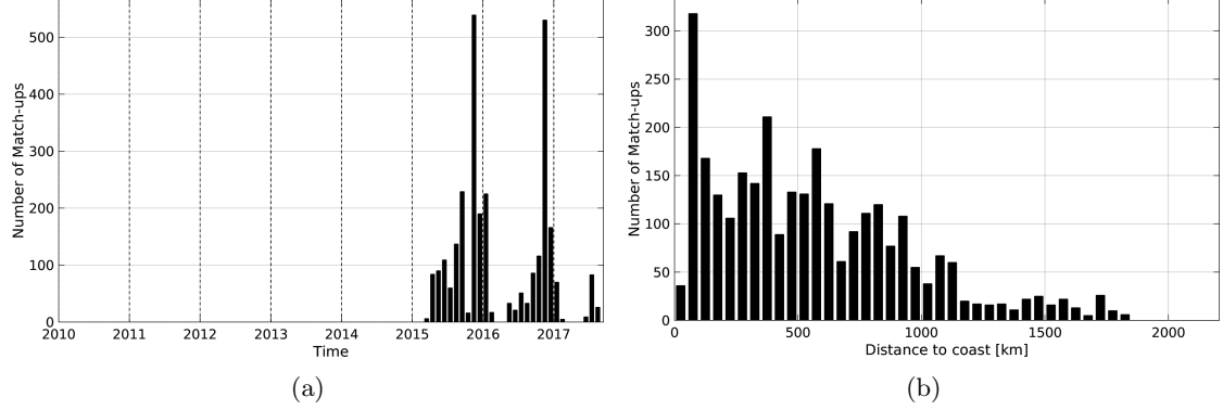
Figure 1: Number of match-ups between Sea mammals and SMAP-L3-RSS-V2-8DAY-RUNNING-70KM SSS as a function of time (a) and as function of the distance to coast (b) over the Indian Ocean Pi-MEP region and for the full satellite product period.
