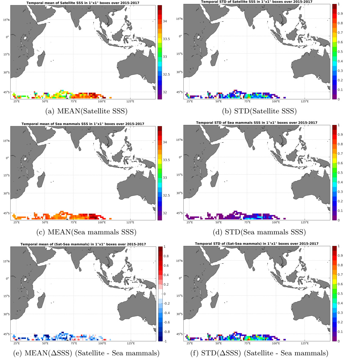
Figure 6: Temporal mean (left) and STD (right) of SSS from SMAP-L3-RSS-V2-8DAY-RUNNING-70KM (top), Sea mammals (middle), and of \Delta SSS (Satellite - Sea mammals). Only match-up pairs are used to generate these maps.
