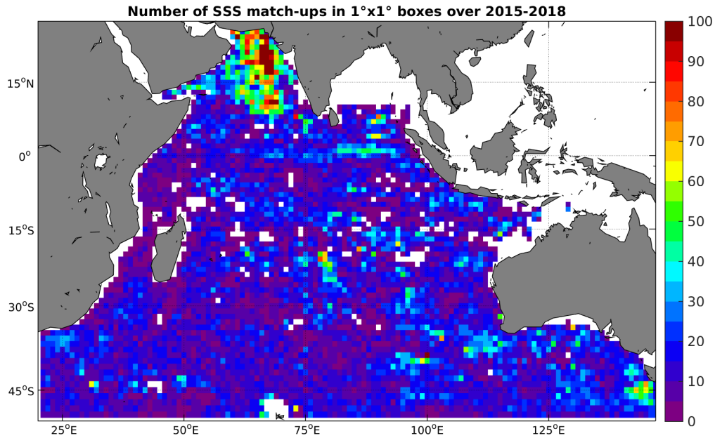
Figure 4: Number of SSS match-ups between Argo SSS and the SMAP-L3-RSS-V2-8DAY-RUNNING-70KM SSS product for the Indian Ocean Pi-MEP region over 1^\circ \times 1^\circ boxes and for the full satellite product period.
