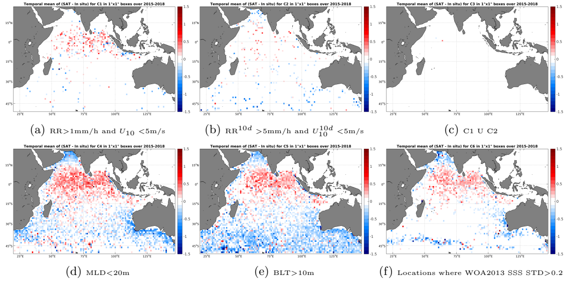
Figure 12: Temporal mean gridded over spatial boxes of size 1^\circ \times 1^\circ of \Delta SSS (SMAP-L3-RSS-V2-8DAY-RUNNING-70KM - Argo) for 6 different subdatasets corresponding to: RR > 1\text{mm/h} and U_{10} < 5\text{m/s} (a), RR^{10d} > 5\text{mm/h} and U_{10}^{10d} < 5\text{m/s} (b), C1 U C2 (c), MLD < 20\text{m} (d), BLT > 10\text{m} (e), Locations where WOA2013 SSS STD > 0.2 (f).
