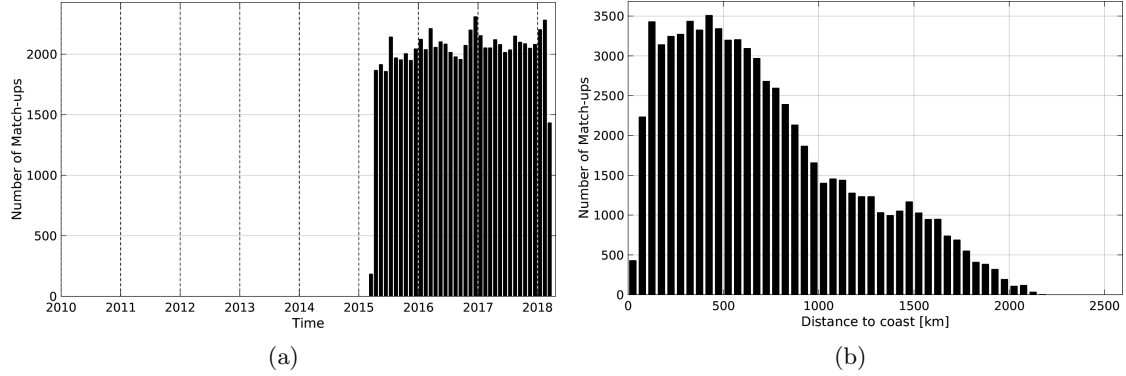
Figure 1: Number of match-ups between Argo and SMAP-L3-RSS-V2-8DAY-RUNNING-70KM SSS as a function of time (a) and as function of the distance to coast (b) over the Indian Ocean Pi-MEP region and for the full satellite product period.
