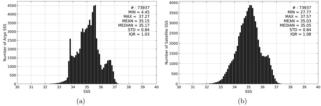
Figure 2: Histograms of SSS from Argo (a) and SMAP-L3-RSS-V2-8DAY-RUNNING-70KM (b) considering all match-up pairs per bins of 0.1 over the Indian Ocean Pi-MEP region and for the full satellite product period.
