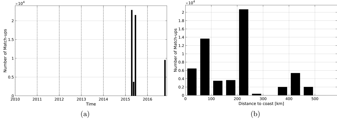
Figure 1: Number of match-ups between TSG-SAMOS and SMAP-L3-RSS-V2-MONTHLY-0.25DEG-40KM SSS as a function of time (a) and as function of the distance to coast (b) over the Indian Ocean Pi-MEP region and for the full satellite product period.
