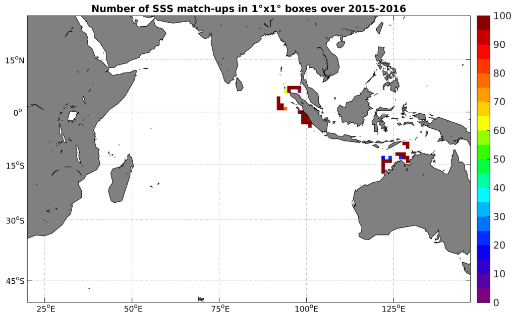
Figure 4: Number of SSS match-ups between TSG-SAMOS SSS and the SMAP-L3-RSS-V2-MONTHLY-0.25DEG-40KM SSS product for the Indian Ocean Pi-MEP region over 1^\circ \times 1^\circ boxes and for the full satellite product period.
