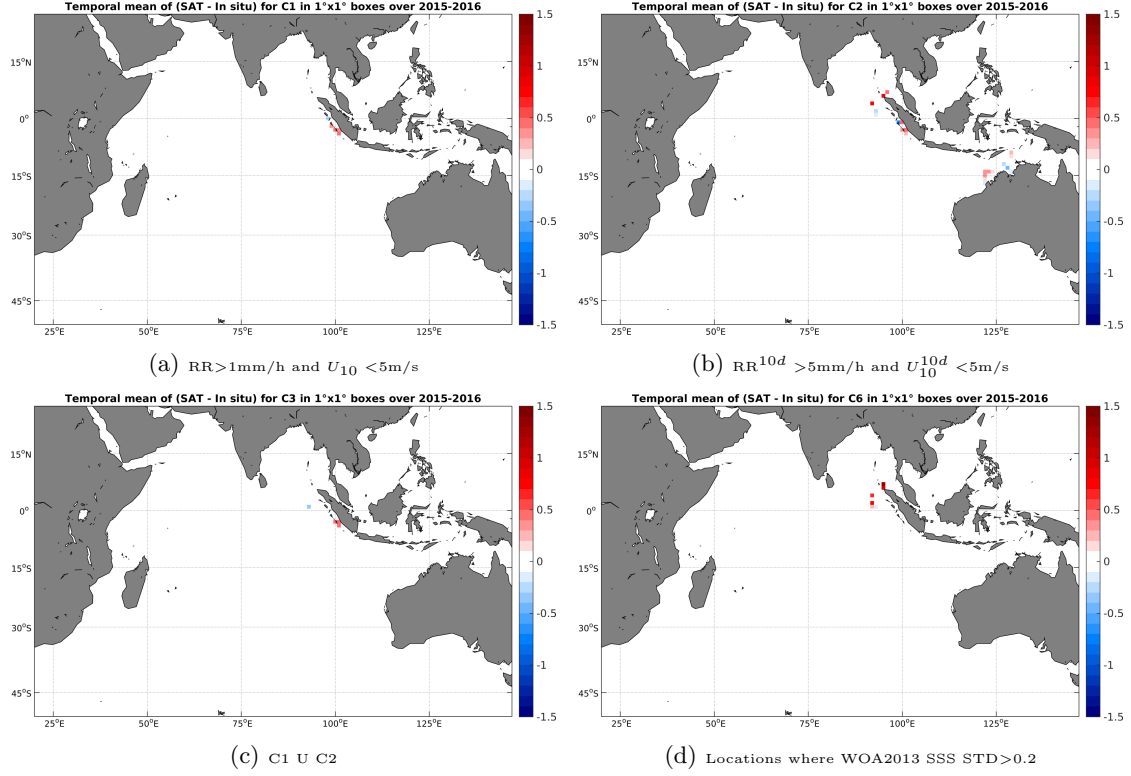
Figure 12: Temporal mean gridded over spatial boxes of size 1^\circ \times 1^\circ of \Delta SSS (SMAP-L3-RSS-V2-MONTHLY-0.25DEG-40KM - TSG-SAMOS) for 4 different subdatasets corresponding to: RR > 1 mm/h and U_{10} < 5 m/s (a), RR^{10d} > 5 mm/h and U_{10}^{10d} < 5 m/s (b), C1 U C2 (c), Locations where WOA2013 SSS STD > 0.2 (d).
