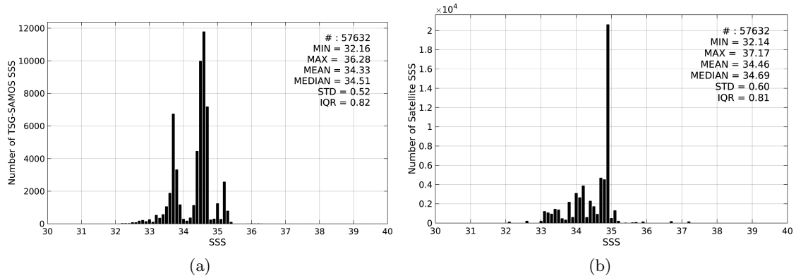
Figure 2: Histograms of SSS from TSG-SAMOS (a) and SMAP-L3-RSS-V2-MONTHLY-0.25DEG-40KM (b) considering all match-up pairs per bins of 0.1 over the Indian Ocean Pi-MEP region and for the full satellite product period.
