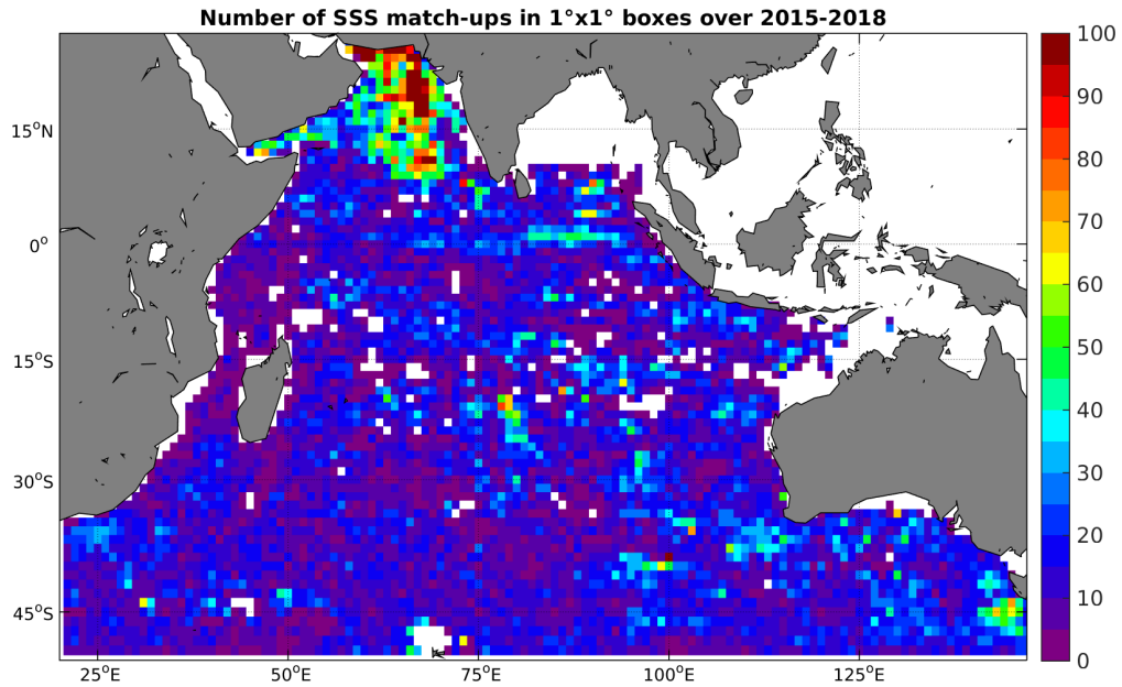
Figure 4: Number of SSS match-ups between Argo SSS and the SMAP-L3-RSS-V2-MONTHLY-0.25DEG-40KM SSS product for the Indian Ocean Pi-MEP region over 1^\circ \times 1^\circ boxes and for the full satellite product period.
