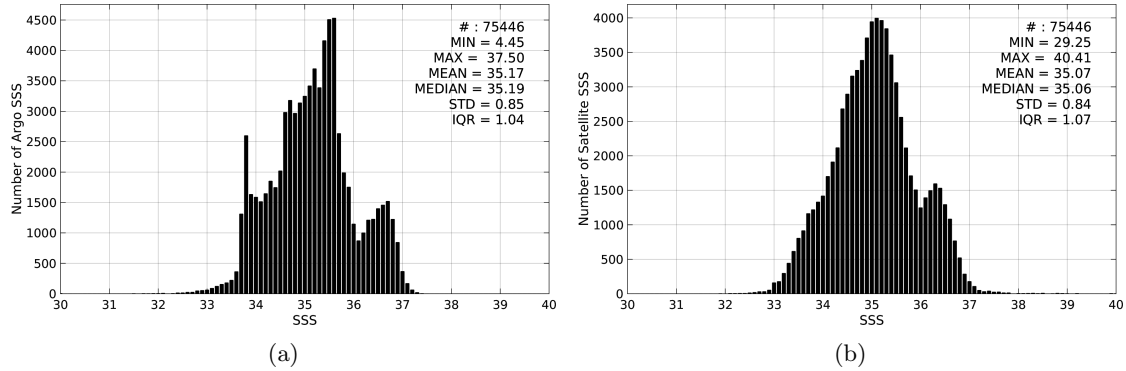
Figure 2: Histograms of SSS from Argo (a) and SMAP-L3-RSS-V2-MONTHLY-0.25DEG-40KM (b) considering all match-up pairs per bins of 0.1 over the Indian Ocean Pi-MEP region and for the full satellite product period.
