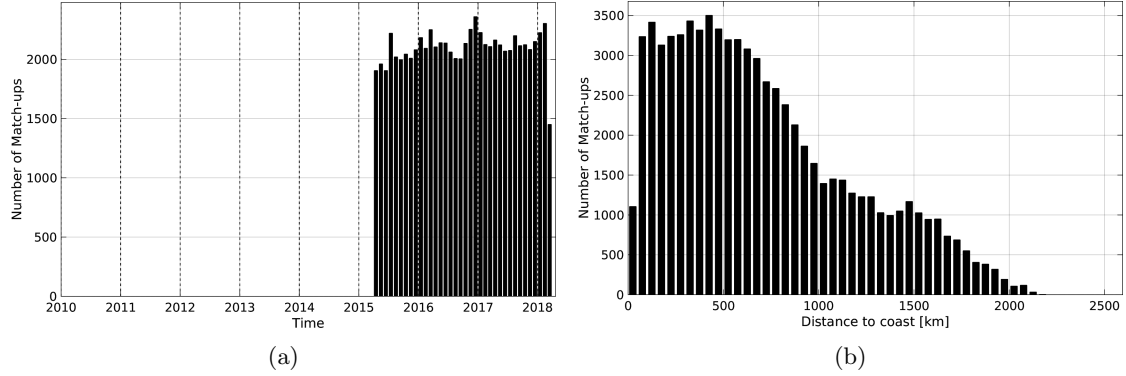
Figure 1: Number of match-ups between Argo and SMAP-L3-RSS-V2-MONTHLY-0.25DEG-40KM SSS as a function of time (a) and as function of the distance to coast (b) over the Indian Ocean Pi-MEP region and for the full satellite product period.
