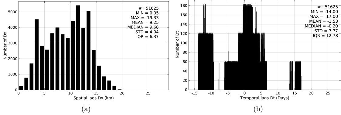
Figure 5: Histograms of the spatial (a) and temporal (b) lags between the time of the TSG-SAMOS measurements and the date of the corresponding SMAP-L3-RSS-V2-MONTHLY-70KM SSS product.
