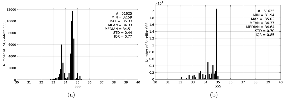
Figure 2: Histograms of SSS from TSG-SAMOS (a) and SMAP-L3-RSS-V2-MONTHLY-70KM (b) considering all match-up pairs per bins of 0.1 over the Indian Ocean Pi-MEP region and for the full satellite product period.
