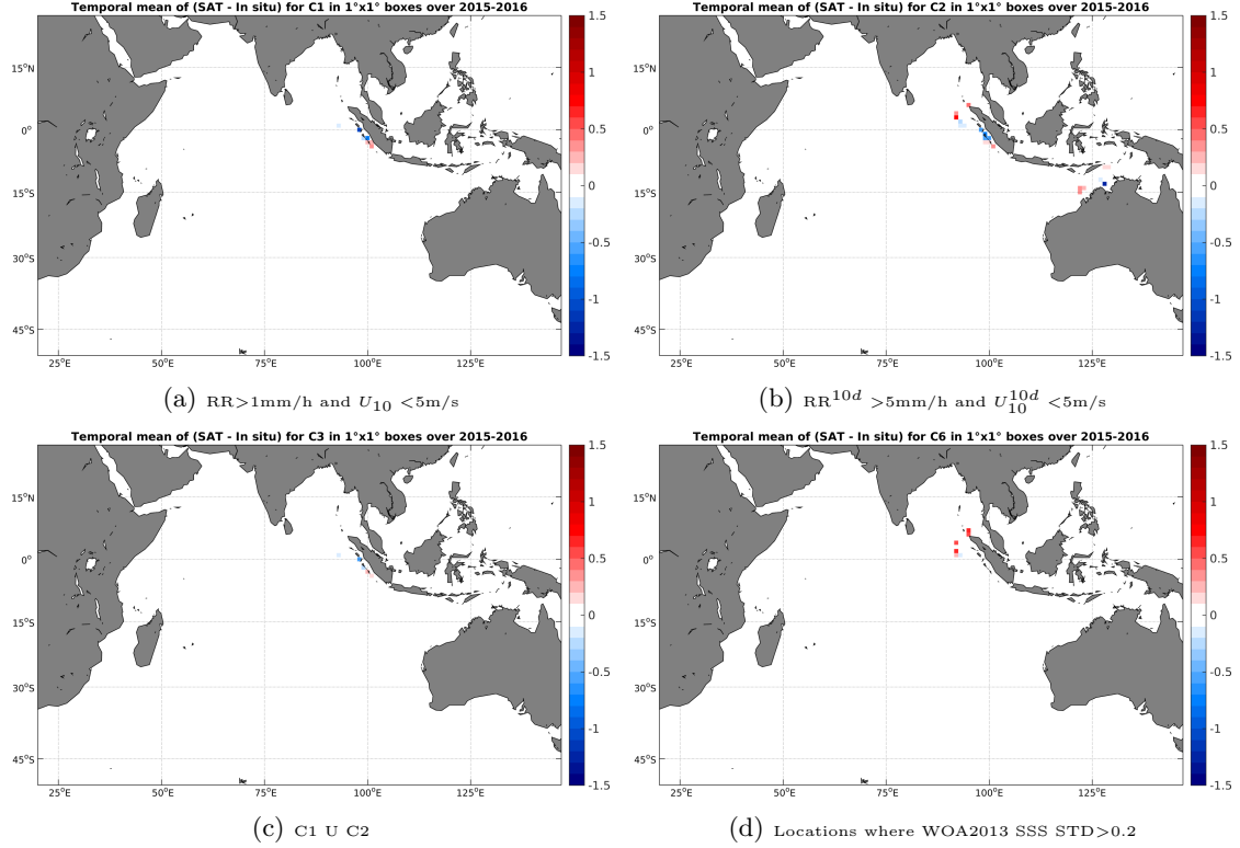
Figure 12: Temporal mean gridded over spatial boxes of size 1^\circ \times 1^\circ of \Delta SSS (SMAP-L3-RSS-V2-MONTHLY-70KM - TSG-SAMOS) for 4 different subdatasets corresponding to: RR > 1 mm/h and U_{10} < 5 m/s (a), RR^{10d} > 5 mm/h and U_{10}^{10d} < 5 m/s (b), C1 U C2 (c), Locations where WOA2013 SSS STD > 0.2 (d).
