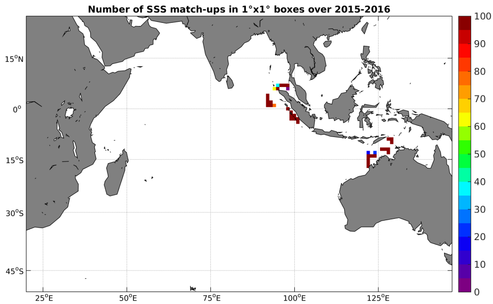
Figure 4: Number of SSS match-ups between TSG-SAMOS SSS and the SMAP-L3-RSS-V2-MONTHLY-70KM SSS product for the Indian Ocean Pi-MEP region over 1°x1° boxes and for the full satellite product period.
