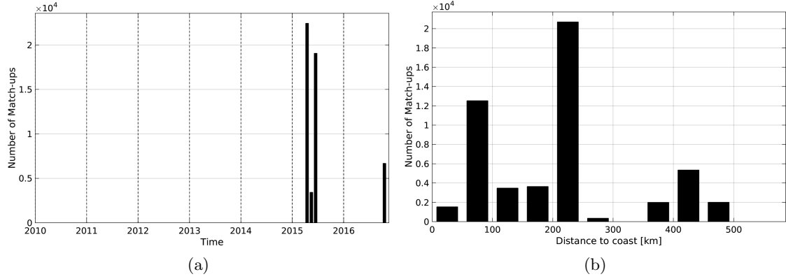
Figure 1: Number of match-ups between TSG-SAMOS and SMAP-L3-RSS-V2-MONTHLY-70KM SSS as a function of time (a) and as function of the distance to coast (b) over the Indian Ocean Pi-MEP region and for the full satellite product period.
