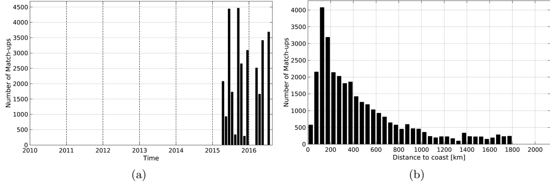
Figure 1: Number of match-ups between TSG-LEGOS-DM and SMAP-L3-RSS-V2-MONTHLY-70KM SSS as a function of time (a) and as function of the distance to coast (b) over the Indian Ocean Pi-MEP region and for the full satellite product period.
