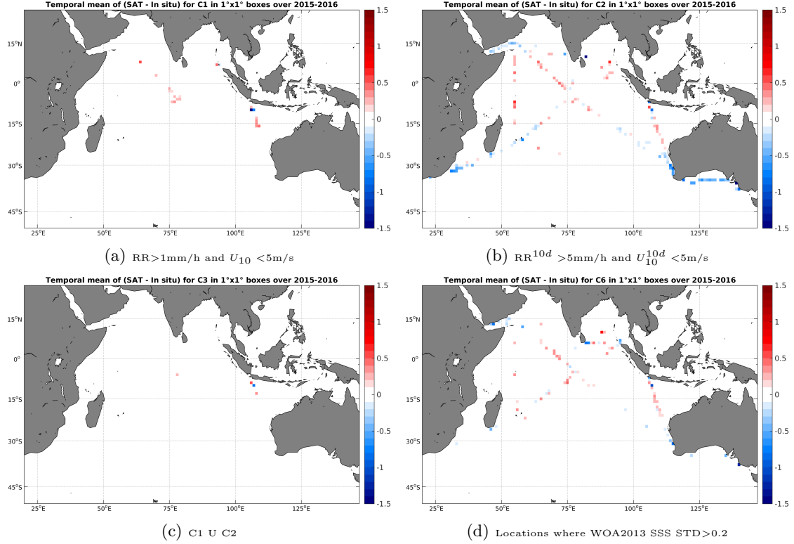
Figure 12: Temporal mean gridded over spatial boxes of size 1^\circ \times 1^\circ of \Delta SSS (SMAP-L3-RSS-V2-MONTHLY-70KM - TSG-LEGOS-DM) for 4 different subdatasets corresponding to: RR > 1\text{mm/h} and U_{10} < 5\text{m/s} (a), RR^{10d} > 5\text{mm/h} and U_{10}^{10d} < 5\text{m/s} (b), C1 U C2 (c), Locations where WOA2013 SSS STD > 0.2 (d).
