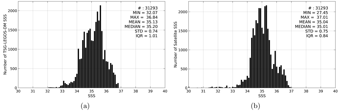
Figure 2: Histograms of SSS from TSG-LEGOS-DM (a) and SMAP-L3-RSS-V2-MONTHLY-70KM (b) considering all match-up pairs per bins of 0.1 over the Indian Ocean Pi-MEP region and for the full satellite product period.
