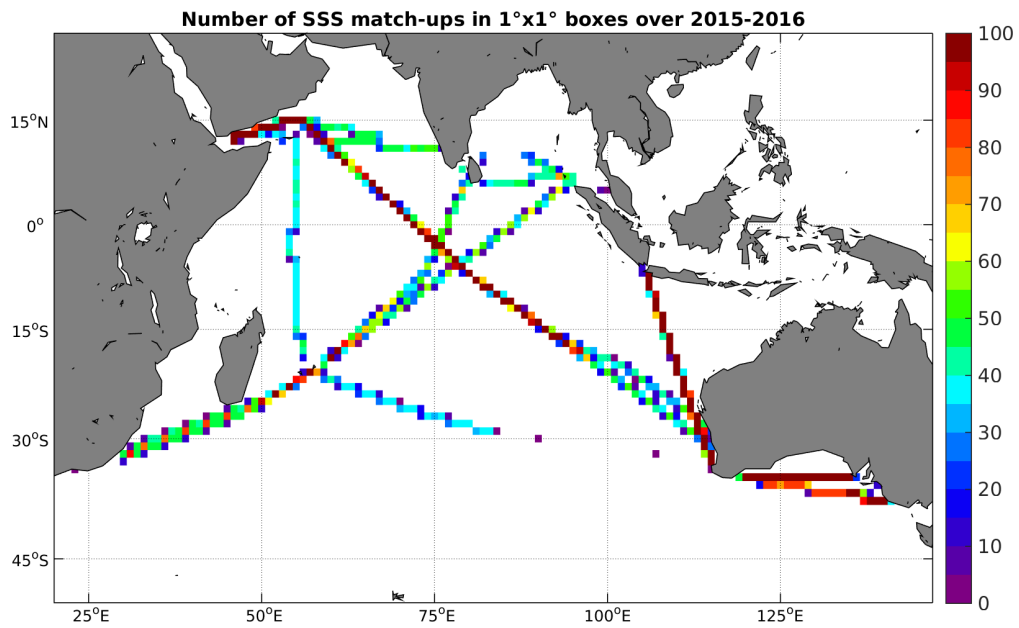
Figure 4: Number of SSS match-ups between TSG-LEGOS-DM SSS and the SMAP-L3-RSS-V2-MONTHLY-70KM SSS product for the Indian Ocean Pi-MEP region over 1°x1° boxes and for the full satellite product period.
