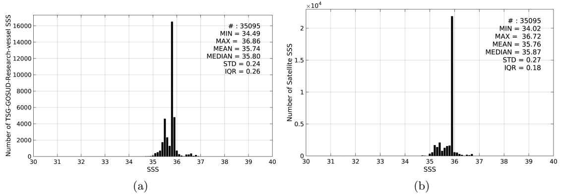
Figure 2: Histograms of SSS from TSG-GOSUD-Research-vessel (a) and SMAP-L3-RSS-V2-MONTHLY-70KM (b) considering all match-up pairs per bins of 0.1 over the Indian Ocean Pi-MEP region and for the full satellite product period.
