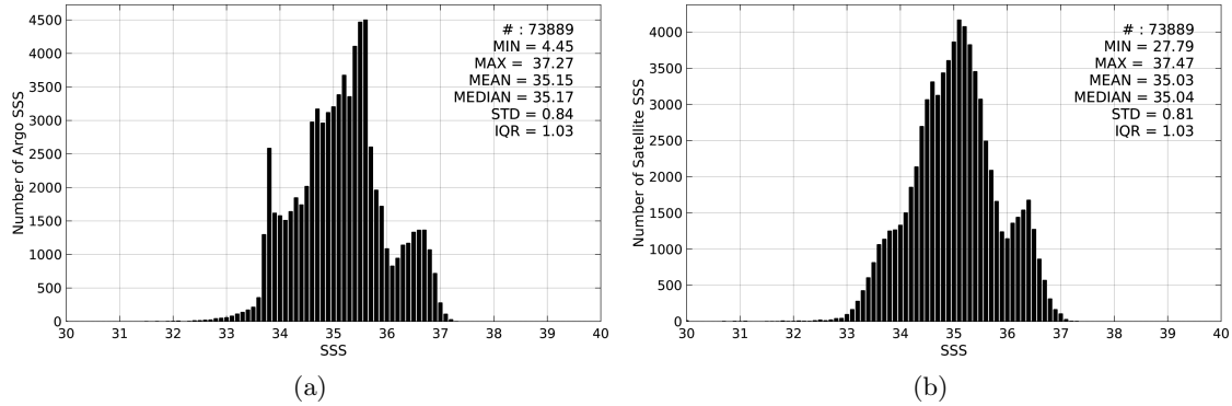
Figure 2: Histograms of SSS from Argo (a) and SMAP-L3-RSS-V2-MONTHLY-70KM (b) considering all match-up pairs per bins of 0.1 over the Indian Ocean Pi-MEP region and for the full satellite product period.
