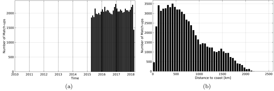
Figure 1: Number of match-ups between Argo and SMAP-L3-RSS-V2-MONTHLY-70KM SSS as a function of time (a) and as function of the distance to coast (b) over the Indian Ocean Pi-MEP region and for the full satellite product period.
