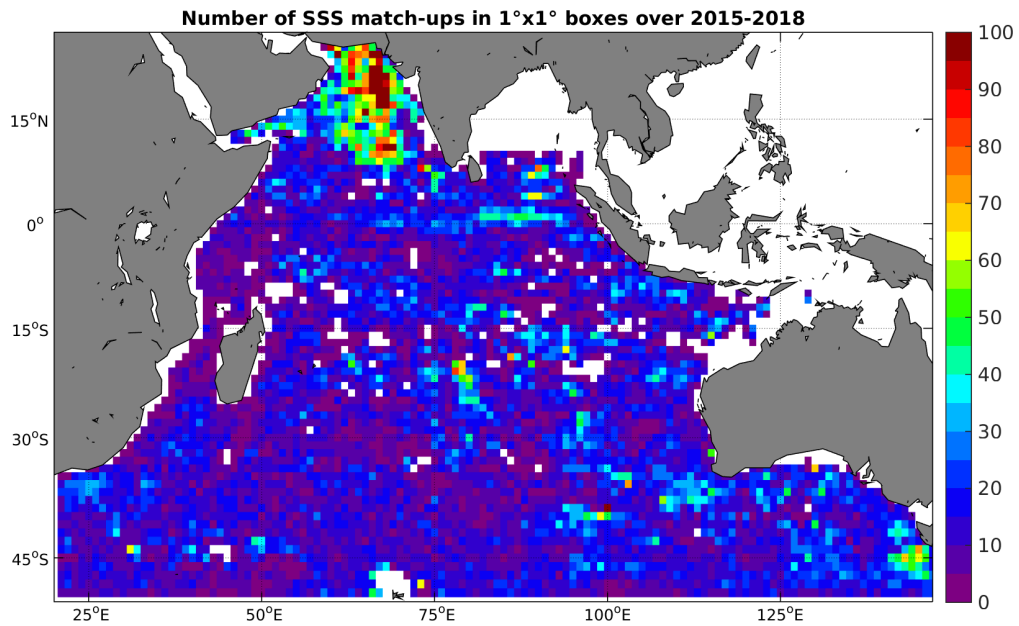
Figure 4: Number of SSS match-ups between Argo SSS and the SMAP-L3-RSS-V2-MONTHLY-70KM SSS product for the Indian Ocean Pi-MEP region over 1^\circ \times 1^\circ boxes and for the full satellite product period.
