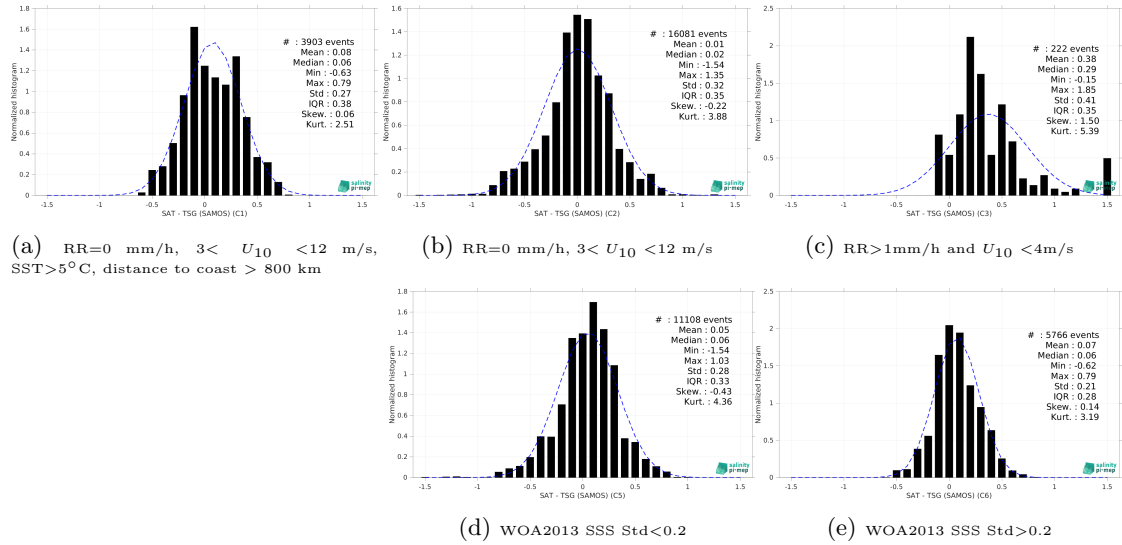
Figure 15: Normalized histogram of \Delta SSS (SMAP SSS L3 v5.0 - 8-Day running (JPL) - TSG (SAMOS)) for 5 different subdatasets corresponding to: RR=0 mm/h, 3 < U_{10} < 12 m/s, SST>5°C, distance to coast > 800 km (a), RR=0 mm/h, 3 < U_{10} < 12 m/s (b), RR>1mm/h and U_{10} < 4 m/s (c), WOA2013 SSS Std<0.2 (d), WOA2013 SSS Std>0.2 (e).
