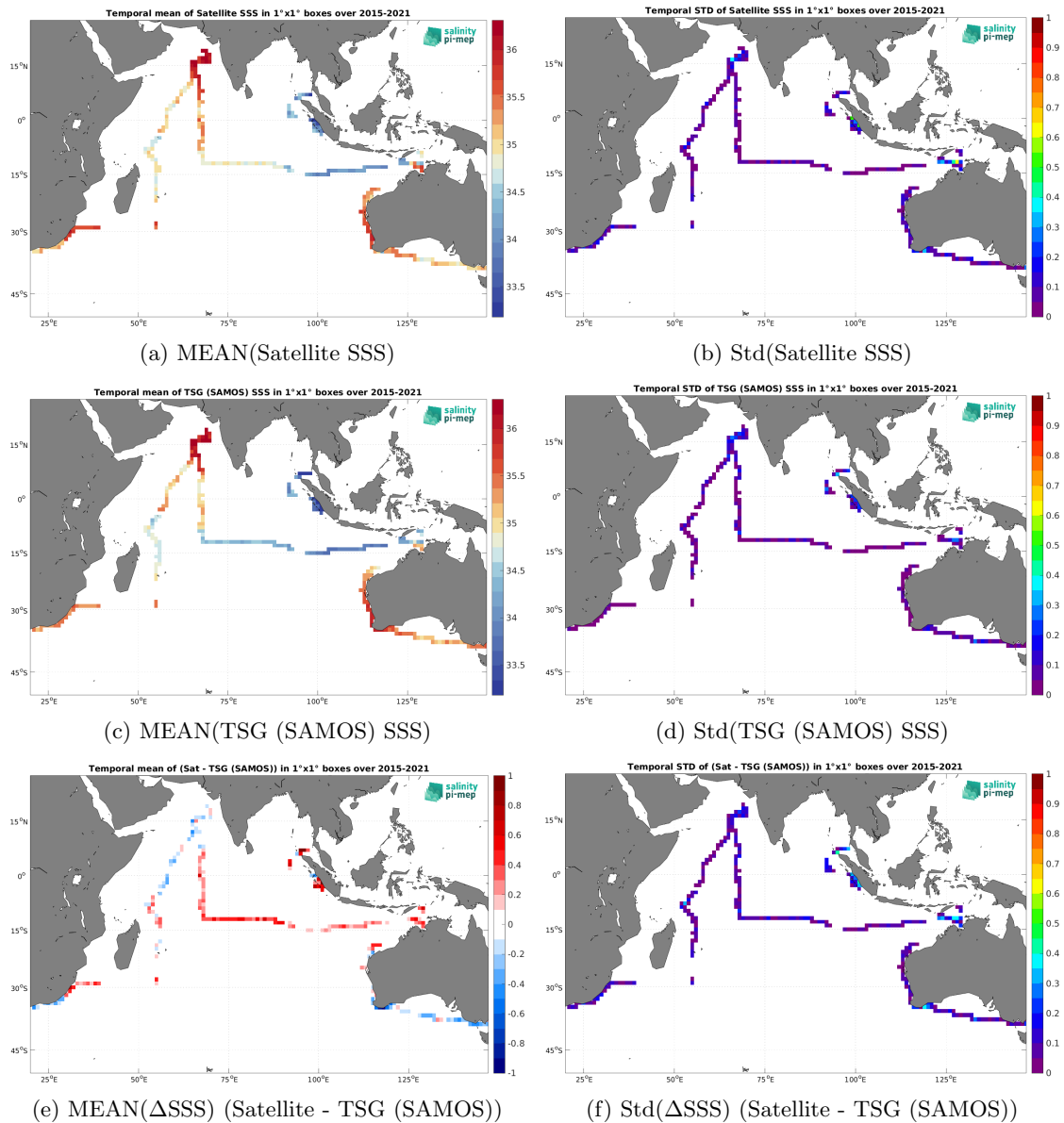
Figure 7: Temporal mean (left) and Std (right) of SSS from SMAP SSS L3 v5.0 - 8-Day running (JPL) (top), TSG (SAMOS) (middle), and of \Delta SSS (Satellite - TSG (SAMOS)). Only match-up pairs are used to generate these maps.
