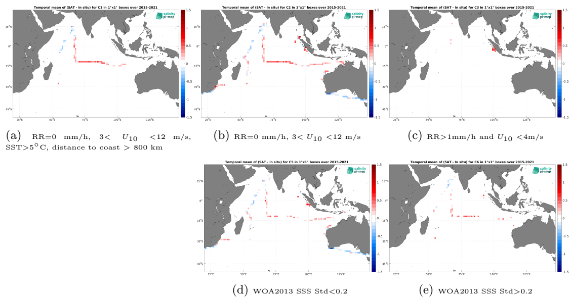
Figure 14: Temporal mean gridded over spatial boxes of size 1^\circ \times 1^\circ of \Delta SSS (SMAP SSS L3 v5.0 - 8-Day running (JPL) - TSG (SAMOS)) for 5 different subdatasets corresponding to:RR=0 mm/h, 3 < U_{10} < 12 m/s, SST >5^\circ\text{C} , distance to coast > 800 km (a), RR=0 mm/h, 3 < U_{10} < 12 m/s (b), RR >1 mm/h and U_{10} < 4 m/s (c), WOA2013 SSS Std <0.2 (d), WOA2013 SSS Std >0.2 (e).
