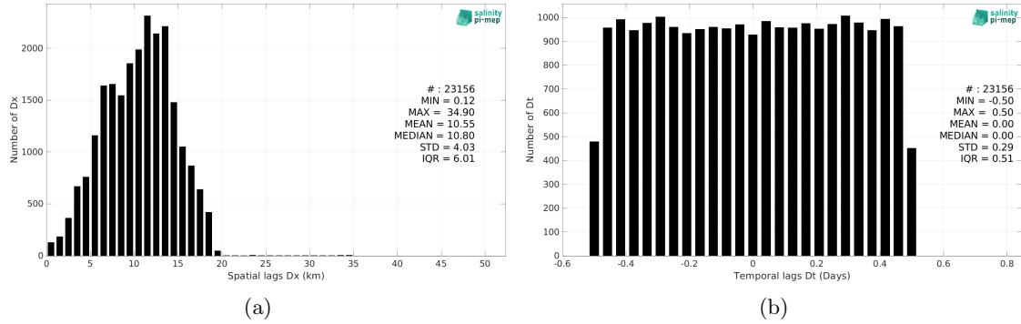
Figure 6: Histograms of the spatial (a) and temporal (b) lags between the location/time of the TSG (SAMOS) measurement and the date of the corresponding SMAP SSS L3 v5.0 - 8-Day running (JPL) SSS pixel.
