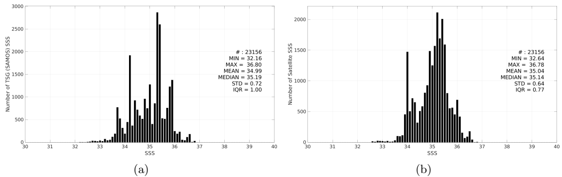
Figure 3: Histograms of SSS from TSG (SAMOS) (a) and SMAP SSS L3 v5.0 - 8-Day running (JPL) (b) considering all match-up pairs per bins of 0.1 over the Indian Ocean Pi-MEP region and for the full satellite product period.
