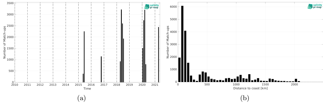
Figure 2: Number of match-ups between TSG (SAMOS) and SMAP SSS L3 v5.0 - 8-Day running (JPL) SSS as a function of time (a) and as function of the distance to coast (b) over the Indian Ocean Pi-MEP region and for the full satellite product period.
