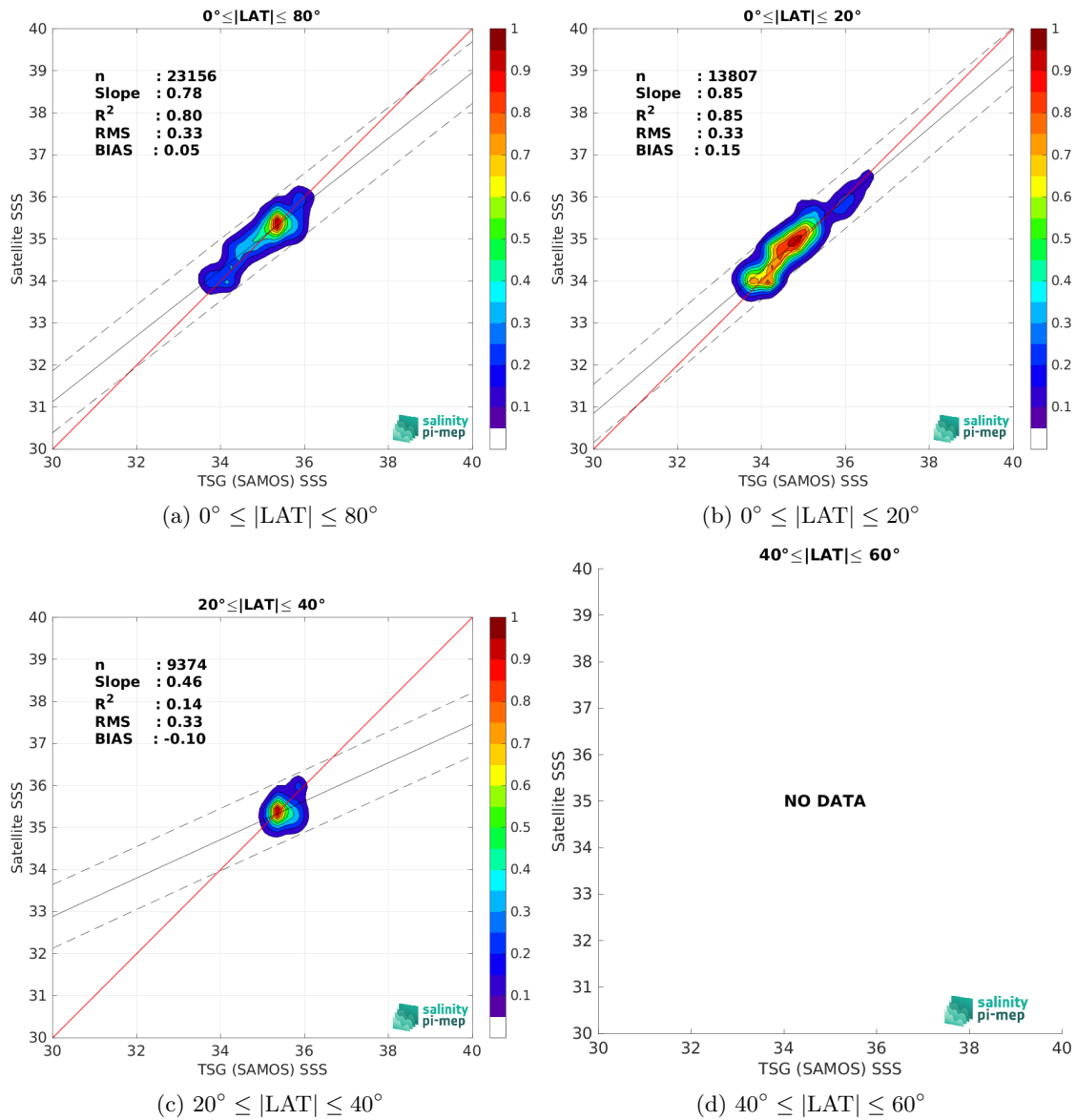
Figure 10: Contour maps of the concentration of SMAP SSS L3 v5.0 - 8-Day running (JPL) SSS (y-axis) versus TSG (SAMOS) SSS (x-axis) at match-up pairs for different latitude bands. For each plot, the red line shows x=y . The black thin and dashed lines indicate a linear fit through the data cloud and the \pm 95\% confidence levels, respectively. The number match-up pairs n , the slope and R^2 coefficient of the linear fit, the root mean square (RMS) and the mean bias between satellite and in situ data are indicated for each latitude band in each plots.
