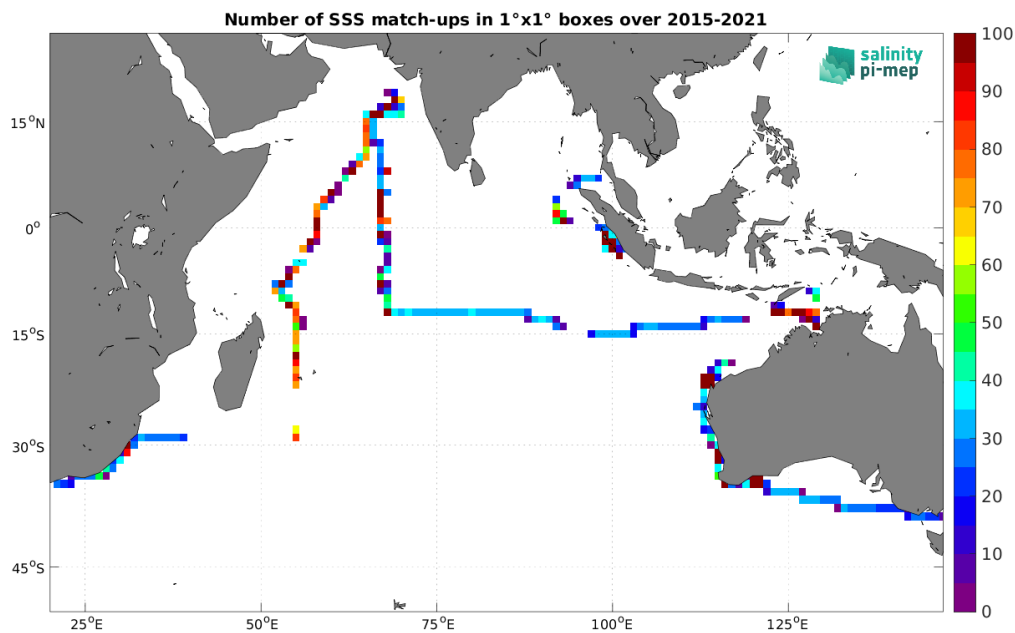
Figure 5: Number of SSS match-ups between TSG (SAMOS) SSS and the SMAP SSS L3 v5.0 - 8-Day running (JPL) SSS product for the Indian Ocean Pi-MEP region over 1^\circ \times 1^\circ boxes and for the full satellite product period.
