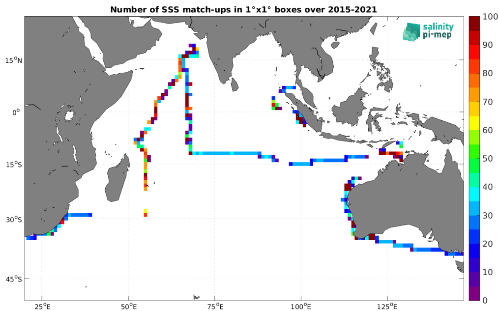
Figure 4: Number of SSS match-ups between TSG (SAMOS) SSS and the SMAP SSS L3 v5.0 - 8-Day running (JPL) SSS product for the Indian Ocean Pi-MEP region over 1^\circ \times 1^\circ boxes and for the full satellite product period.
