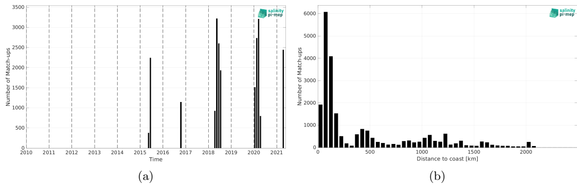
Figure 1: Number of match-ups between TSG (SAMOS) and SMAP SSS L3 v5.0 - 8-Day running (JPL) SSS as a function of time (a) and as function of the distance to coast (b) over the Indian Ocean Pi-MEP region and for the full satellite product period.
