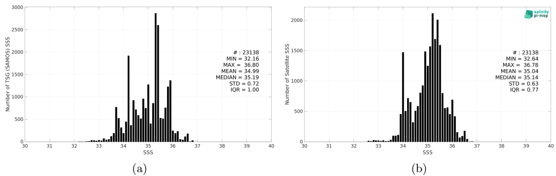
Figure 2: Histograms of SSS from TSG (SAMOS) (a) and SMAP SSS L3 v5.0 - 8-Day running (JPL) (b) considering all match-up pairs per bins of 0.1 over the Indian Ocean Pi-MEP region and for the full satellite product period.
