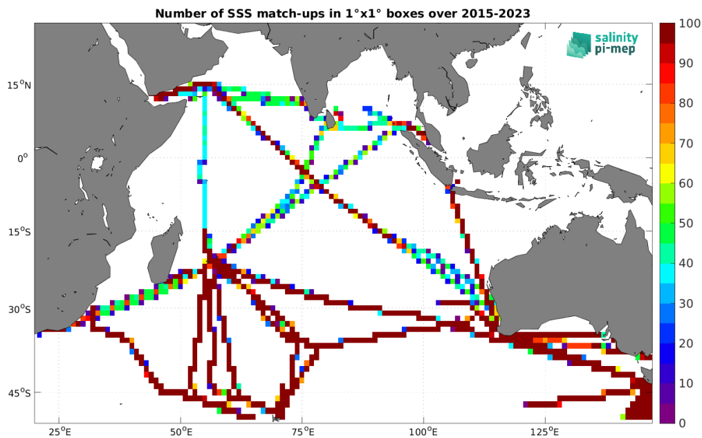
Figure 4: Number of SSS match-ups between TSG (LEGOS-DM) SSS and the SMAP SSS L3 v5.0 - 8-Day running (JPL) SSS product for the Indian Ocean Pi-MEP region over 1^\circ \times 1^\circ boxes and for the full satellite product period.
