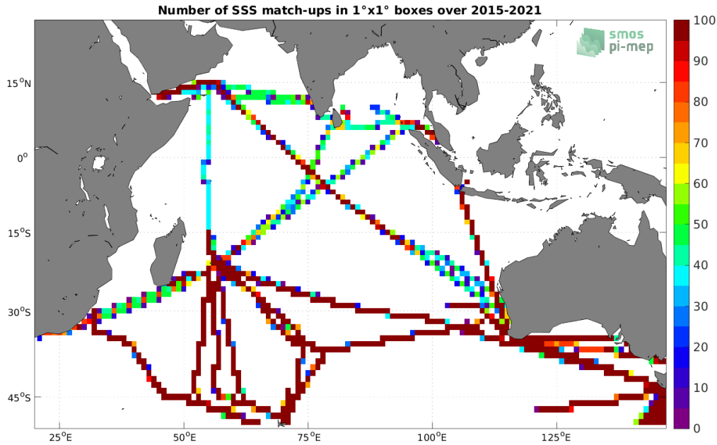
Figure 4: Number of SSS match-ups between TSG (LEGOS-DM) SSS and the SMAP SSS L3 v5.0 - 8-Day running (JPL) SSS product for the Indian Ocean Pi-MEP region over 1^\circ \times 1^\circ boxes and for the full satellite product period.
