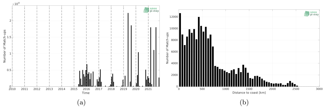
Figure 1: Number of match-ups between TSG (LEGOS-DM) and SMAP SSS L3 v5.0 - 8-Day running (JPL) SSS as a function of time (a) and as function of the distance to coast (b) over the Indian Ocean Pi-MEP region and for the full satellite product period.
