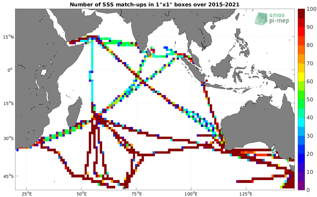
Figure 4: Number of SSS match-ups between TSG (LEGOS-DM) SSS and the SMAP SSS L3 v5.0 - 8-Day running (JPL) SSS product for the Indian Ocean Pi-MEP region over 1^{\circ} \times 1^{\circ} boxes and for the full satellite product period.
