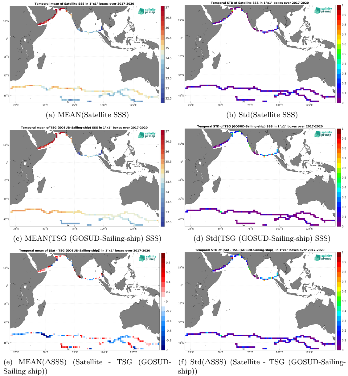
Figure 7: Temporal mean (left) and Std (right) of SSS from SMAP SSS L3 v5.0 - 8-Day running (JPL) (top), TSG (GOSUD-Sailing-ship) (middle), and of \Delta SSS (Satellite - TSG (GOSUD-Sailing-ship)). Only match-up pairs are used to generate these maps.
