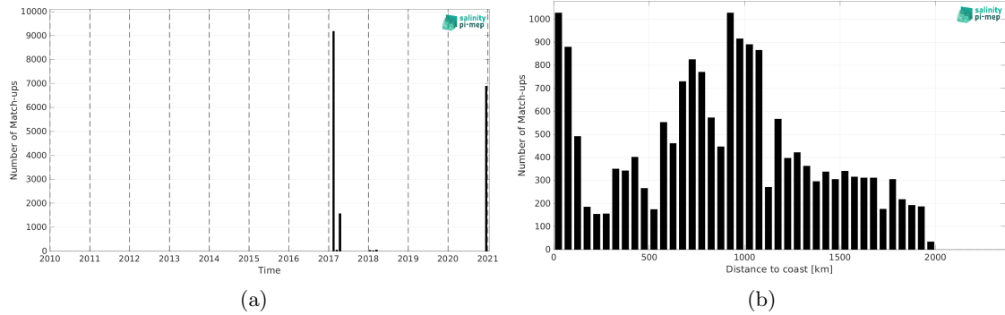
Figure 2: Number of match-ups between TSG (GOSUD-Sailing-ship) and SMAP SSS L3 v5.0 - 8-Day running (JPL) SSS as a function of time (a) and as function of the distance to coast (b) over the Indian Ocean Pi-MEP region and for the full satellite product period.
