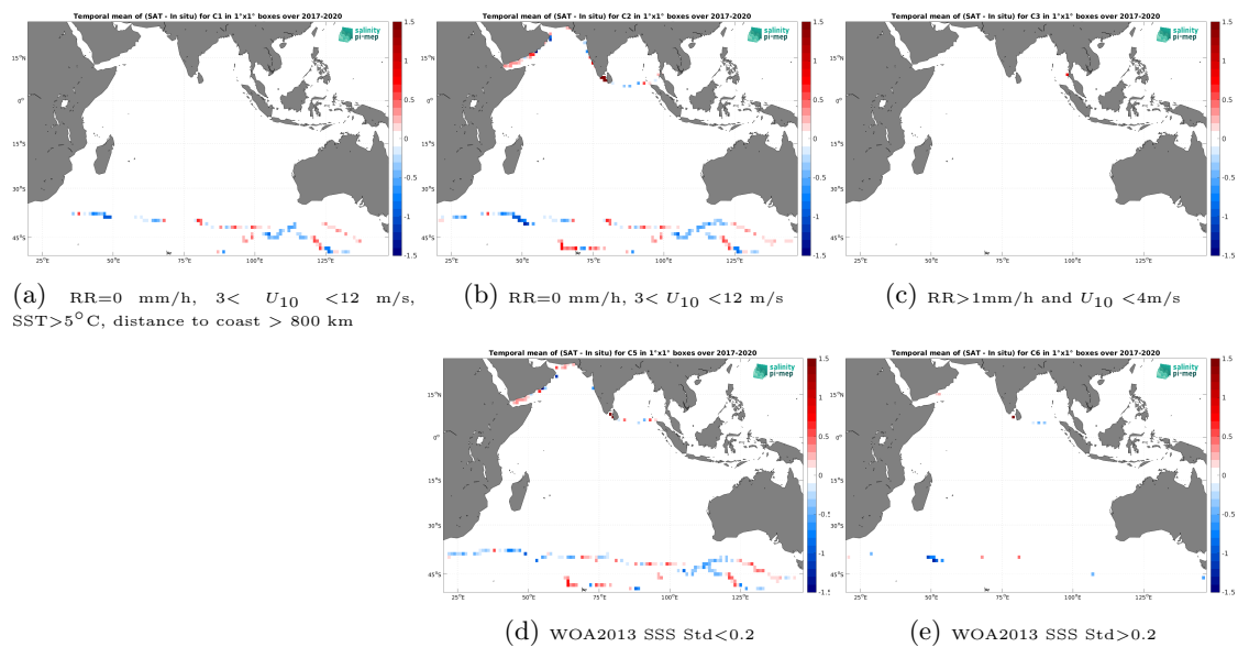
Figure 14: Temporal mean gridded over spatial boxes of size 1^\circ \times 1^\circ of \Delta SSS (SMAP SSS L3 v5.0 - 8-Day running (JPL) - TSG (GOSUD-Sailing-ship)) for 5 different subdatasets corresponding to:RR=0 mm/h, 3 < U_{10} < 12 m/s, SST > 5^\circ\text{C} , distance to coast > 800 km (a), RR=0 mm/h, 3 < U_{10} < 12 m/s (b), RR > 1 mm/h and U_{10} < 4 m/s (c), WOA2013 SSS Std < 0.2 (d), WOA2013 SSS Std > 0.2 (e).
