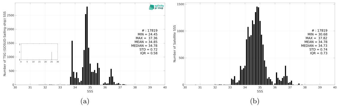
Figure 3: Histograms of SSS from TSG (GOSUD-Sailing-ship) (a) and SMAP SSS L3 v5.0 - 8-Day running (JPL) (b) considering all match-up pairs per bins of 0.1 over the Indian Ocean Pi-MEP region and for the full satellite product period.
