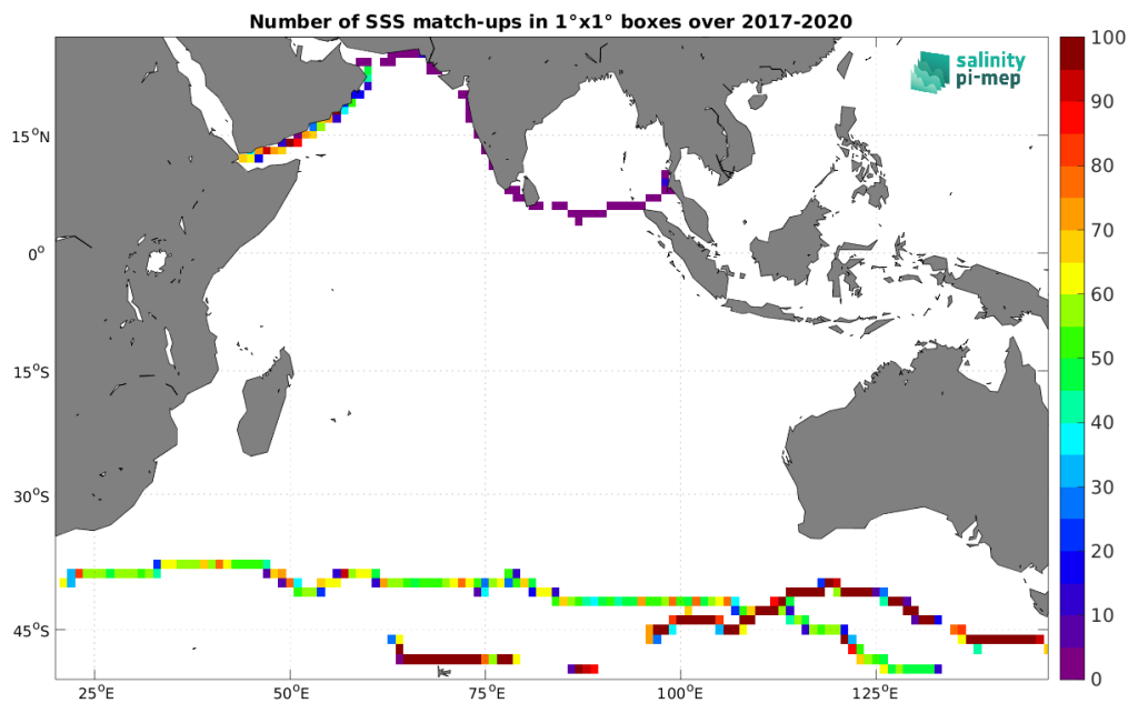
Figure 5: Number of SSS match-ups between TSG (GOSUD-Sailing-ship) SSS and the SMAP SSS L3 v5.0 - 8-Day running (JPL) SSS product for the Indian Ocean Pi-MEP region over 1^\circ \times 1^\circ boxes and for the full satellite product period.
