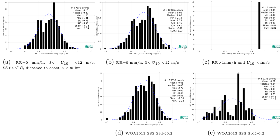
Figure 15: Normalized histogram of \Delta\text{SSS} (SMAP SSS L3 v5.0 - 8-Day running (JPL) - TSG (GOSUD-Sailing-ship)) for 5 different subdatasets corresponding to: RR=0 mm/h, 3 < U_{10} < 12 m/s, SST > 5^{\circ}\text{C} , distance to coast > 800 km (a), RR=0 mm/h, 3 < U_{10} < 12 m/s (b), RR > 1\text{mm/h} and U_{10} < 4\text{m/s} (c), WOA2013 SSS Std < 0.2 (d), WOA2013 SSS Std > 0.2 (e).
