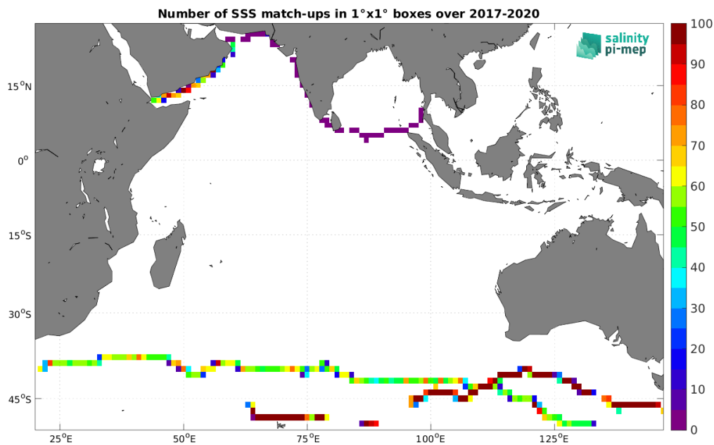
Figure 4: Number of SSS match-ups between TSG (GOSUD-Sailing-ship) SSS and the SMAP SSS L3 v5.0 - 8-Day running (JPL) SSS product for the Indian Ocean Pi-MEP region over 1^\circ \times 1^\circ boxes and for the full satellite product period.
