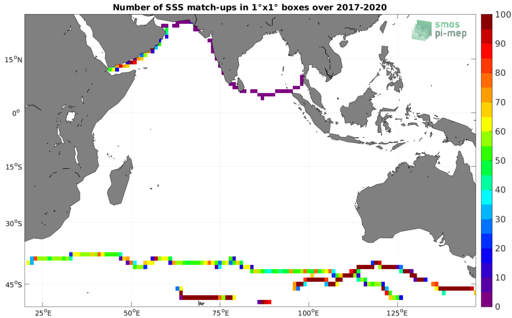
Figure 4: Number of SSS match-ups between TSG (GOSUD-Sailing-ship) SSS and the SMAP SSS L3 v5.0 - 8-Day running (JPL) SSS product for the Indian Ocean Pi-MEP region over 1^\circ \times 1^\circ boxes and for the full satellite product period.
