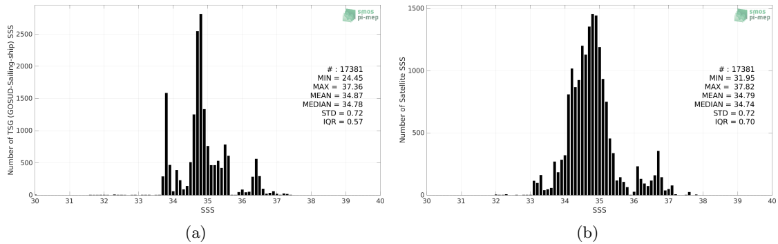
Figure 2: Histograms of SSS from TSG (GOSUD-Sailing-ship) (a) and SMAP SSS L3 v5.0 - 8-Day running (JPL) (b) considering all match-up pairs per bins of 0.1 over the Indian Ocean Pi-MEP region and for the full satellite product period.
