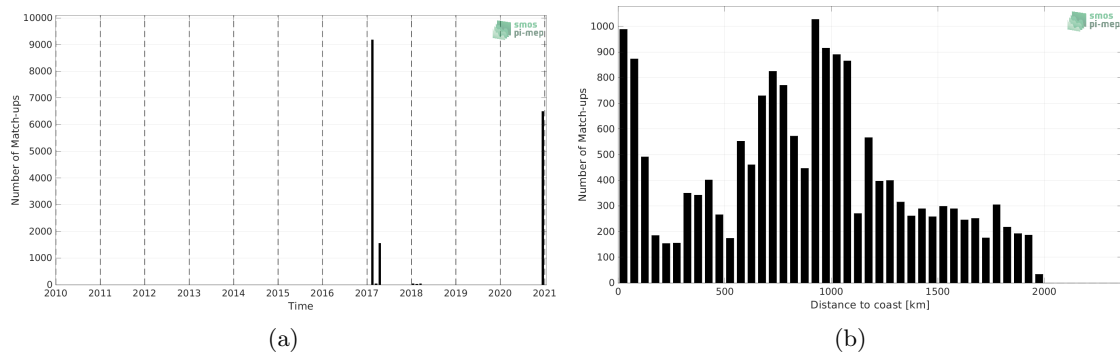
Figure 1: Number of match-ups between TSG (GOSUD-Sailing-ship) and SMAP SSS L3 v5.0 - 8-Day running (JPL) SSS as a function of time (a) and as function of the distance to coast (b) over the Indian Ocean Pi-MEP region and for the full satellite product period.
