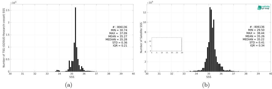
Figure 3: Histograms of SSS from TSG (GOSUD-Research-vessel) (a) and SMAP SSS L3 v5.0 - 8-Day running (JPL) (b) considering all match-up pairs per bins of 0.1 over the Indian Ocean Pi-MEP region and for the full satellite product period.
