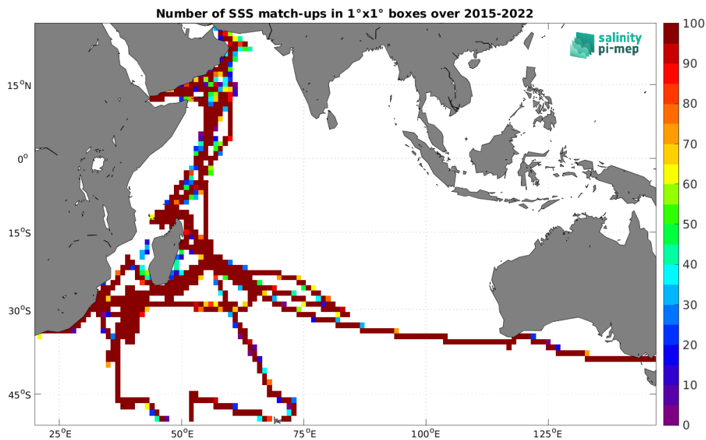
Figure 5: Number of SSS match-ups between TSG (GOSUD-Research-vessel) SSS and the SMAP SSS L3 v5.0 - 8-Day running (JPL) SSS product for the Indian Ocean Pi-MEP region over 1^\circ \times 1^\circ boxes and for the full satellite product period.
