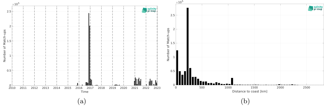
Figure 2: Number of match-ups between TSG (GOSUD-Research-vessel) and SMAP SSS L3 v5.0 - 8-Day running (JPL) SSS as a function of time (a) and as function of the distance to coast (b) over the Indian Ocean Pi-MEP region and for the full satellite product period.
