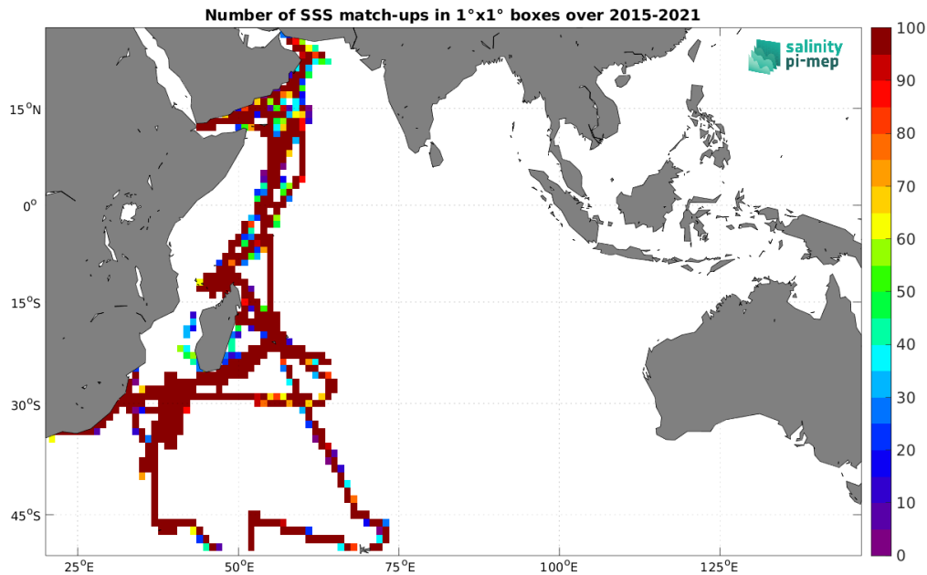
Figure 4: Number of SSS match-ups between TSG (GOSUD-Research-vessel) SSS and the SMAP SSS L3 v5.0 - 8-Day running (JPL) SSS product for the Indian Ocean Pi-MEP region over 1^\circ \times 1^\circ boxes and for the full satellite product period.
