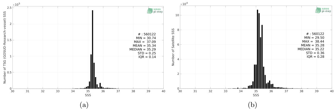
Figure 2: Histograms of SSS from TSG (GOSUD-Research-vessel) (a) and SMAP SSS L3 v5.0 - 8-Day running (JPL) (b) considering all match-up pairs per bins of 0.1 over the Indian Ocean Pi-MEP region and for the full satellite product period.
