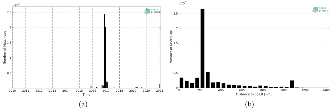
Figure 1: Number of match-ups between TSG (GOSUD-Research-vessel) and SMAP SSS L3 v5.0 - 8-Day running (JPL) SSS as a function of time (a) and as function of the distance to coast (b) over the Indian Ocean Pi-MEP region and for the full satellite product period.
