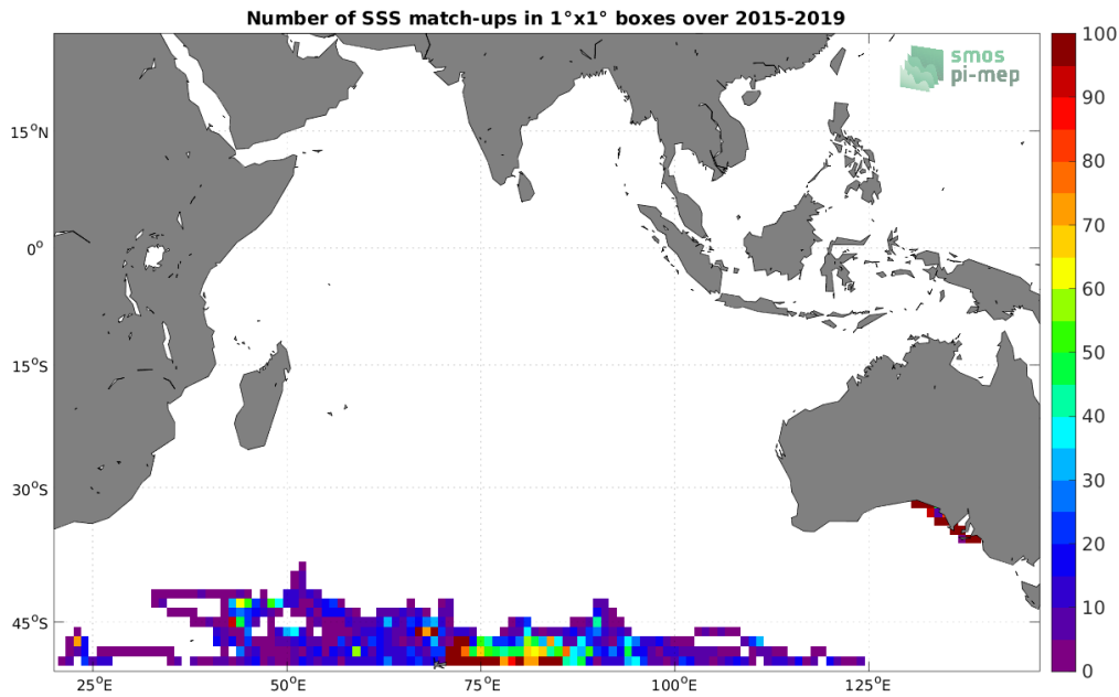
Figure 4: Number of SSS match-ups between Marine mammals SSS and the SMAP SSS L3 v5.0 - 8-Day running (JPL) SSS product for the Indian Ocean Pi-MEP region over 1^\circ \times 1^\circ boxes and for the full satellite product period.
