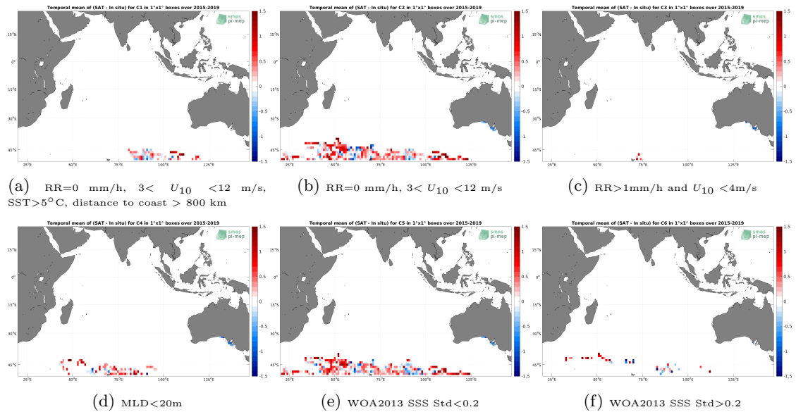
Figure 12: Temporal mean gridded over spatial boxes of size 1^\circ \times 1^\circ of \Delta SSS (SMAP SSS L3 v5.0 - 8-Day running (JPL) - Marine mammals) for 6 different subdatasets corresponding to:RR=0 mm/h, 3 < U_{10} < 12 m/s, SST >5^\circ C, distance to coast > 800 km (a), RR=0 mm/h, 3 < U_{10} < 12 m/s (b), RR >1 mm/h and U_{10} < 4 m/s (c),MLD <20 m (d),WOA2013 SSS Std <0.2 (e),WOA2013 SSS Std >0.2 (f).
