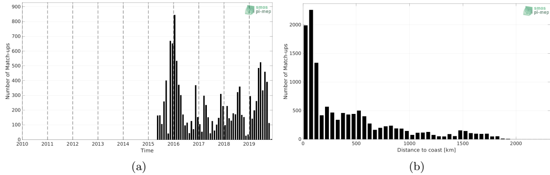
Figure 1: Number of match-ups between Marine mammals and SMAP SSS L3 v5.0 - 8-Day running (JPL) SSS as a function of time (a) and as function of the distance to coast (b) over the Indian Ocean Pi-MEP region and for the full satellite product period.
