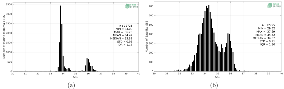
Figure 2: Histograms of SSS from Marine mammals (a) and SMAP SSS L3 v5.0 - 8-Day running (JPL) (b) considering all match-up pairs per bins of 0.1 over the Indian Ocean Pi-MEP region and for the full satellite product period.
